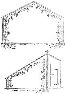
FIG. 2.—LEAN-TO GRAPERY.
