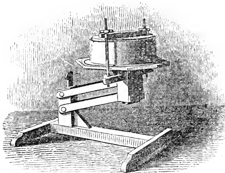
PATENT SELF-ACTING CHEESE PRESS.
