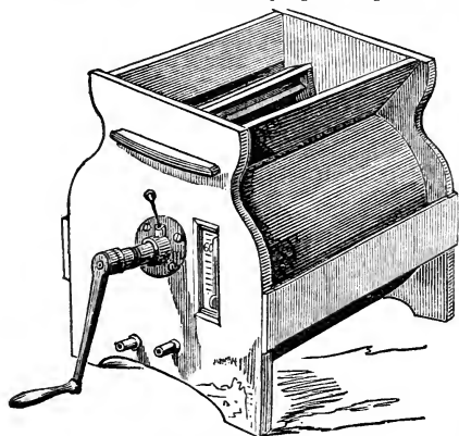
THERMOMETER CHURN.
