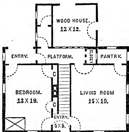
Fig. 3.— First Floor.
