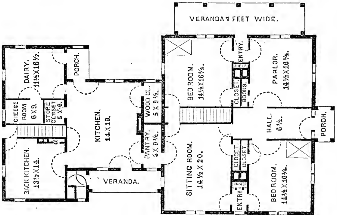
Fig. 15.— First Floor.
