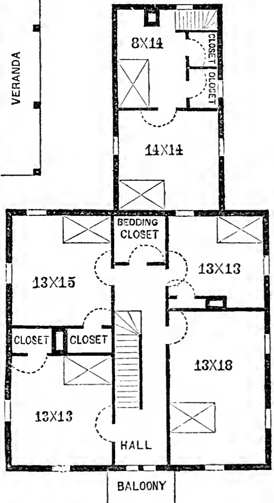
Fig. 21.—Chamber Floor.
