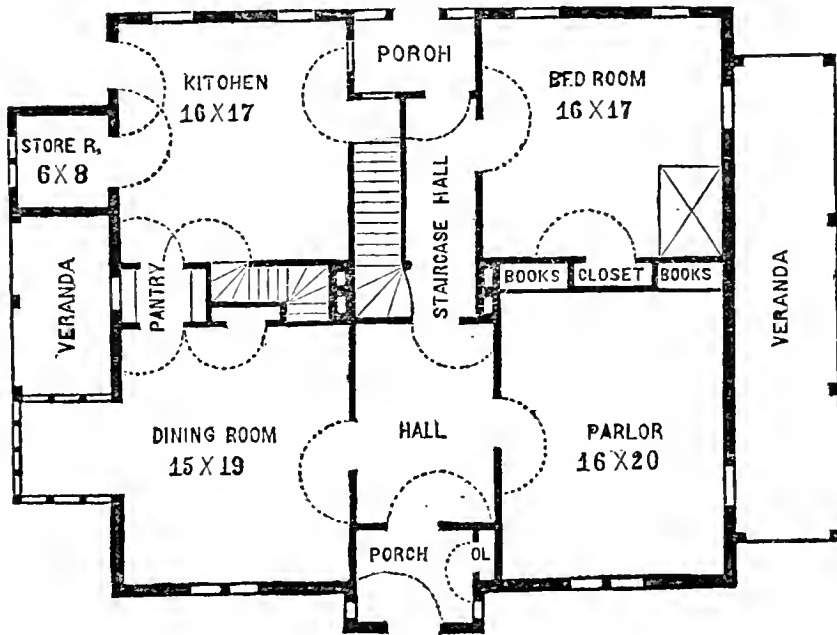
Fig. 17.—First Floor.
