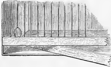
FIG. 5.—TURN-RAIL.
