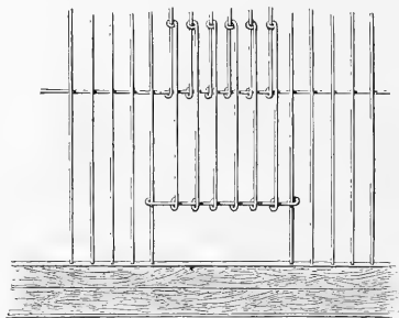
FIG. 10.—SLIDING DOOR.
