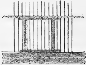
FIG. 7.—WOODEN DOOR.
