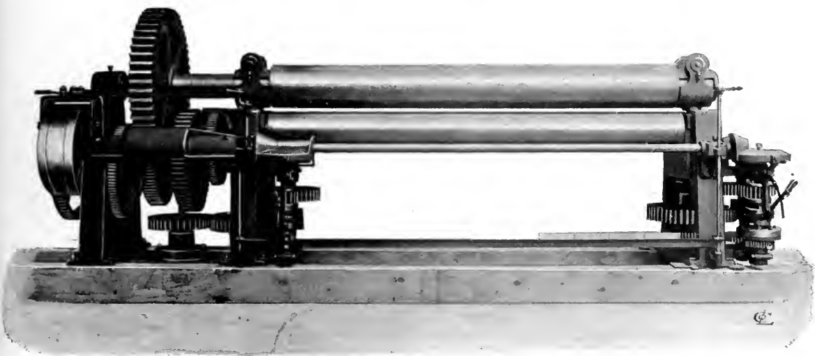
16" PATENT PLATE BENDING MACHINE.
