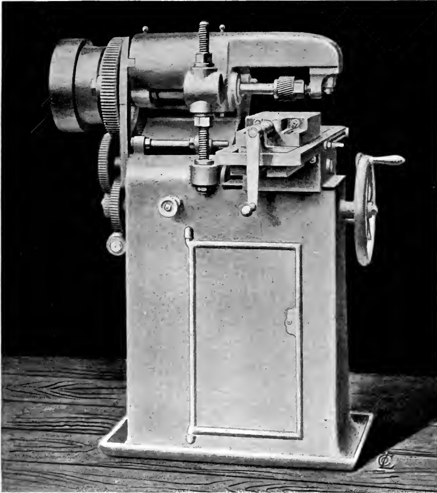
MILLING MACHINE.
