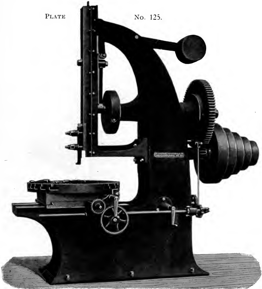
48" SLOTTING MACHINE.
