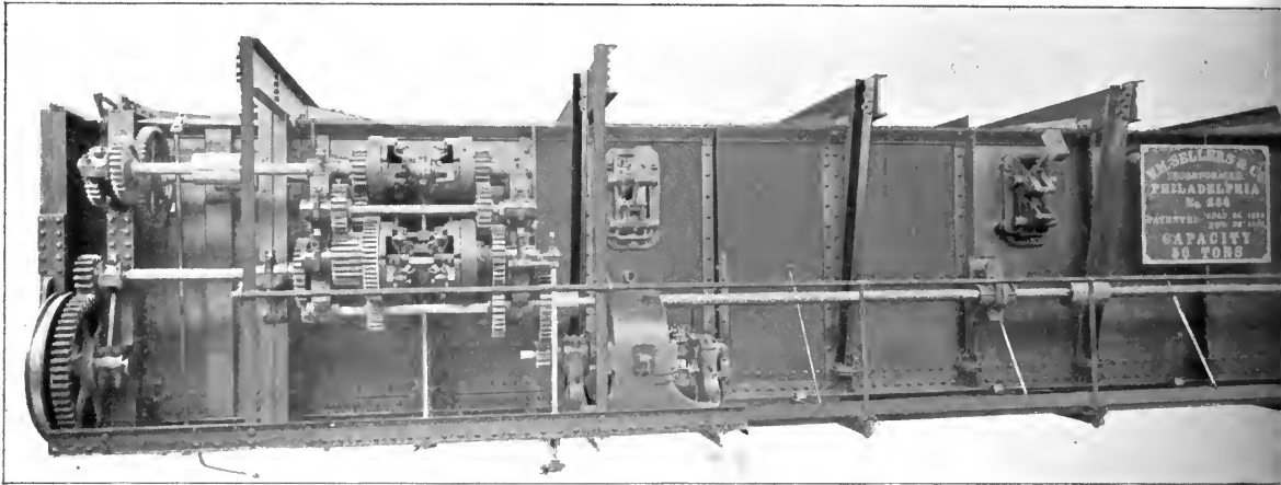
50-TON TRAVELLING CRANE.—SINGLE MOTOR TYPE.
