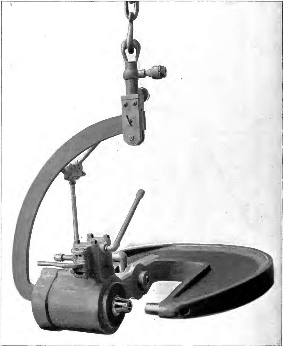
DIRECT-ACTING PORTABLE HYDRAULIC RIVETER. WITH SWIVEL HANGING BAIL.
