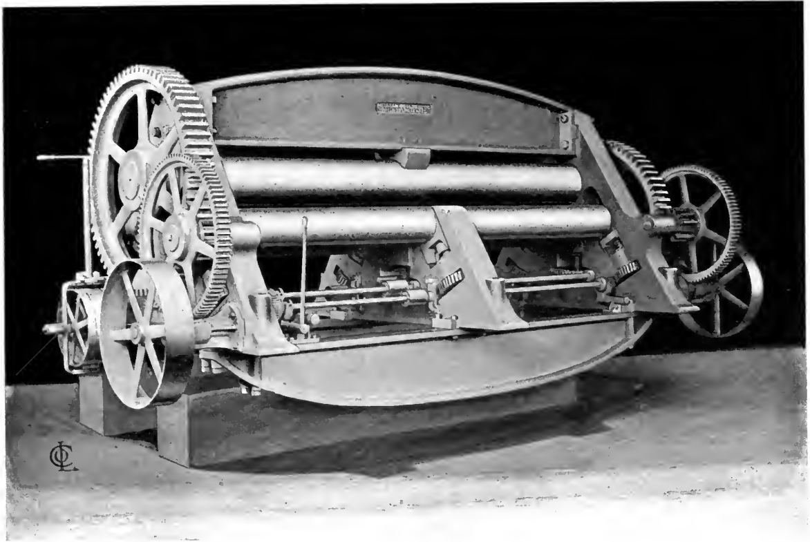
16" SHIP-PLATE ROLLS.—14 FEET BETWEEN HOUSINGS.
