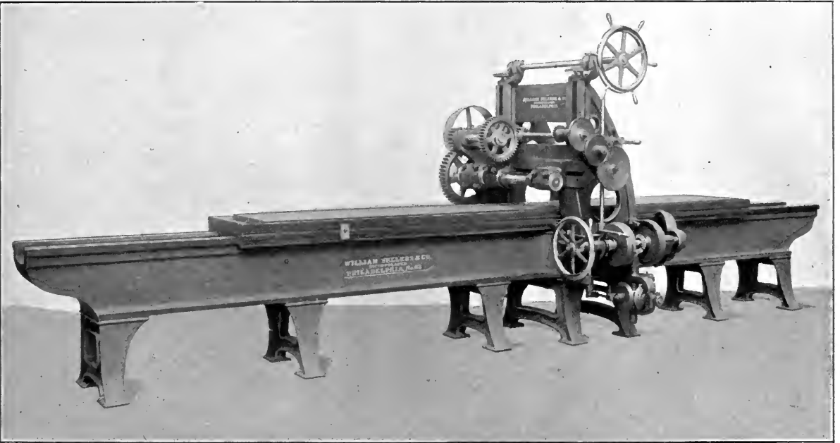
25" SLABBING MACHINE—12 FT. TABLE.
