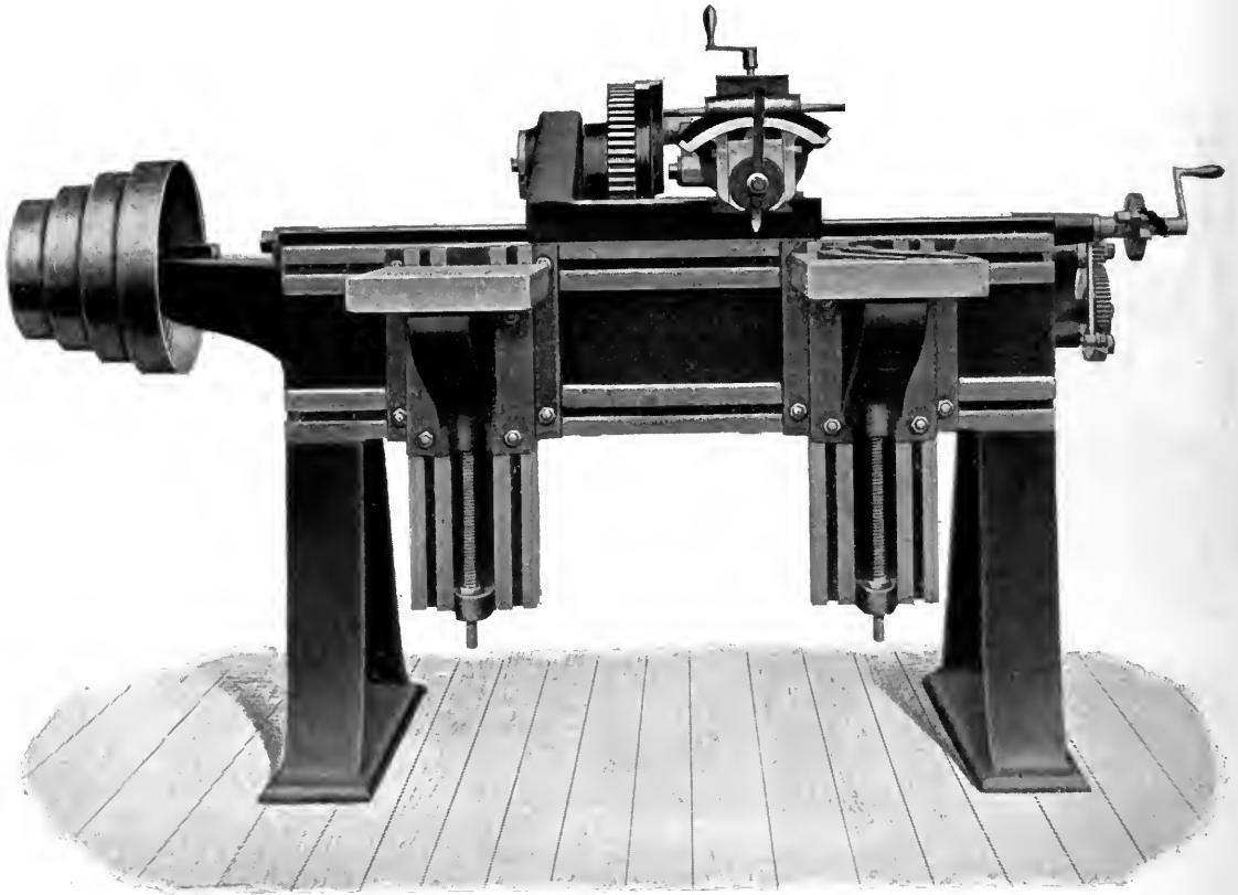
12" SHAPING MACHINE.
