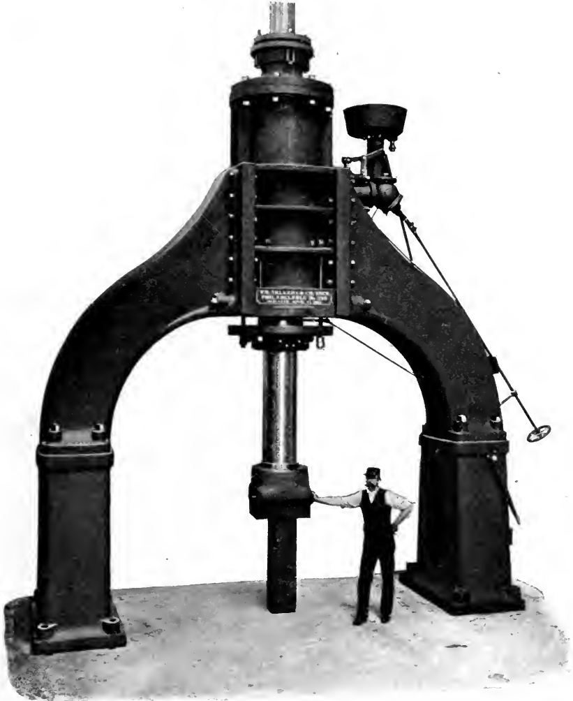
7 TON HAND-ACTING STEAM HAMMER.
