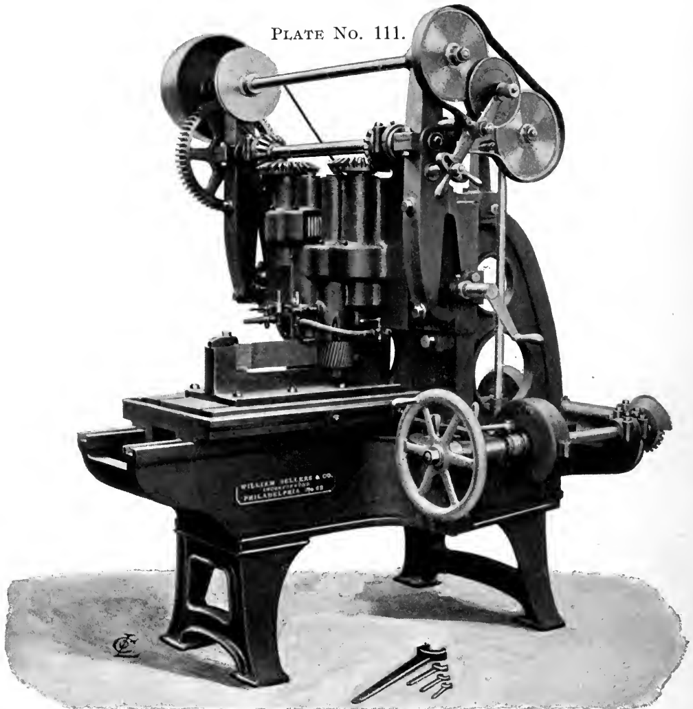
TWO-SPINDLE VERTICAL MILLING MACHINE—FOR TEST SPECIMENS.
