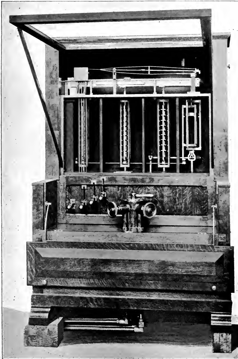
HYDRAULIC SCALE FOR EMERY TESTING MACHINES.
