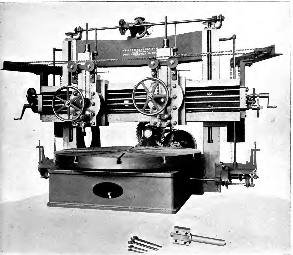
7-FOOT BORING AND TURNING MILL,—WITH TWO SADDLES.
