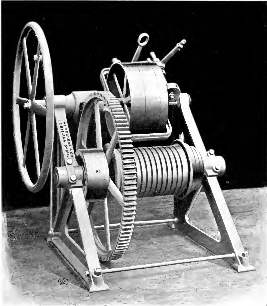
SPUR-GEARED HOISTING CRAB.—WITH WESTON RETAINING CLUTCH.
