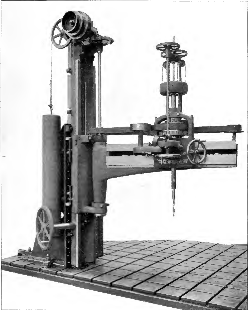
72" RADIAL DRILLING MACHINE—ARRANGED FOR ATTACHING TO A COLUMN.
