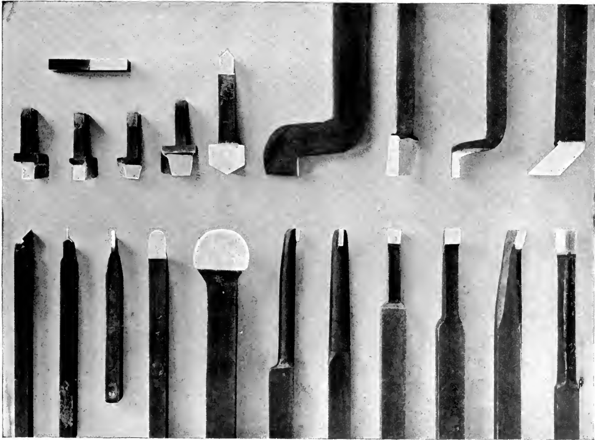
EXAMPLES OF MISCELLANEOUS THREAD, BORING, SLOTTING, AND OTHER TOOLS OF DIFFICULT SHAPES, FINISHED BY THE TOOL-GRINDING AND SHAPING MACHINE.
