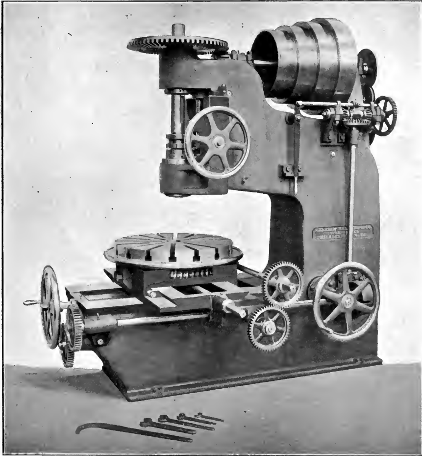
27" VERTICAL MILLING MACHINE.
