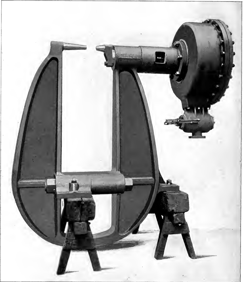
5-FT. STEAM RIVETING MACHINE—WITH EXTRA WIDE GAP.
