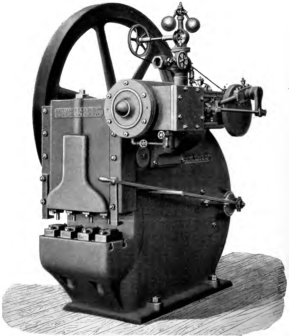
SPLICE PLATE PUNCHING MACHINE.
