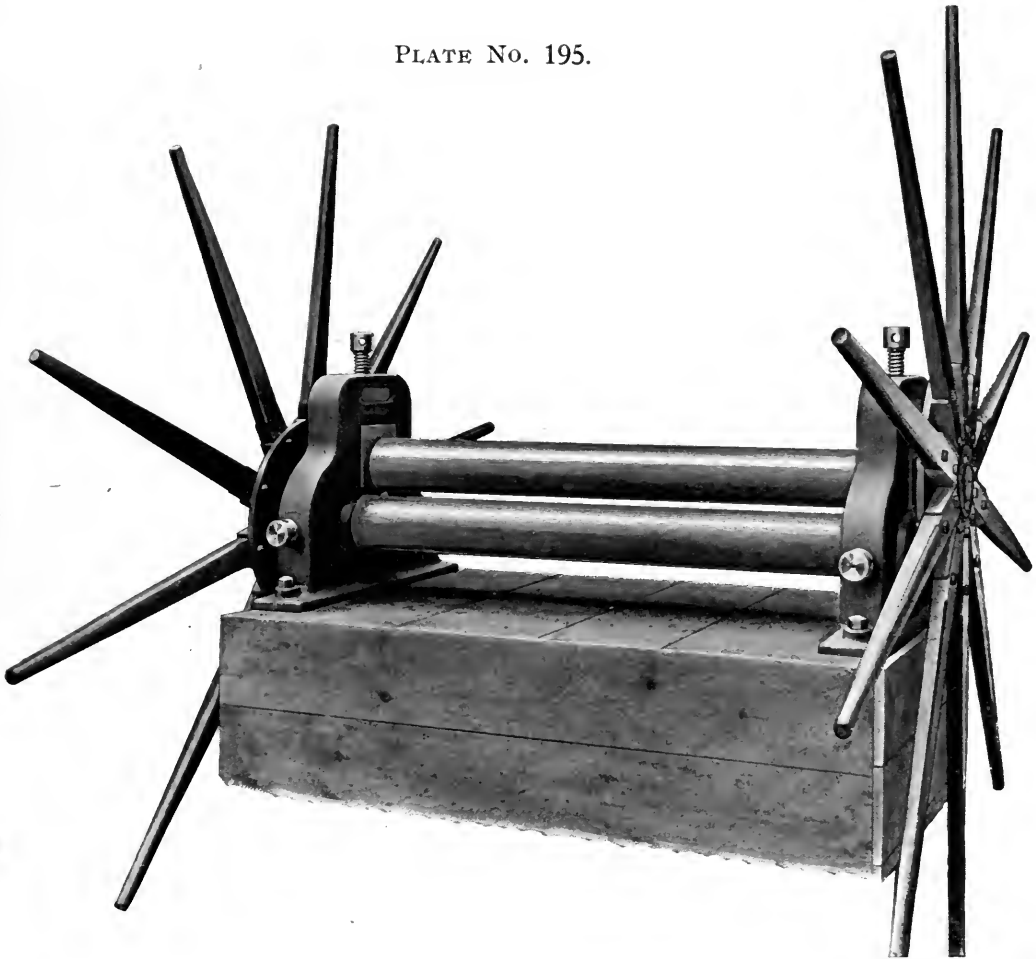
8" HAND BENDING ROLLS.—FOR LIGHT PLATES.
