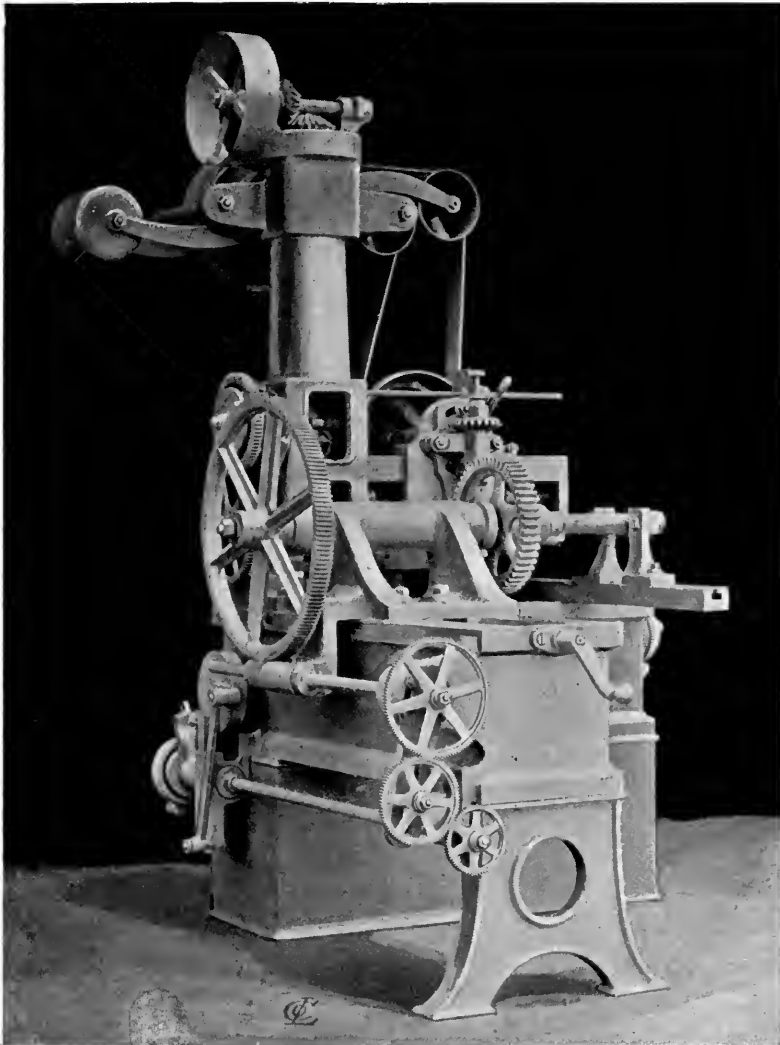
GEAR-CUTTING AND WHEEL-DIVIDING MACHINE.
