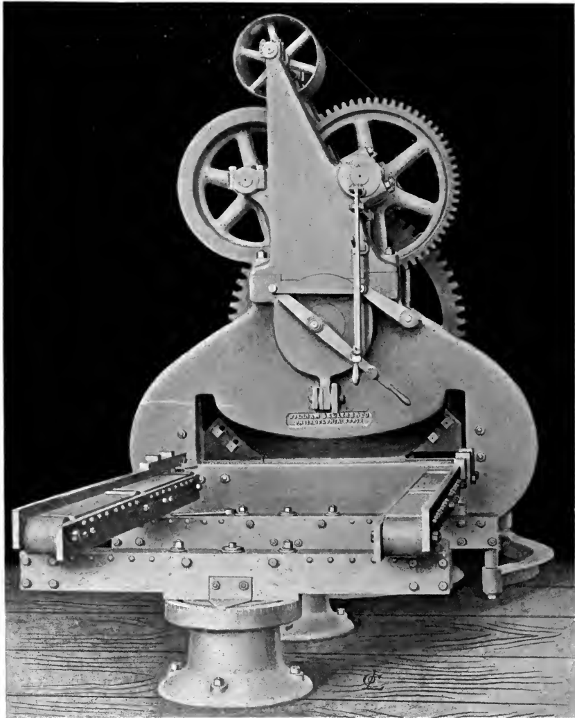
DOUBLE ANGLE SHEAR.
