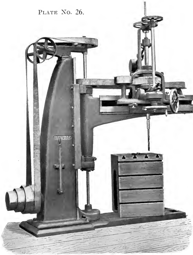
54" RADIAL DRILLING MACHINE.
