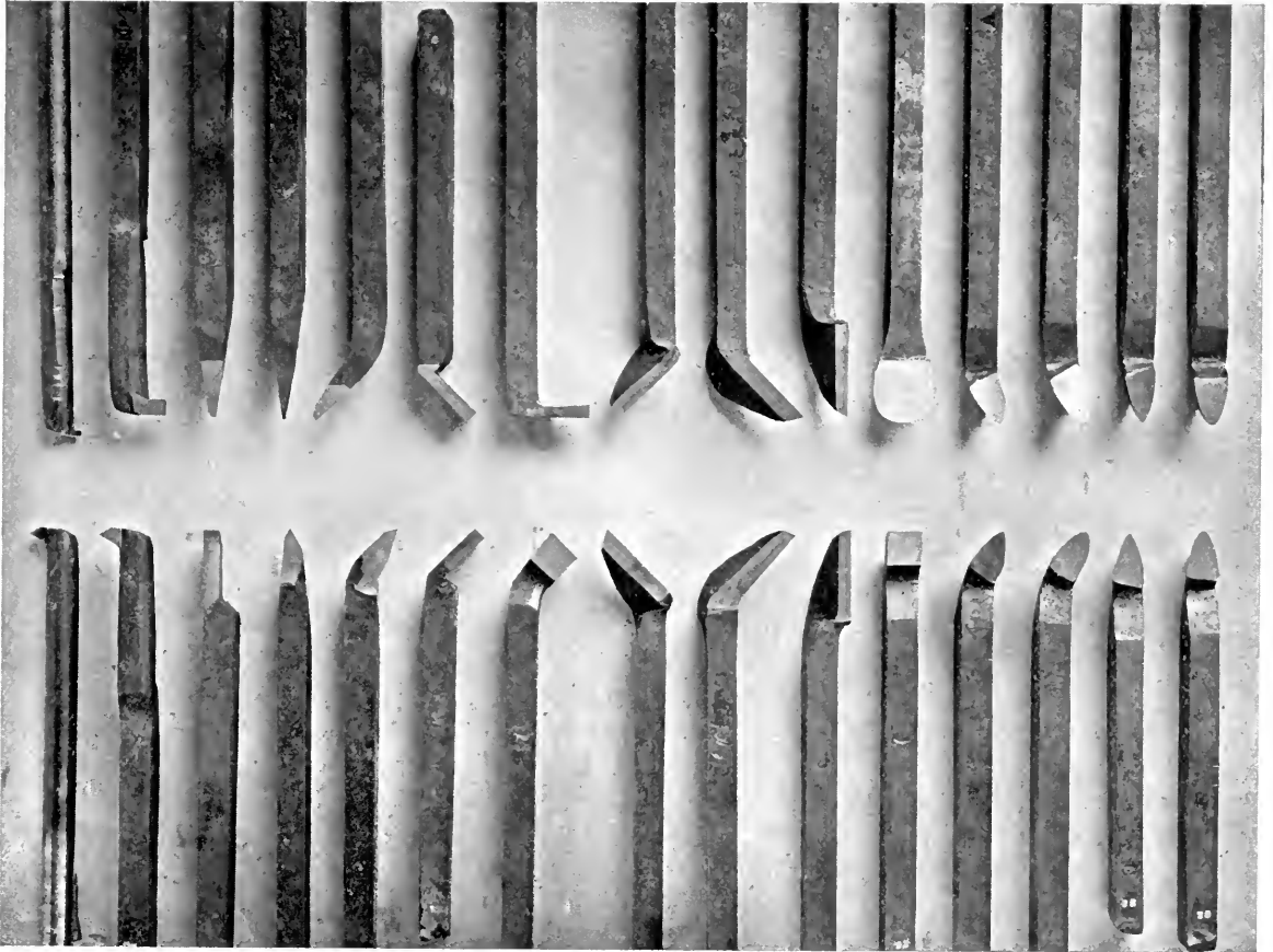
EXAMPLES OF LATHE TOOLS FINISHED TO SHAPE BY THE TOOL-GRINDING AND SHAPING MACHINE.
