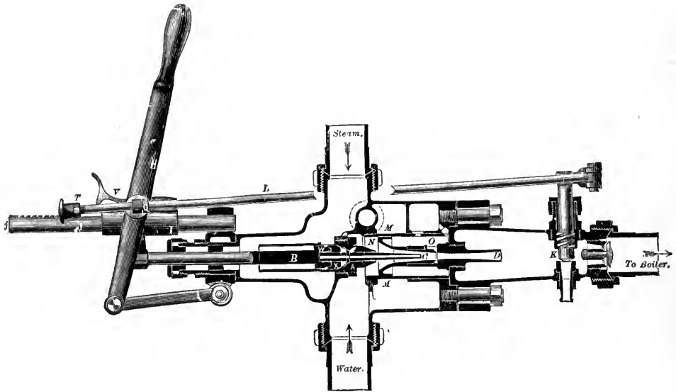
THE INJECTOR OF 1876.
