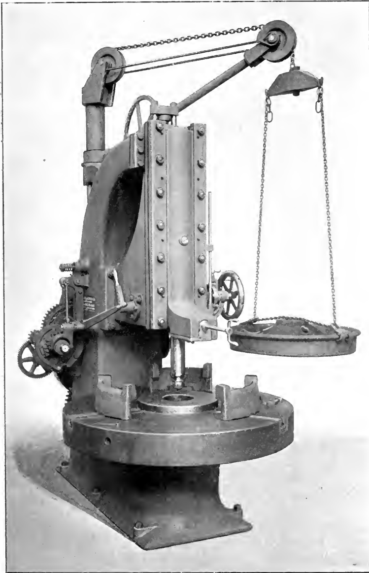
54" CAR-WHEEL BORING-MILL.
