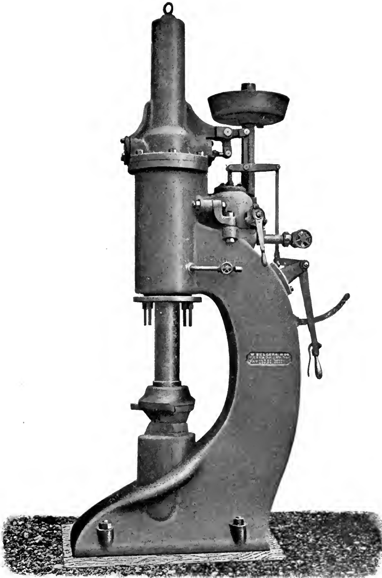
400-LB. HAND AND SELF-ACTING HAMMER.
