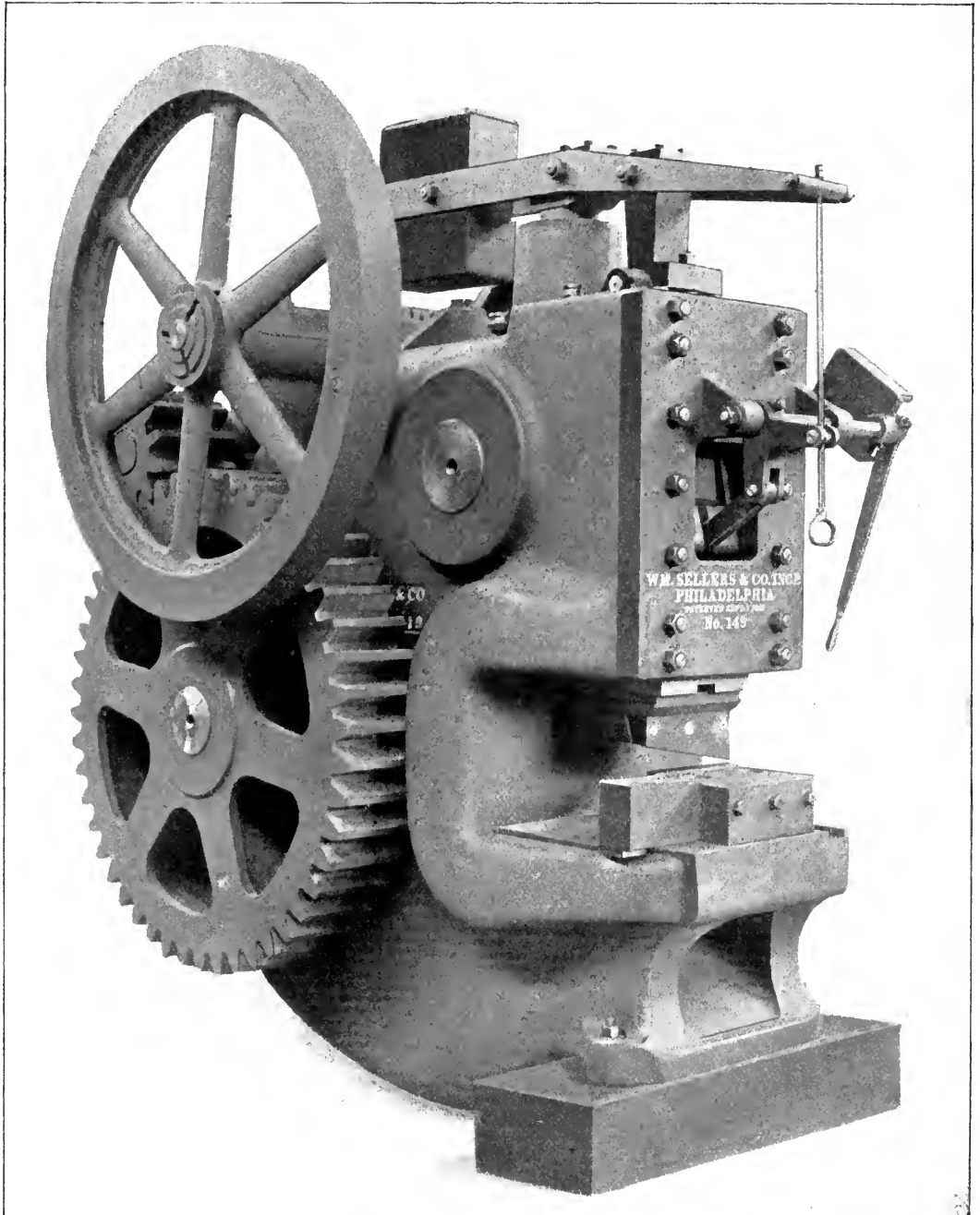
LEVER BAR SHEAR—10" OVERREACH.
