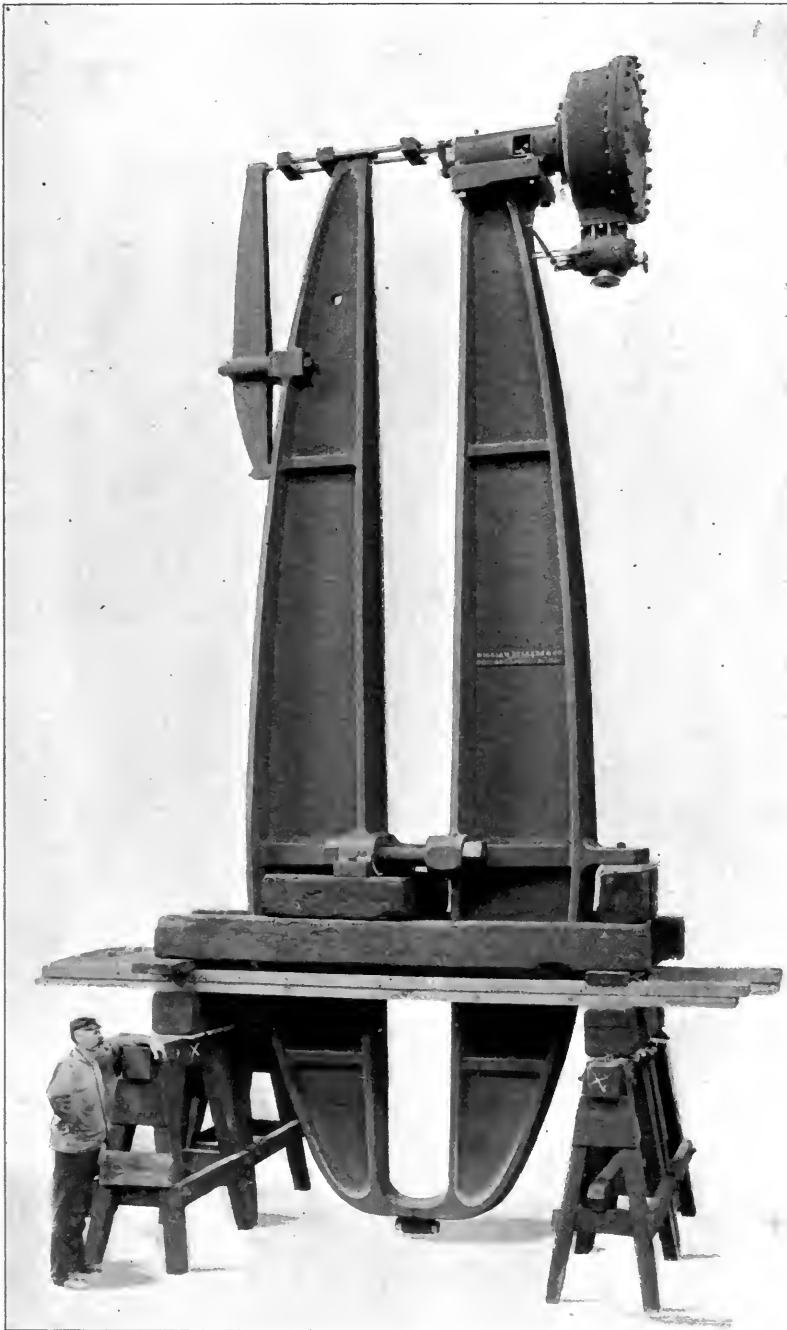
16-FT. STEAM RIVETING MACHINE WITH AUXILLIARY STAKE FOR SMALL FLUES. 36" steam cylinder and improved balanced piston valve. Auxilliary stake, for small flues, extra.
