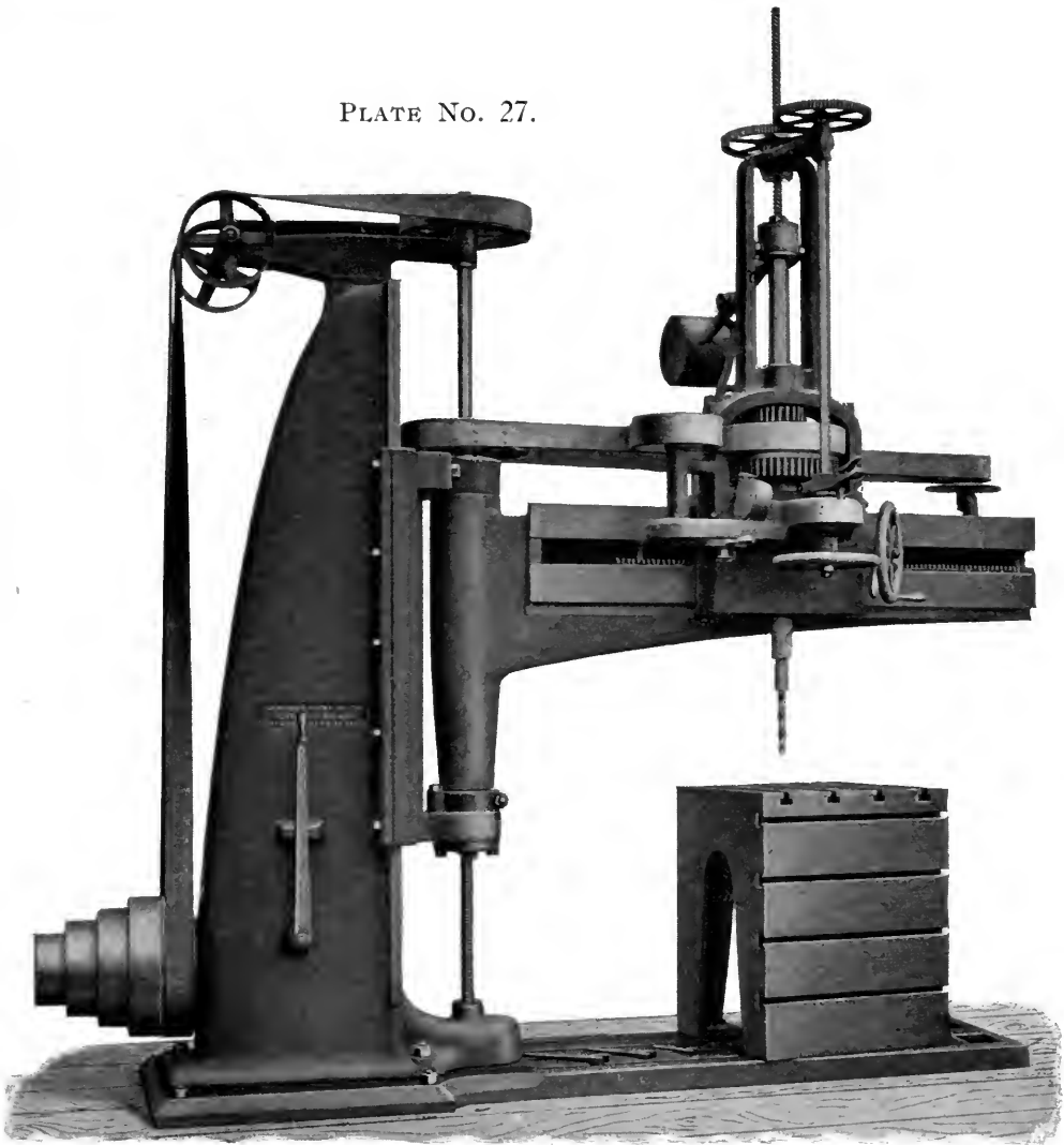
72" RADIAL DRILLING MACHINE.
