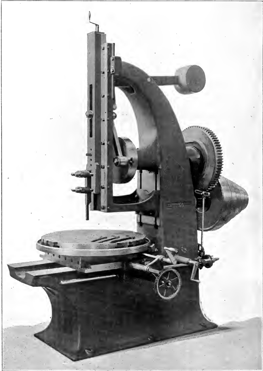
42" SLOTTING MACHINE
