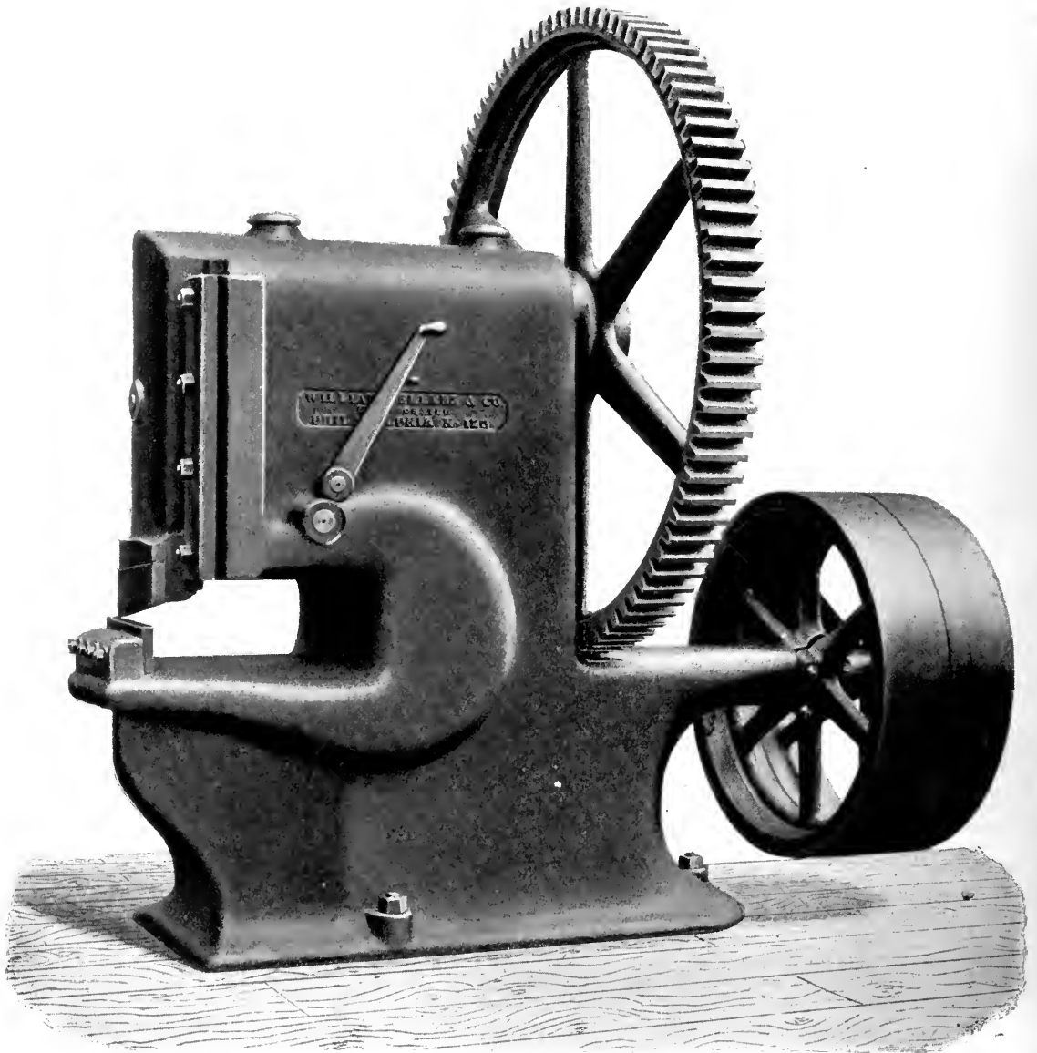
CRANK MOTION SHEAR—18" OVERREACH.
