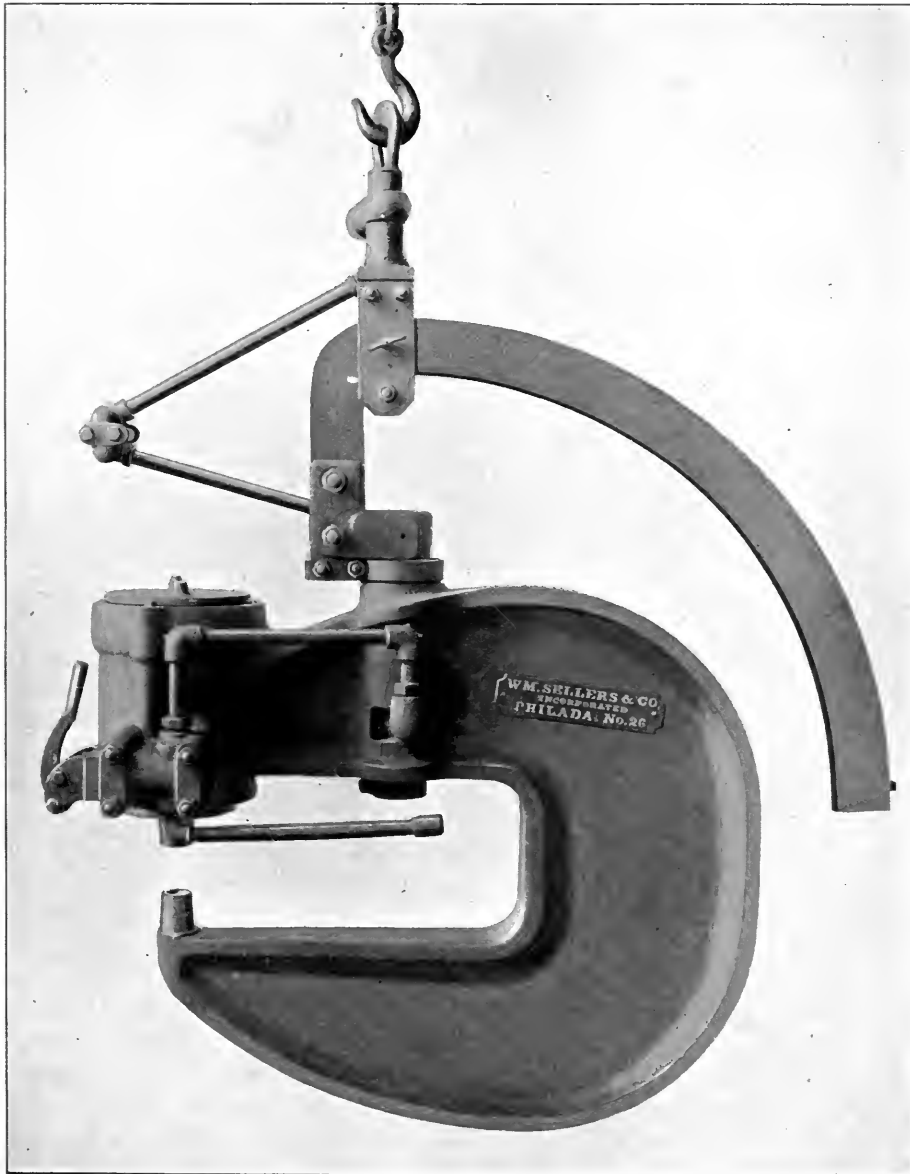
DIRECT-ACTING PORTABLE HYDRAULIC RIVETER. WITH SWIVEL HANGING BAIL.
