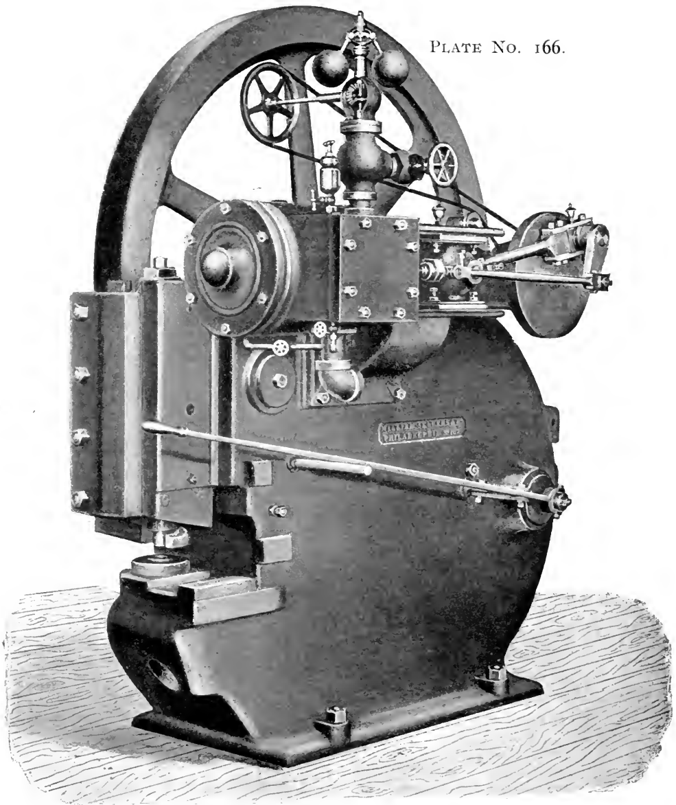
BAR SHEAR—WITH PUNCHING ATTACHMENT.
