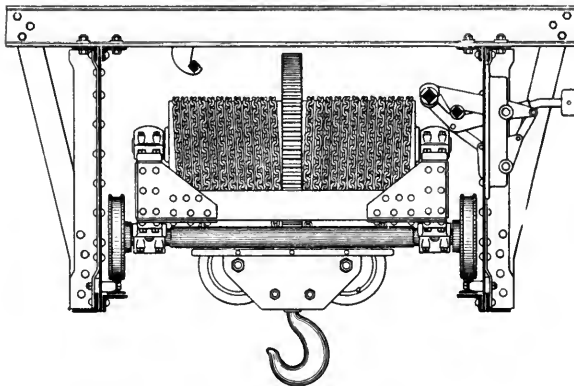
SECTION THROUGH BRIDGE WITH TROLLEY IN POSITION.
