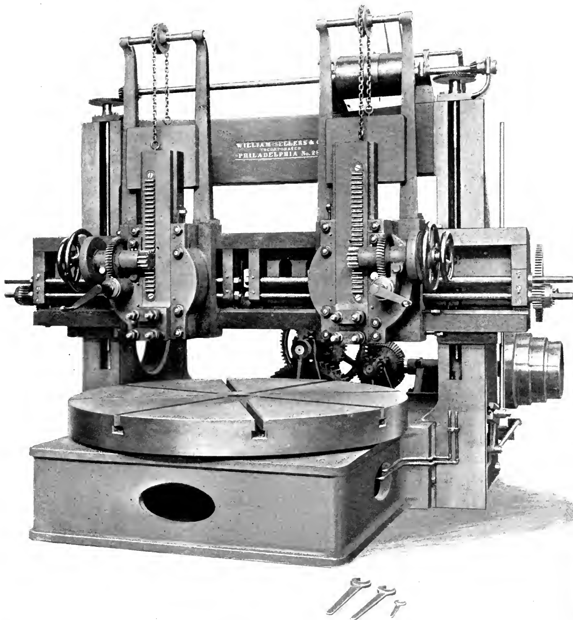
7-FOOT BORING AND TURNING MACHINE—FOR STEEL RAILWAY TIRES, ETC.
