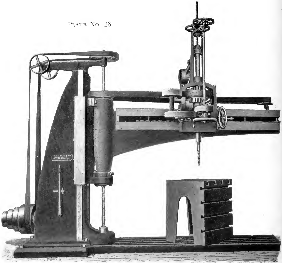
96" RADIAL DRILLING MACHINE.
