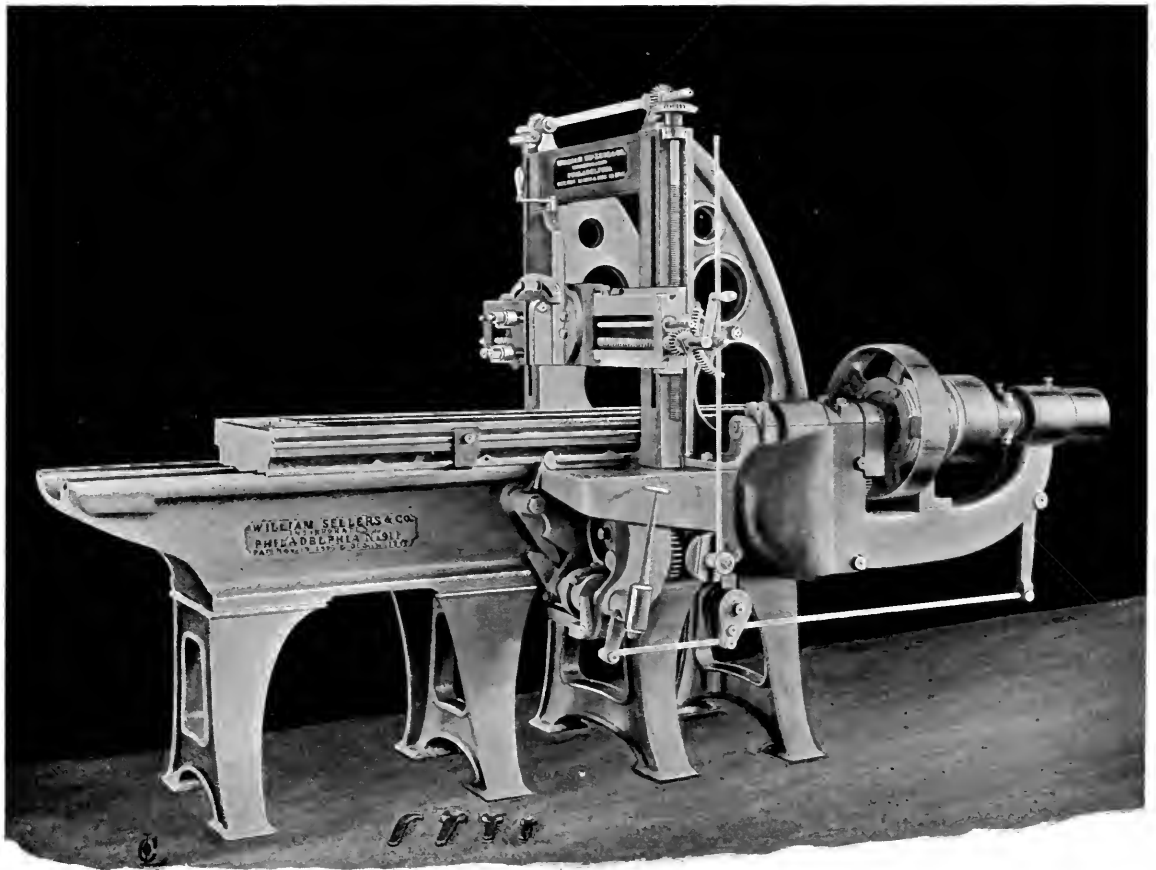
20" x 20" PATENT SPIRAL-GEARED PLANING MACHINE.
