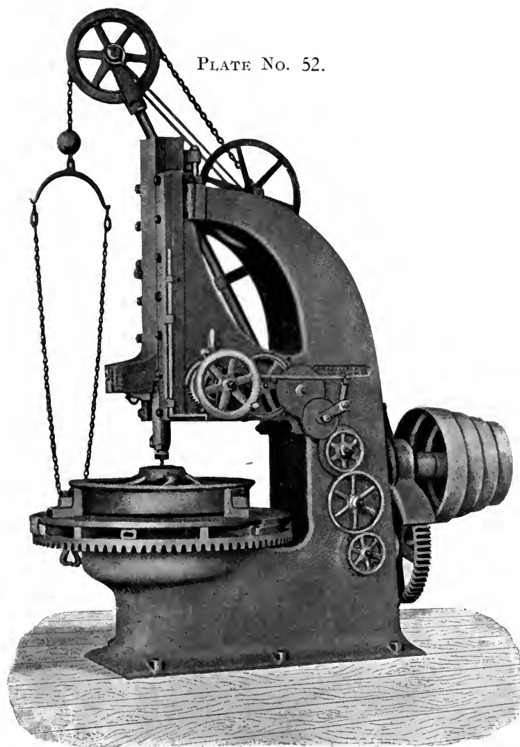
50" CAR-WHEEL BORING-MILL, No. 1.
