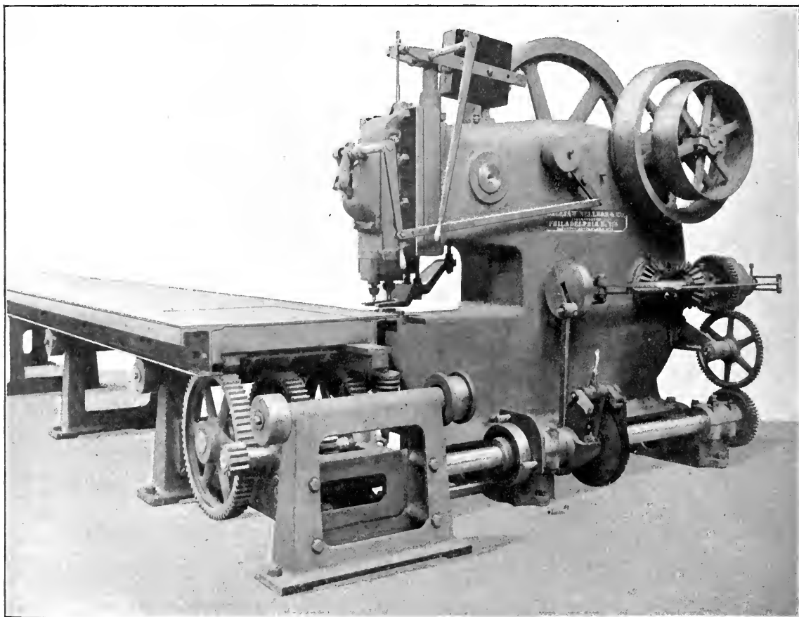
26" PUNCHING MACHINE—WITH AUTOMATIC SPACING TABLE.
