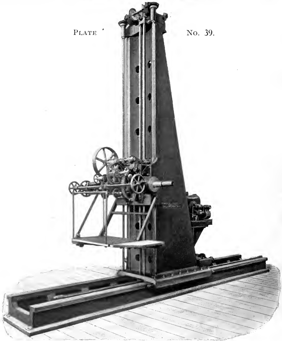
FLOOR-BORING MACHINE ON INDEPENDENT BED. DRIVEN BY ELECTRIC MOTOR.
