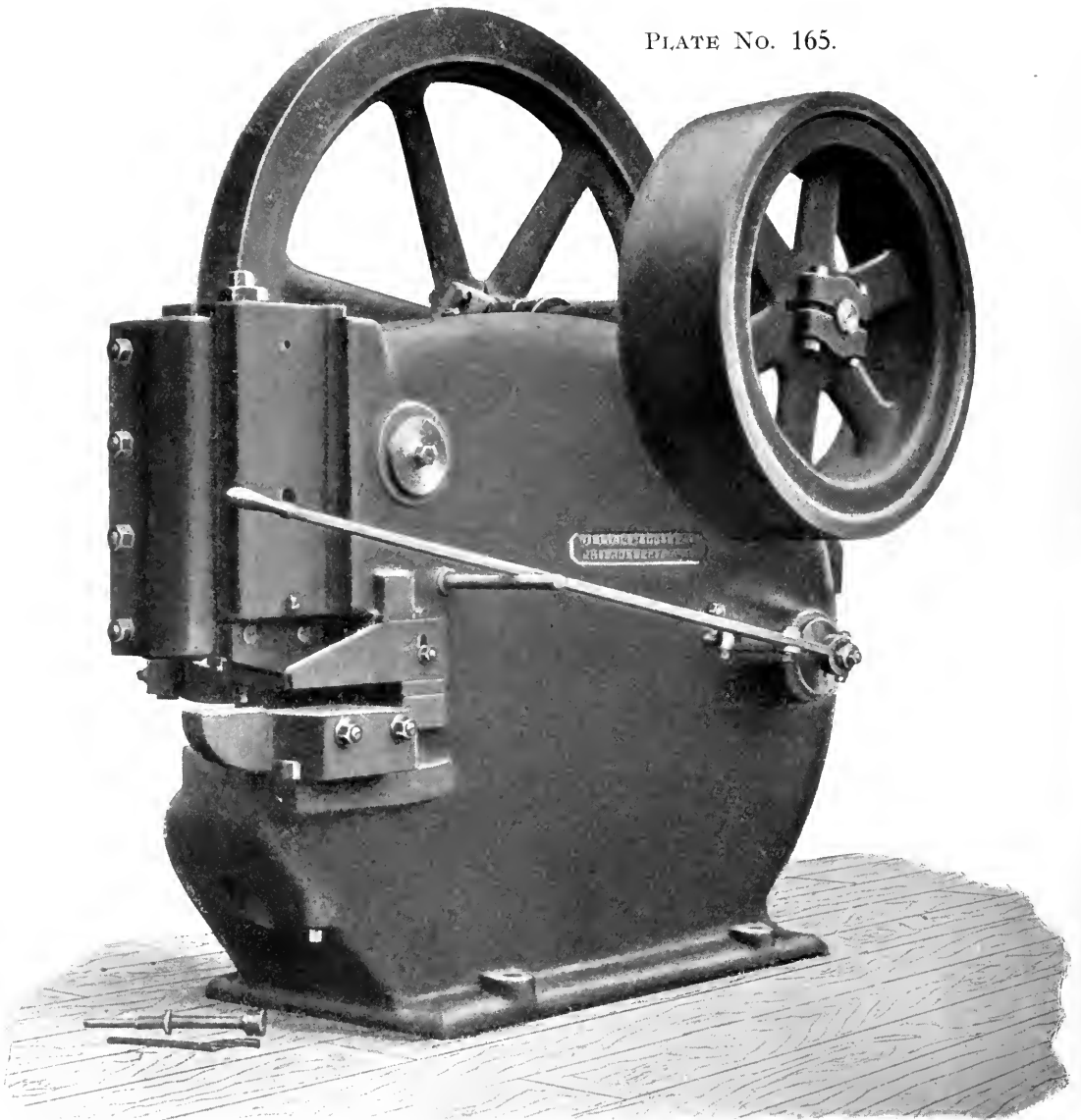
BAR SHEAR—WITH PUNCHING ATTACHMENT.
