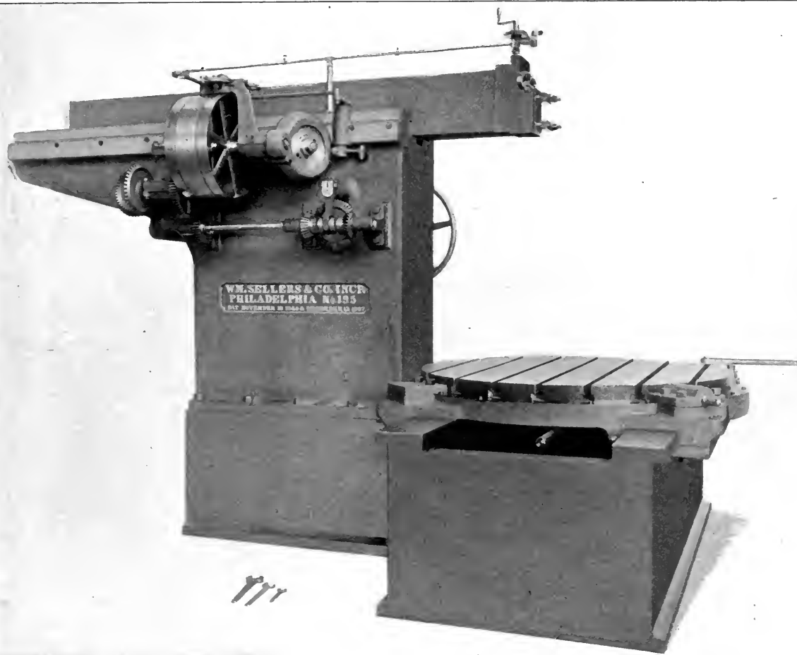
CYLINDER SHAPER.
