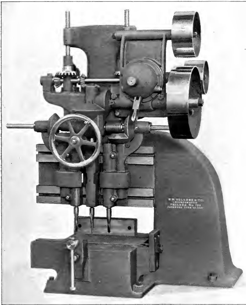
THREE-SPINDLE RAIL DRILLING MACHINE—WITH POST ON ONE SIDE.
