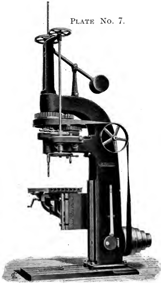
45" VERTICAL DRILLING MACHINE—WITH COMPOUND TABLE.
