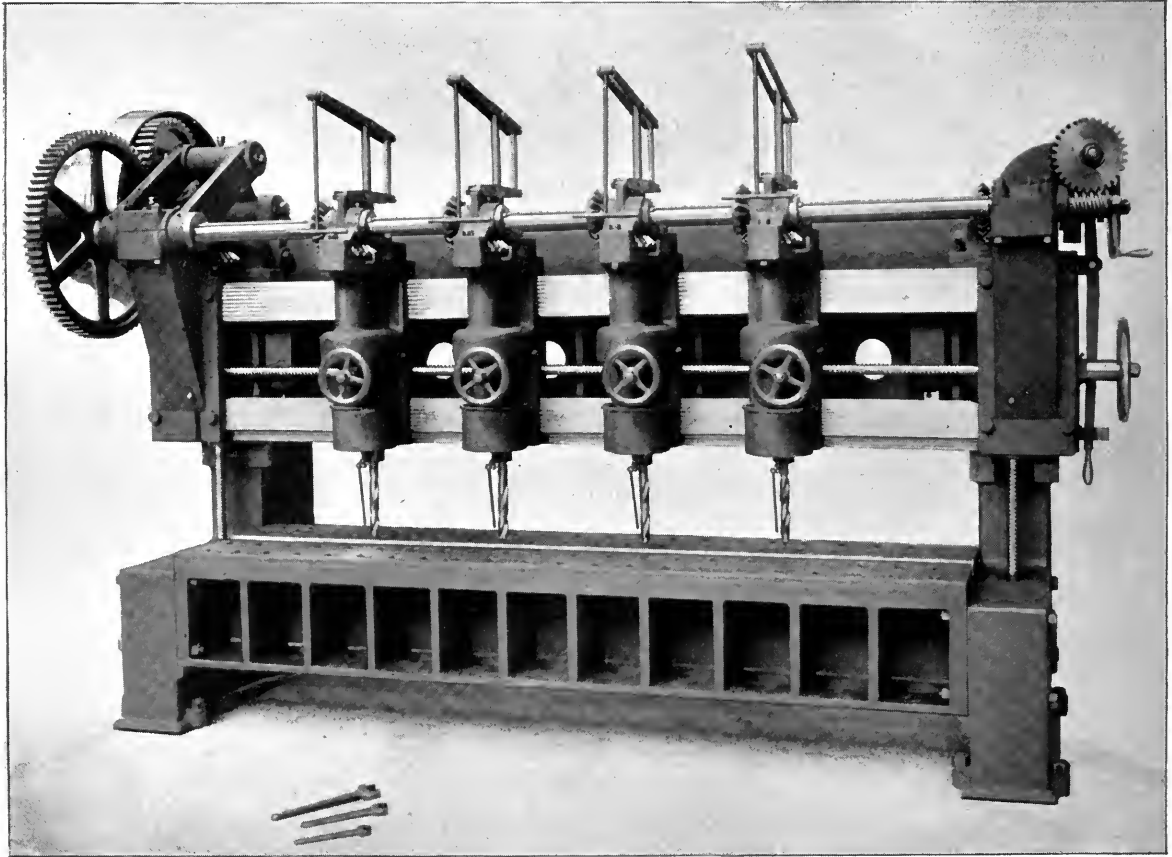
FOUR-SPINDLE VERTICAL DRILLING MACHINE.
