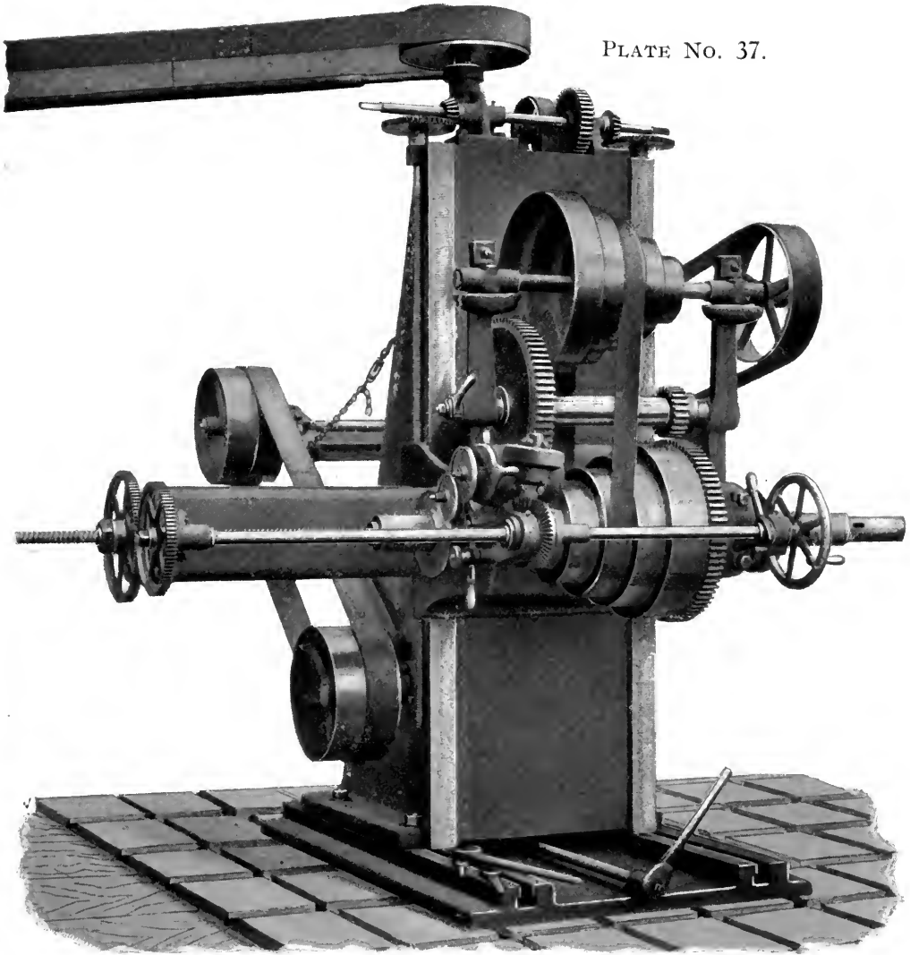
FLOOR-BORING MACHINE—DRIVEN BY BELT AND SWING FRAME.
