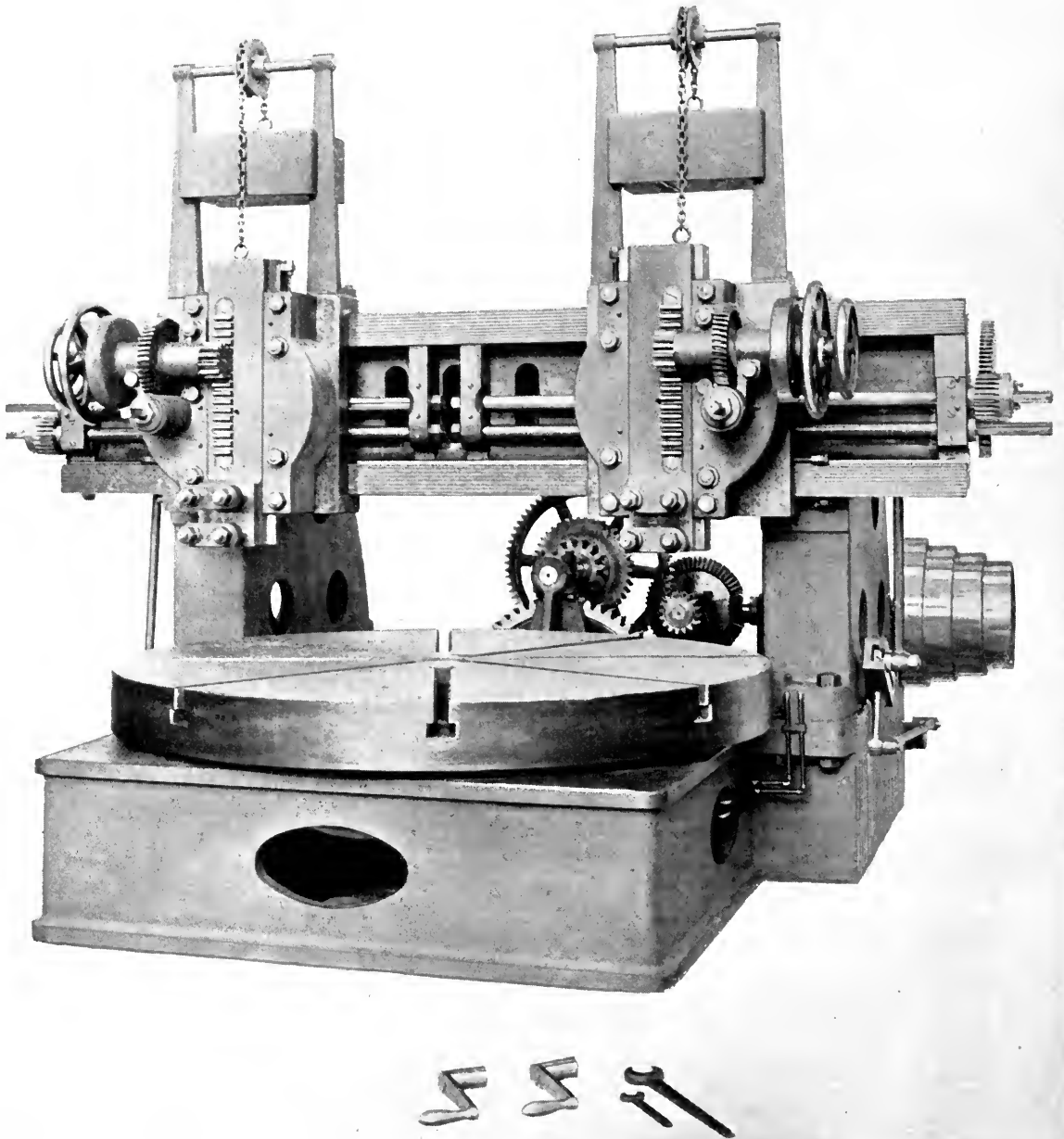
6-FOOT BORING AND TURNING MILL—FOR STEEL RAILWAY TIRES.
