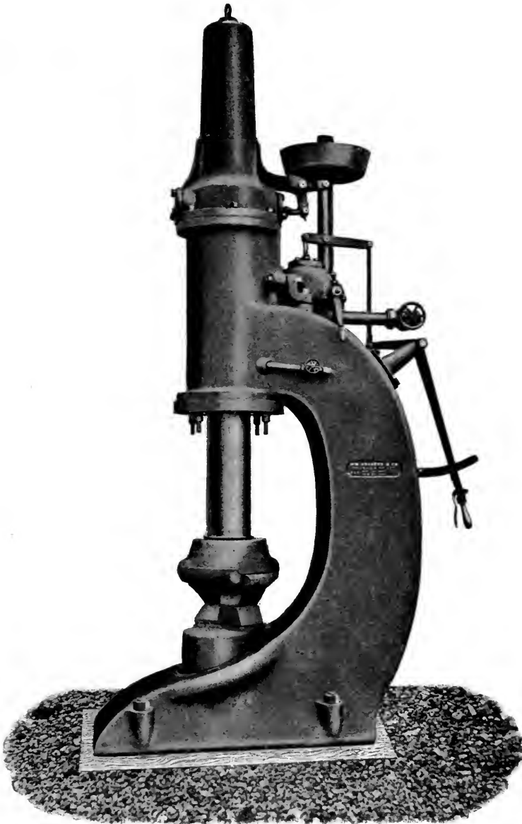
1250-LB. HAND AND SELF-ACTING HAMMER.
