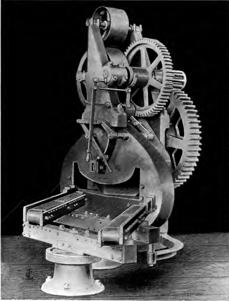
DOUBLE ANGLE SHEAR.
