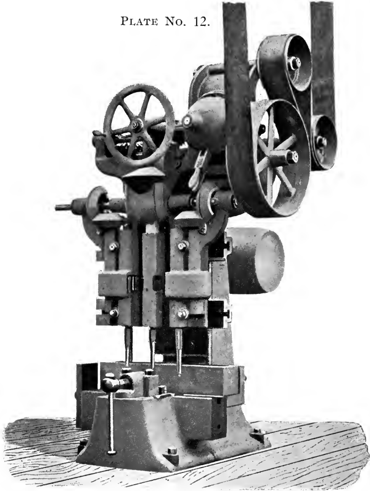
THREE-SPINDLE RAIL DRILLING MACHINE.
