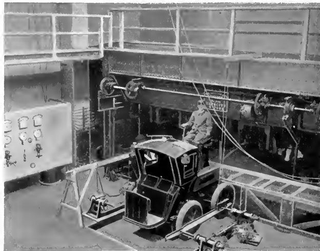
8-TON TRAVELLING CRANE.—FOR HANDLING STORAGE BATTERIES IN THE POWER HOUSE OF THE ELECTRIC VEHICLE CO., NEW YORK.
