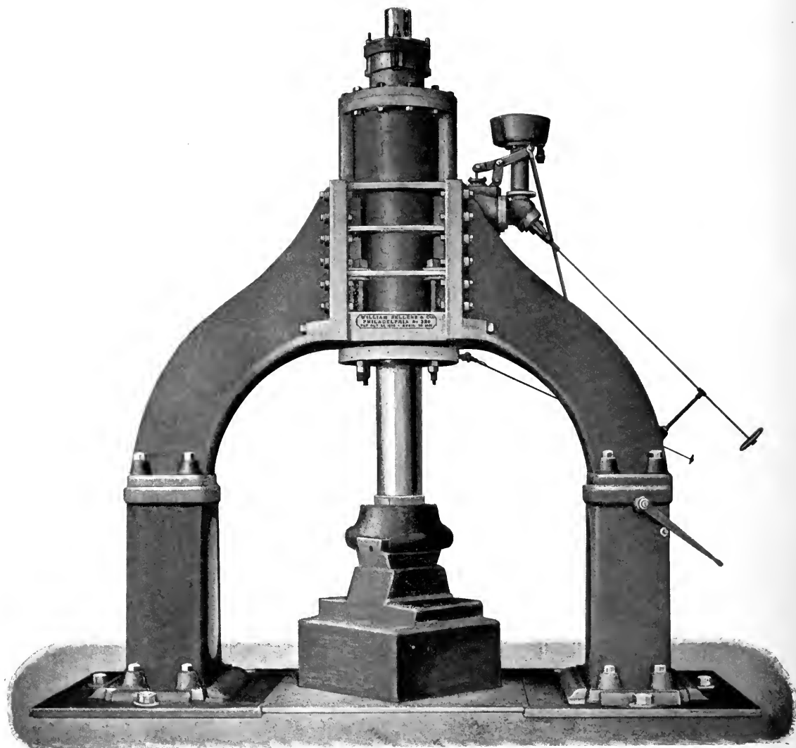
2¼ TON HAND-ACTING STEAM HAMMER.
