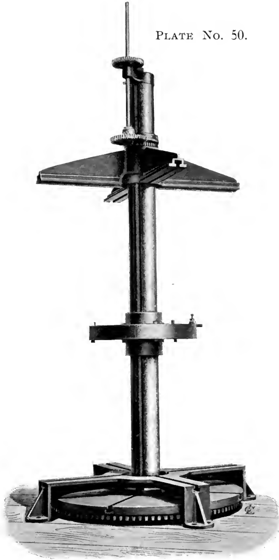
VERTICAL CYLINDER BORING-BAR.
