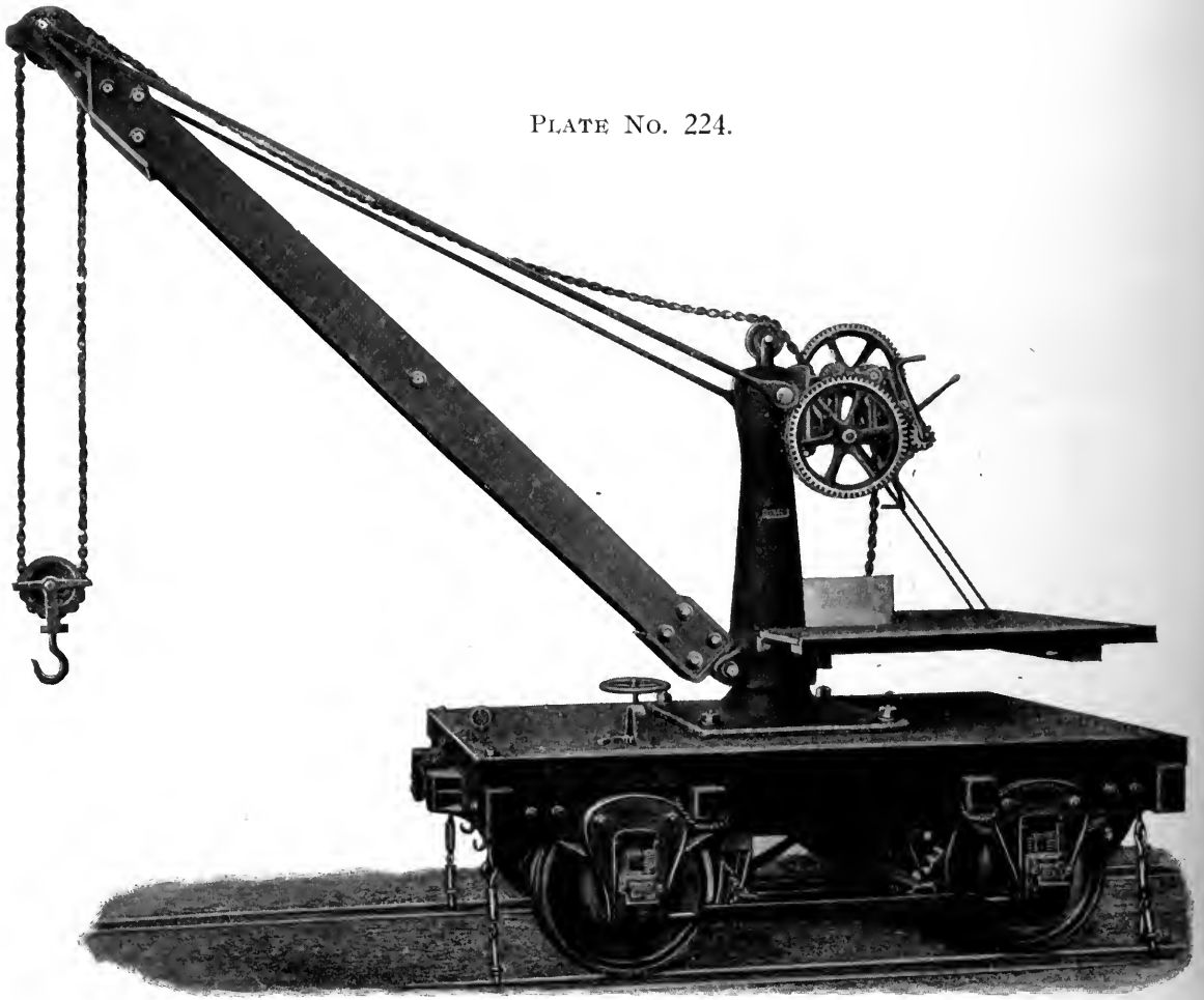
5-TON CAR CRANE.
