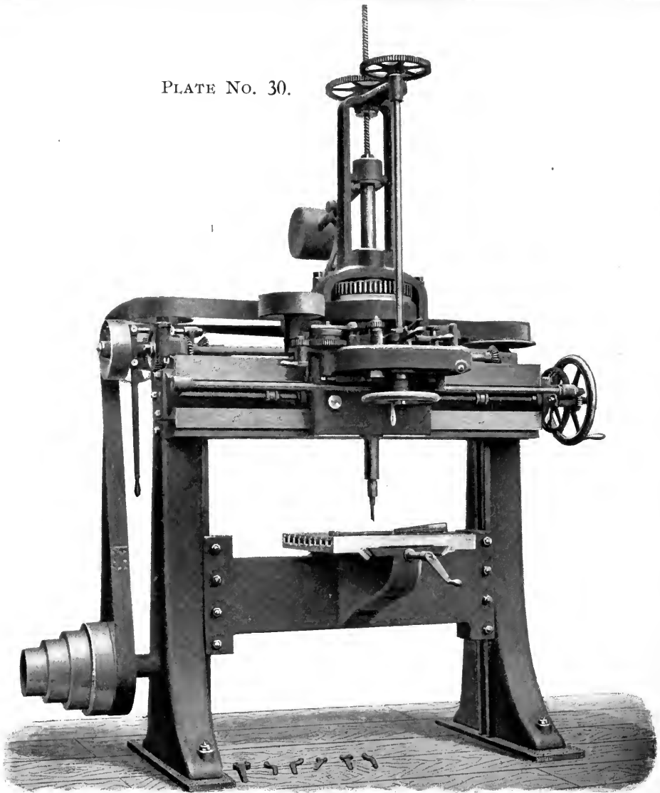
TRAVERSE-DRILL WITH COTTER DRILLING ATTACHMENT. FOR KEYSEATS, SLOTS, ETC.
