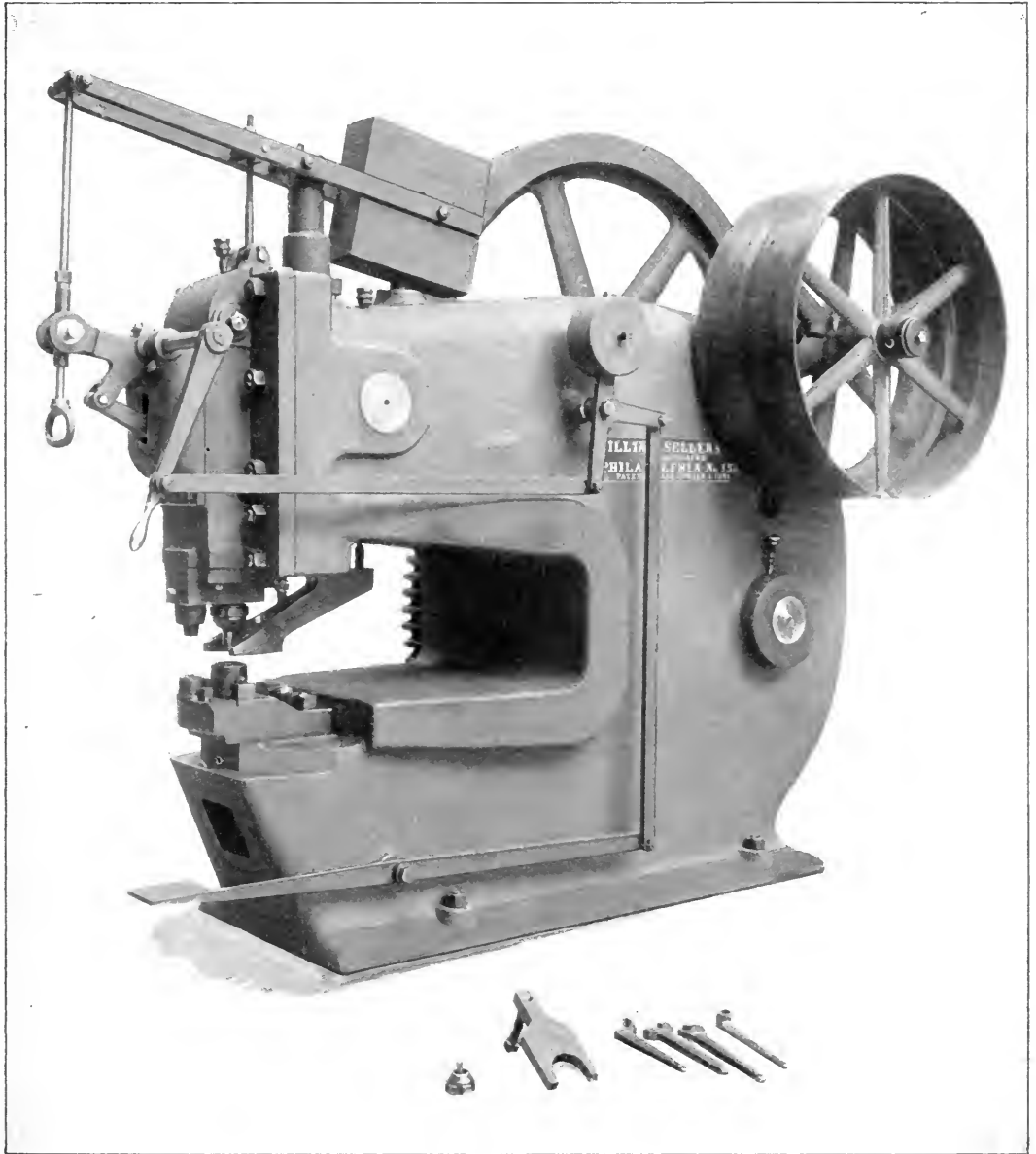
33" PUNCHING MACHINE.
