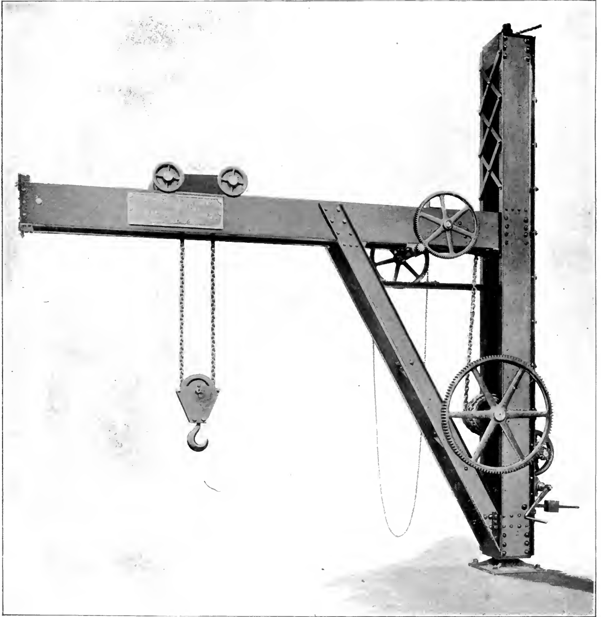
6-TON IRON HAND-POWER JIB-CRANE.
