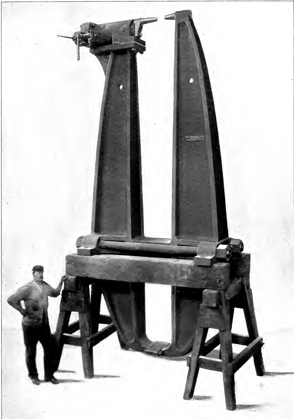
10 FT. HYDRAULIC RIVETING MACHINE.
