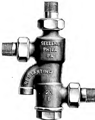
SCREWED CONNECTION.
