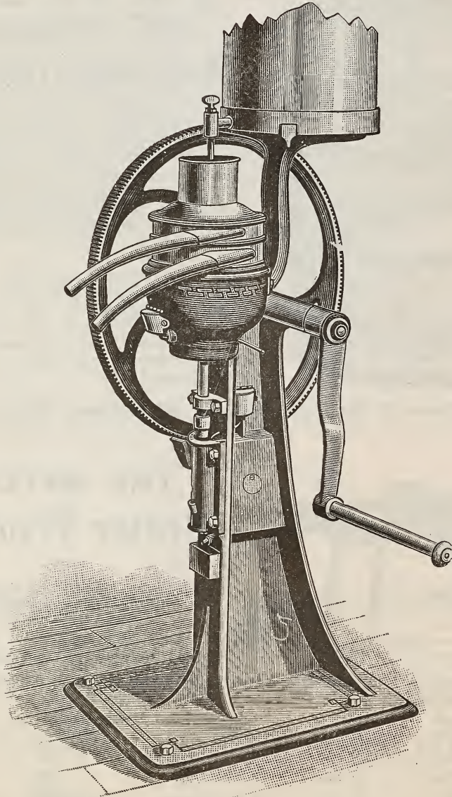
THE DE LAVAL "BABY" HAND SEPARATOR.
