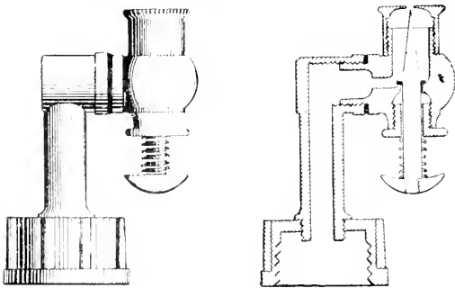
Fig. 81. IMPROVED VERMOREL NOZZLES.
