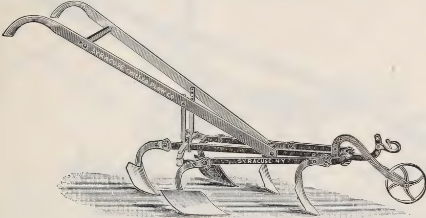
No. 53,—Five 3 inch Points, Wing Points and Shovel Point..... $4.00
