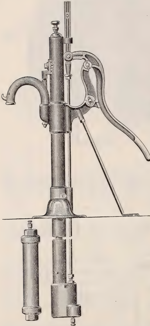
The Thomas Double-Acting Force and Lift Pump.
