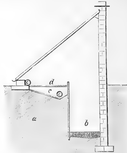
FIG. 191. SECTION OF LEAN-TO PIT.
