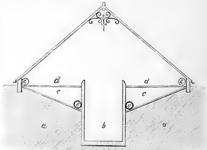
FIG. 192. SECTION OF SPAN-ROOFED PIT.
