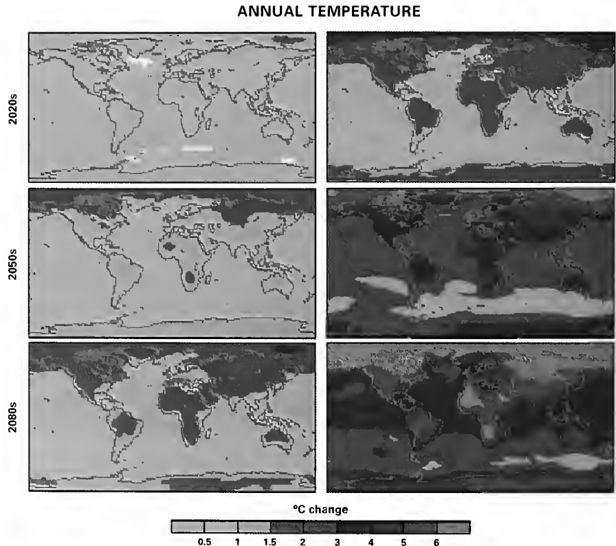
Figure 1. (Left panels) Change in mean annual temperature for the 2020s, 2050s and 2080s (with respect to 1961–90) for the B1-low scenario; median of 10 model simulations. (Right panels) As left, but for the A2-high scenario.
