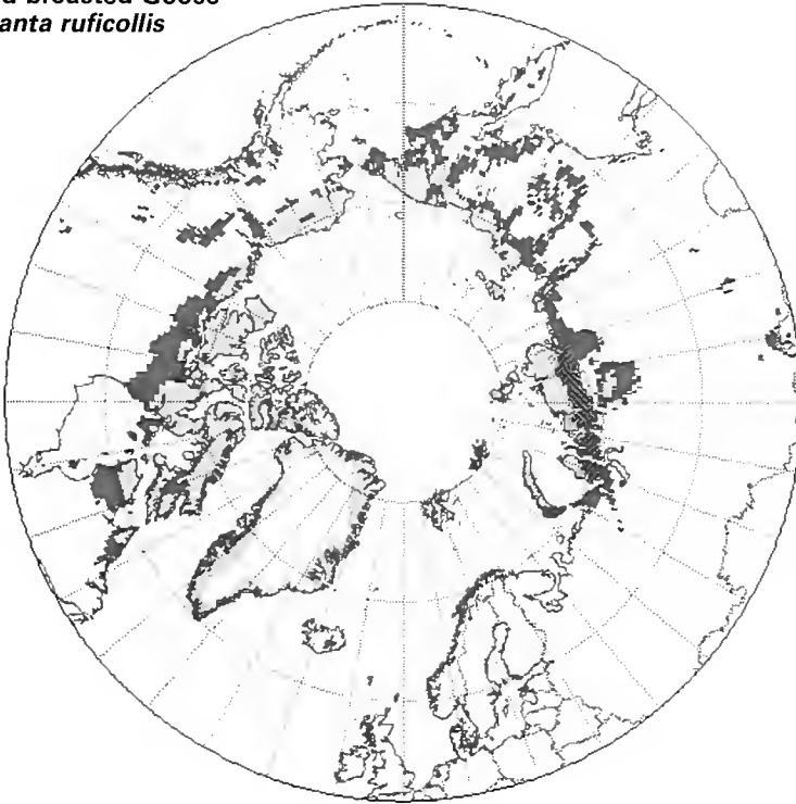
Figure 2. Current breeding distribution and predicted changes in breeding habitat (2070-2099) of the Red-breasted Goose Branta ruficollis (top map) and the Knot Calidris canutus (bottom map).
