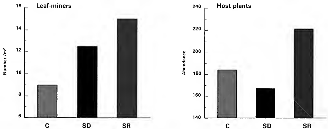
Figure 2. Leaf-miner and host plant responses to summer water manipulations. As in Figure 1, vegetation cover is promoted by supplemented summer rainfall (SR) and decreased by summer drought (SD) in comparison with the control (C). Leaf-miners would be predicted to respond in relation to the vegetation (as for SR), but under SD leaf-miner populations do not crash. Here, these insect herbivores are responding to changes within host plant physiology caused by drought stress, where nutrient levels increase leading to a better quality diet; their performance and subsequent populations therefore increase.
