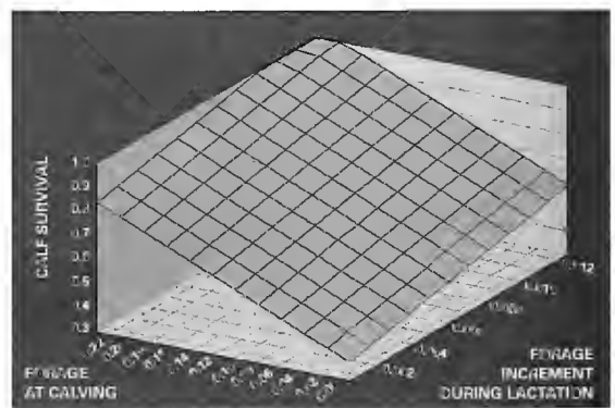
Figure 4. Relationship of Caribou calf survival to the amount of forage available to cows at calving and to the rate of increase in available forage during lactation, Porcupine Caribou herd, Alaska and Canada, 1985–1996.
