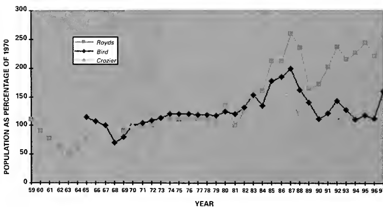
Figure 1. Changes in the numbers of pairs of Adélie Penguin breeding at three colonies (Capes Royds, Bird and Crozier) on Ross Island, Antarctica, 1959–1997. Current numbers at these colonies are: Royds – 4,000 pairs, Bird – 45,000 pairs, Crozier – 170,000 pairs (data from Wilson et al. 2000, in press). Numbers are expressed as percentages of those in 1970.
