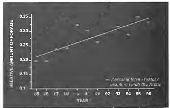
Figure 3. Annual trend in the relative amount of green plant biomass available to lactating cows of the Porcupine Caribou herd in late-June, 1985–1996.
