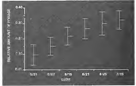
Figure 2. Seasonal profile of the relative amount of green plant biomass on the calving grounds of the Porcupine Caribou herd, Alaska and Canada. Averages from late May to early July, 1985–1996.
