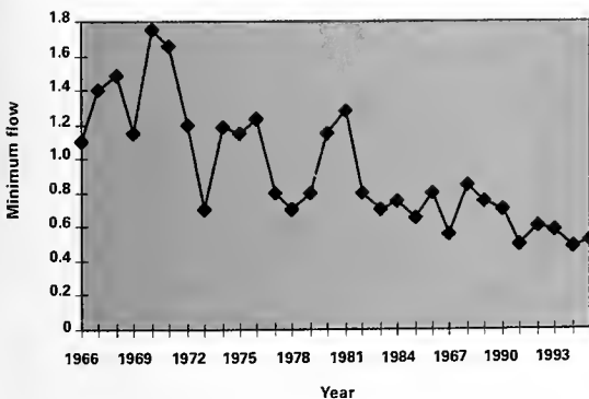
Figure 1. The minimum daily average rate of stream flow (in cubic metres per second) 1966–1995 in the Rio Cañas near Monteverde Cloud Forest Preserve.
