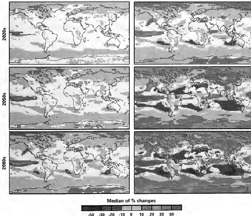
Figure 2. (Left panels) Change in mean annual precipitation for the 2020s, 2050s and 2080s (with respect to 1961–90) for the B1-low scenario; median of 10 model simulations. (Right panels) As left, but for the A2-high scenario.
