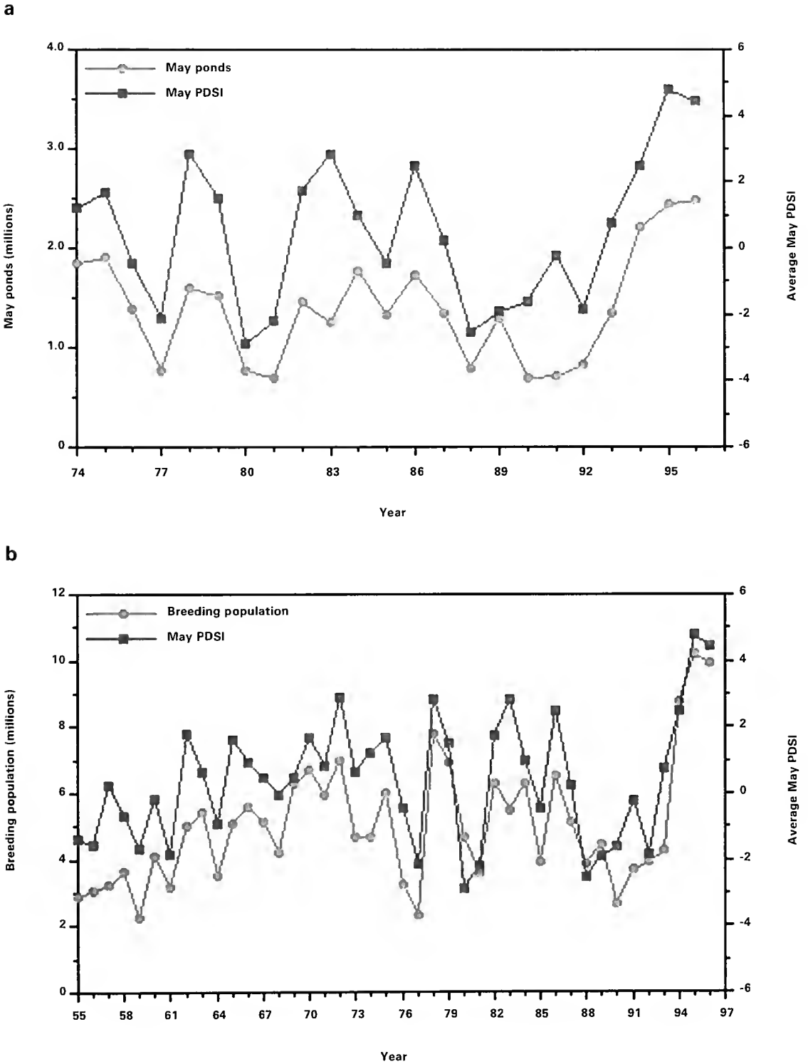
Figure 1. Number of May ponds (a) and May breeding duck population estimates (b) shown in relation to average May Palmer Drought Severity Index (PDSI) values for the north-central USA portion of the Prairie Pothole Region.
