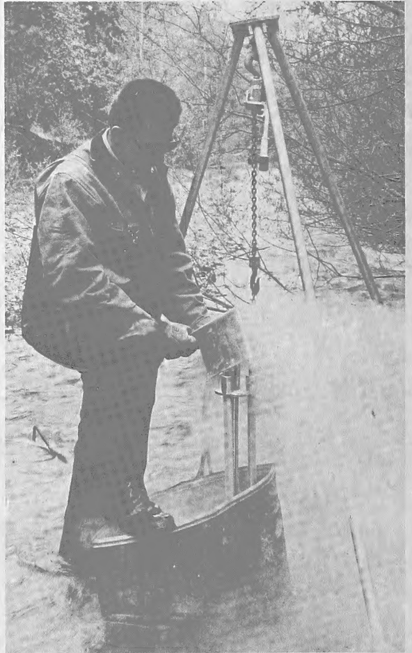
Figure 1. Tri-tube sampler in operation.
