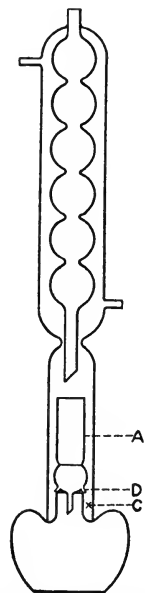
FIG. 1.—Old form of Knorr extraction apparatus.
