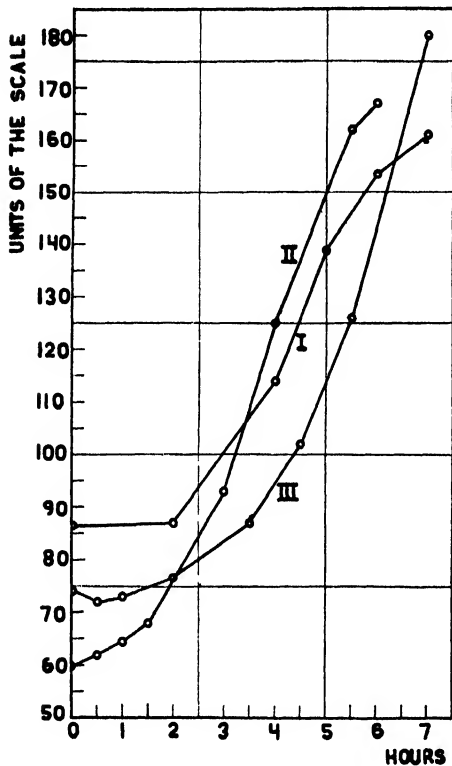
Fig. 4. Some growth curves measured with the nephelometer.
