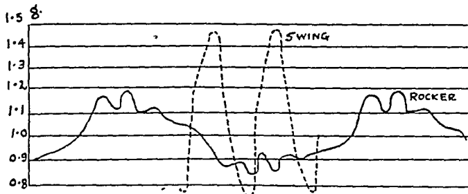
Fig. 3.—Accelerometer readings taken on the pitch-roll rocker and the standard swing. The period of the rocker due to pitch was 8 cycles per minute; the period of the swing, 15 cycles per minute.
