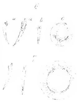
Fig. 6. Poison fang of the cobra, a. Back view. a. „ part of the outer layer removed. b. Front view. c. Section, enlarged.
