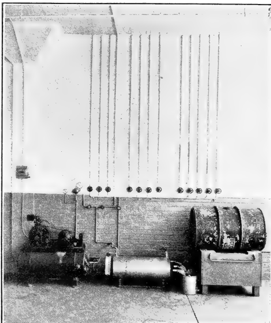
FIGURE 37.—Exterior view of commercial fur-storage vault equipped for fumigation with ethylene dichloride-carbon tetrachloride mixture. Note storage drum at right, pump at left, and pressure tank in center connected with various fumigating vaults, not shown, by pipe lines on wall.
