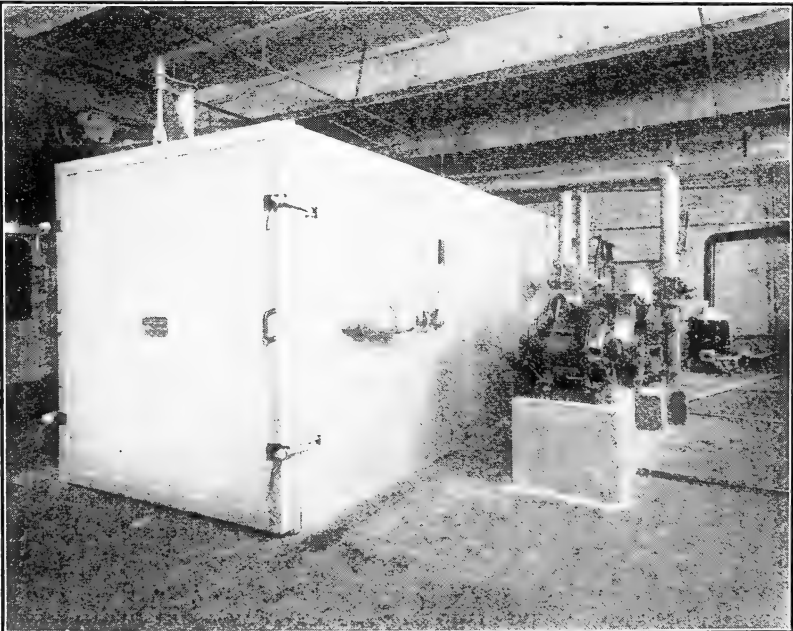
FIGURE 30.—New type of rectangular fumigation chamber. Note vacuum pump at right, with temperature and vacuum gages and other equipment behind it.
