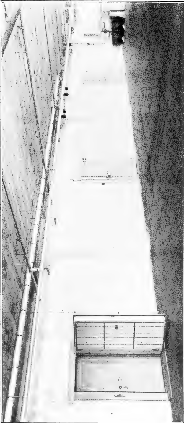
FIGURE 32.—Battery of three large fumigable fur-storage vaults constructed in a modern concrete building, equipped with devices for regulation of temperature and humidity, and for introducing and taking out the fumigant, as well as with burglar alarms. At right on warehouse floor, note storage for fumigant and pump for forcing fumigant to any room desired. These rooms have been operated successfully in southern California for more than 15 years.
