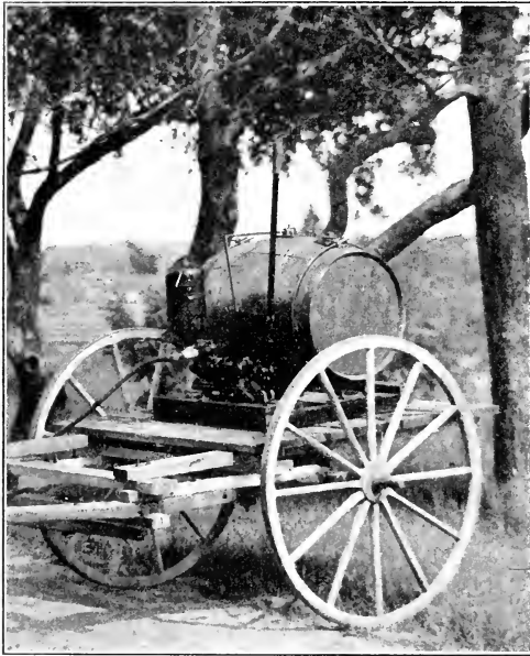
FIG. 62. — A horizontal pump. Original.
