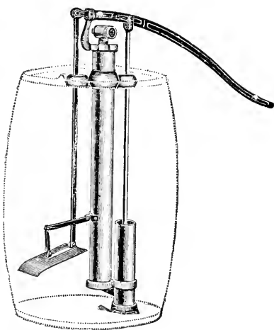
FIG. 34.—A desirable type of barrel pump embodying most of the features described. (Morrill & Morley.)
