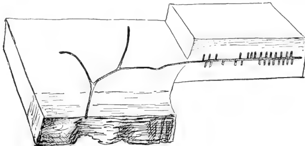
Fig. 53 Galleries of Monarthrum mali in maple. (After Hubbard, U. S. Dep't Agric. Div. Ent. Bul. 7, 1897)
