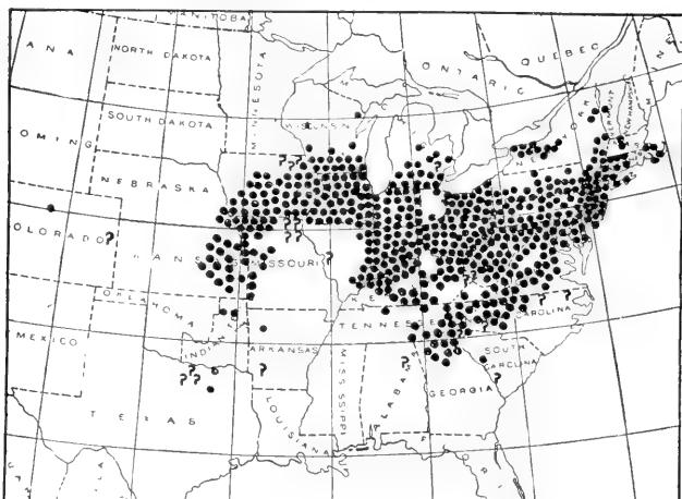
FIG. 23. Map showing the distribution of the broods of the 17 year race. (After Marlatt, U. S. Dep't Agric. Div. Ent. Bul. 14, n. s. 1898, p. 26)
