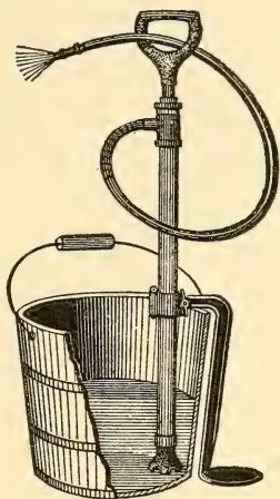
Fig. 23.—Hand bucket pump
