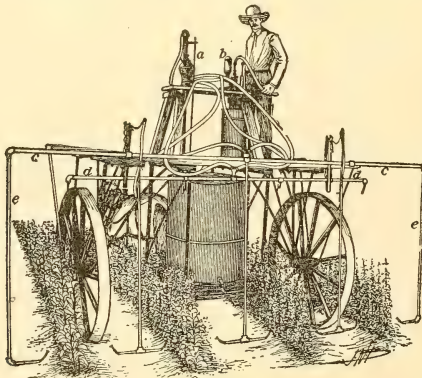
Fig. 24.—A four-row sprayer. (After Washburn)
