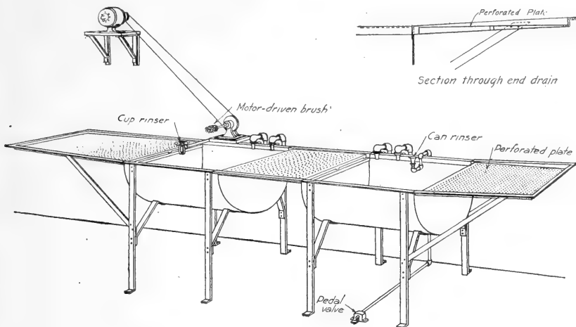
FIG. 21.—Sinks in sterilizing room, showing arrangement of cup rinsers, motor-driven brushes, drains, and can rinsers with pedal valve attachment.
