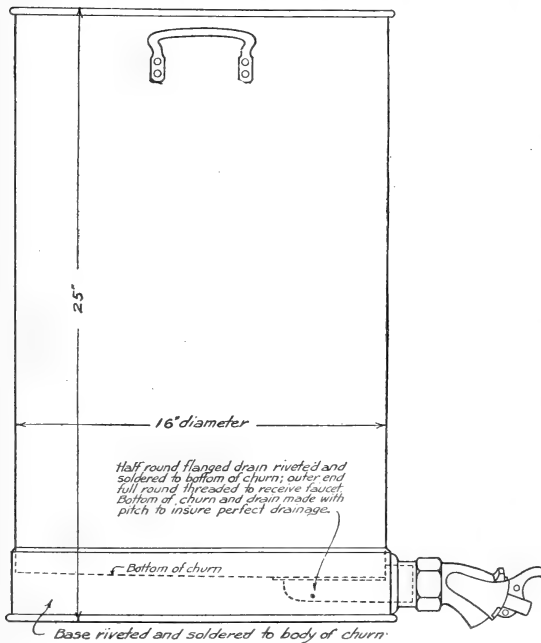
FIG. 19.—Churn barrel.
