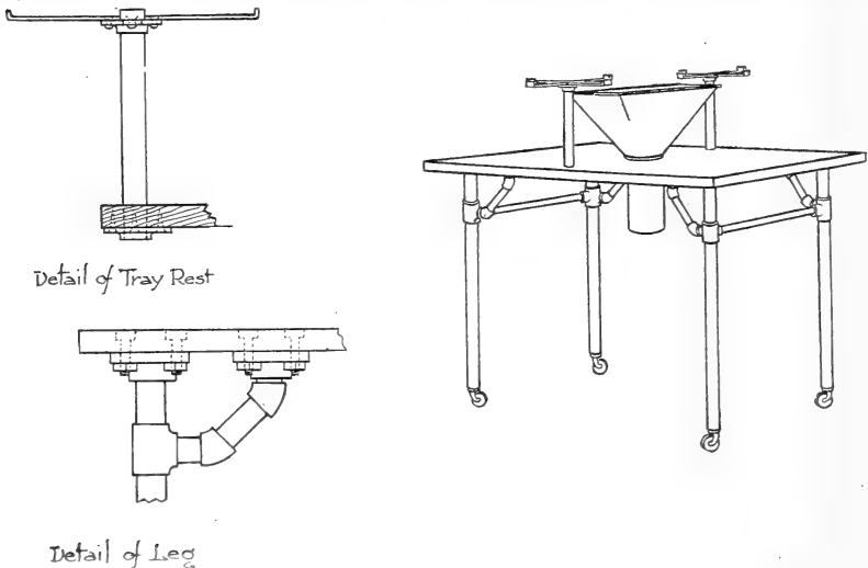
FIG. 11.—Breaking table.
