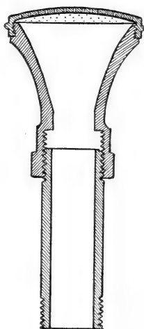
FIG. 23.—Nozzle for rinsing pails and cans (in perspective and cross section).
