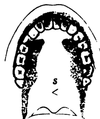
\xi and \zeta Fig. 28a.
