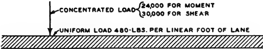
H 15-S12 LOADING
