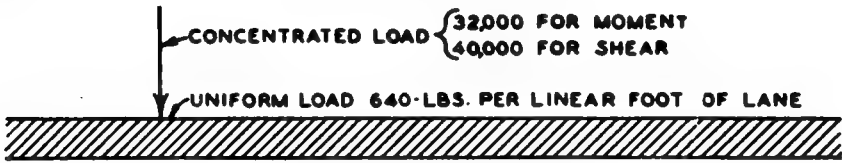
H 20-S16 LOADING
