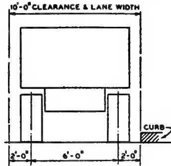
FIGURE 3.—Standard H-8 trucks.
