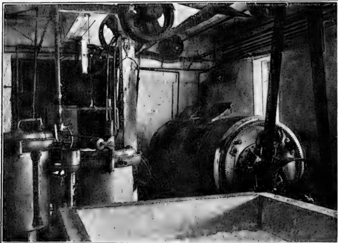
A MODERN CREAMERY. Showing a , pasteurizer with a capacity of 2,500 pounds per hour; b , vat in which cream is ripened 12 to 20 hours after being pasteurized; c , 1,000-pound churn.
