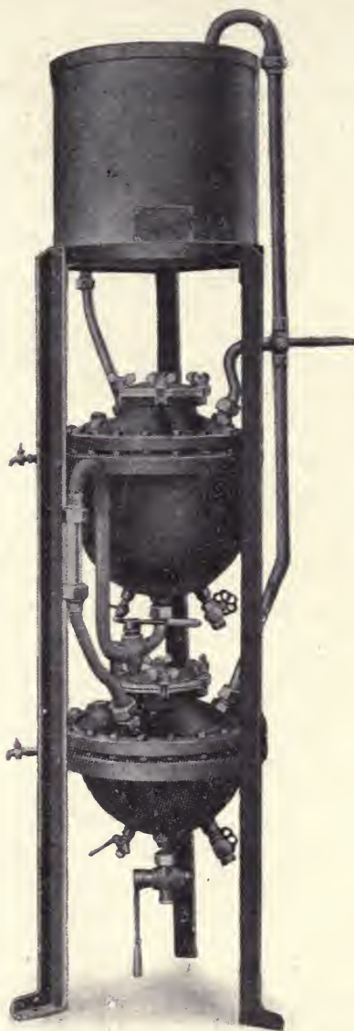
FIG. 109.—EXTRACTION APPARATUS.
