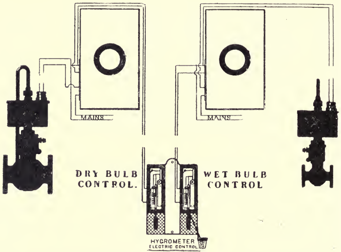
FIG. 137.—“ ISOTHERMAL ” CONTROL OF COTTON-SPINNING ROOMS.
