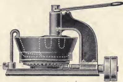
FIG. 18.—ENCLOSED END RUNNER MILL.
