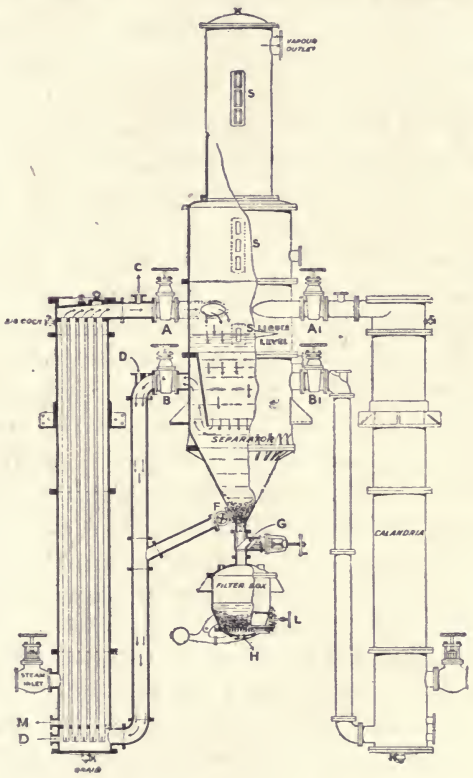
FIG. 101.—KESTNER "SALTING" TYPE EVAPORATOR: SECTION.
