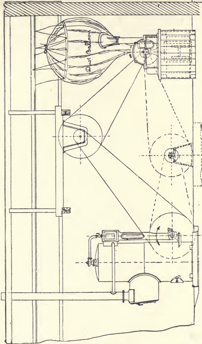
FIG. 15.—G.A. DISINTEGRATOR PLANT: ELEVATION.
