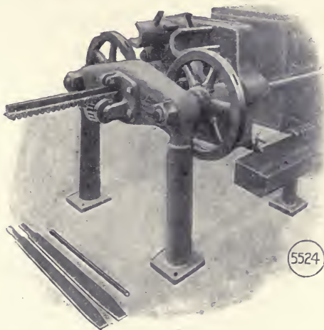
FIG. 61.—FILTER PRESS: RACK AND PINION CLOSING
