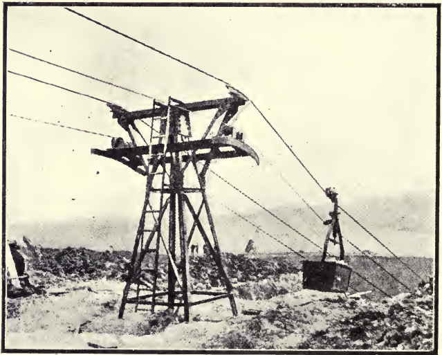
FIG. 150.—STANDARD FOR DOUBLE-ROPE SYSTEM.
