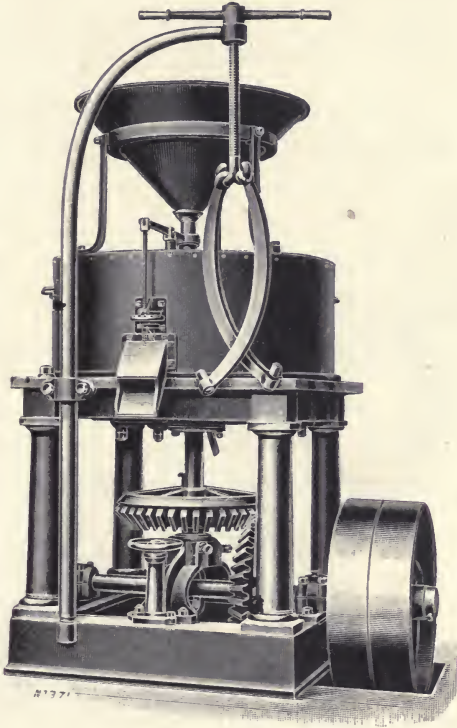
FIG. 16.—MILLSTONE MILL.
