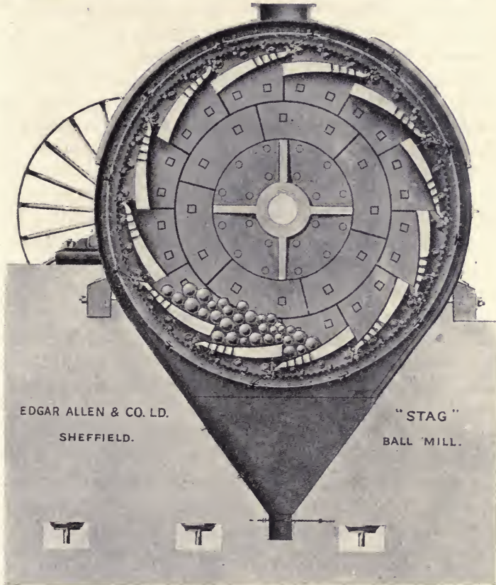
FIG. 22.—“STAG” BALL MILL: SECTION.
