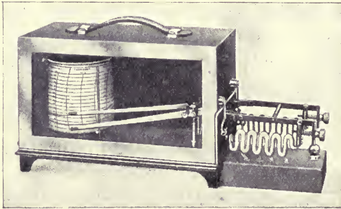
FIG. 78.—RECORDING HYGROMETER.
