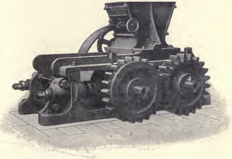
FIG. 5.—FINE CRUSHING ROLLS, TYPE 5, CLASS 1.
