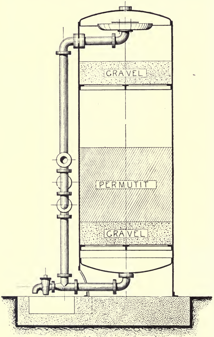
FIG. 127.—PERMUTIT WATER-SOFTENING APPARATUS: DIAGRAM.
