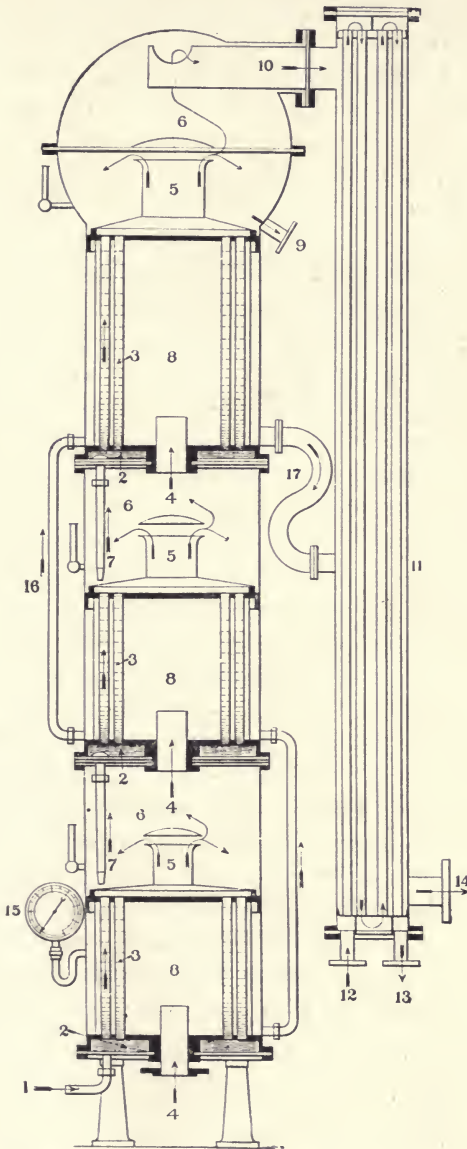
FIG 103.—“MULTIPLEX” TRIPLE-EFFECT EVAPORATOR: SECTION.
