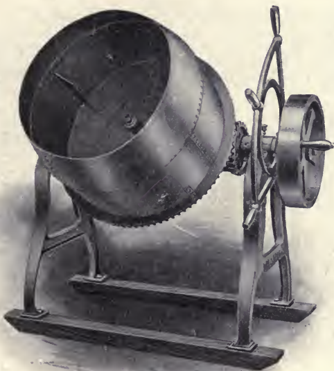
FIG. 48.—“ OPEN-DRUM ” MIXER.
