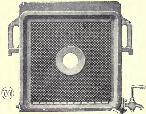
FIG. 55.—FILTER PRESS PLATE: RECESSED TYPE.
