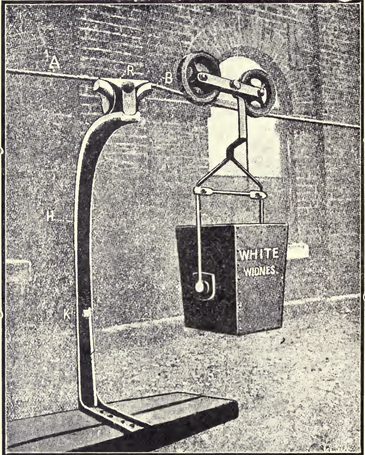
FIG. 148.—INTERWORKS TRAFFIC: PORTABLE ROPEWAY.
