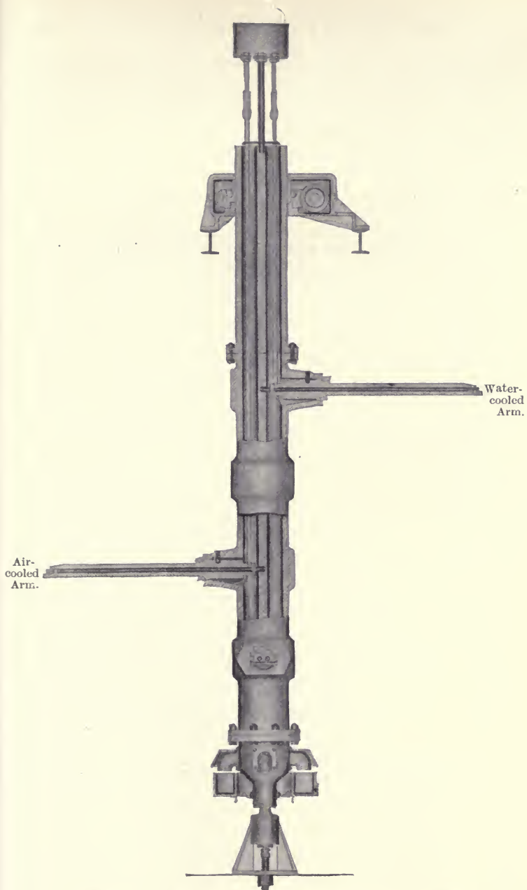
FIG. 121.—"B" TYPE SHAFT FOR ROASTING FURNACE.
