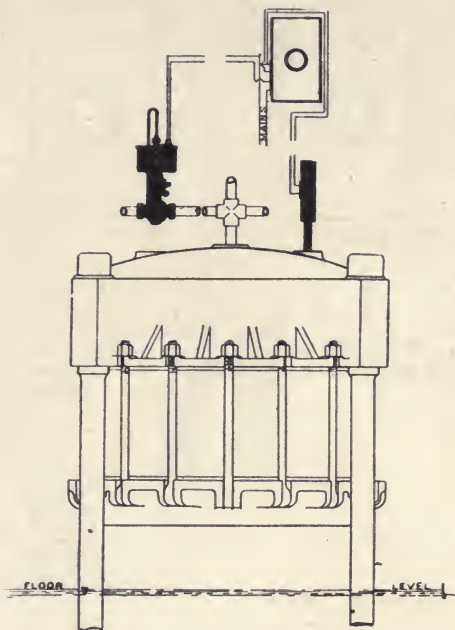
FIG. 135.—“ISOTHERMAL” CONTROL OF VULCANIZING PAN.
