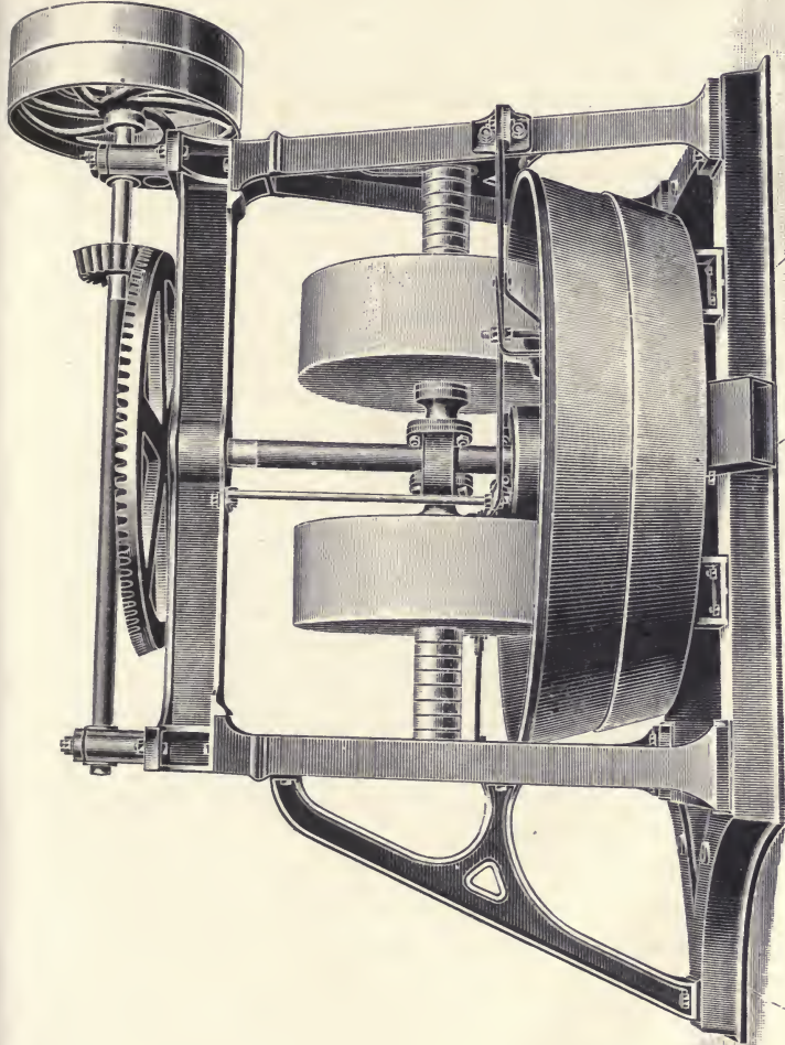
FIG. 10.—MILLS WITH REVOLVING PAN.
