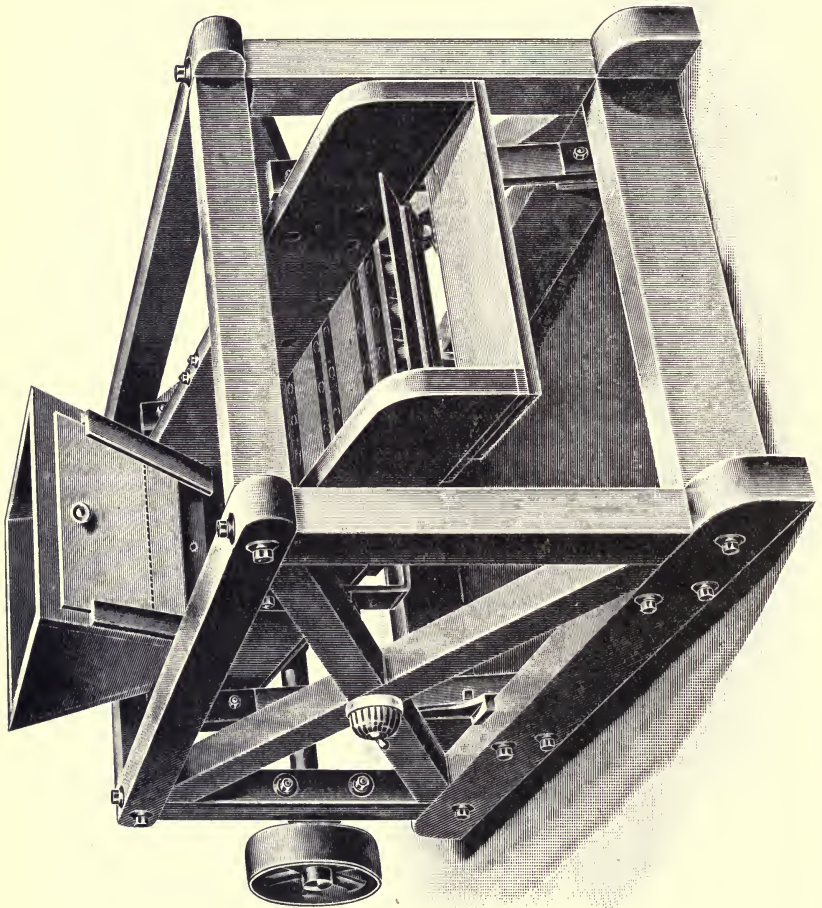
FIG. 36.—ELECTRO-MAGNETIC SEPARATOR.
