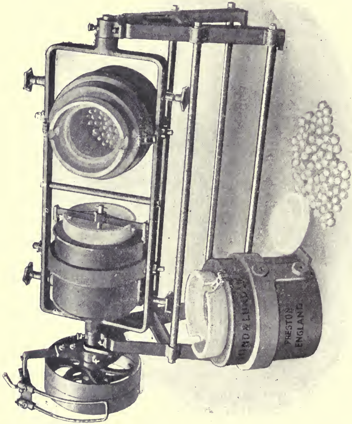
FIG. 20.—BALL GRINDING MILL.
