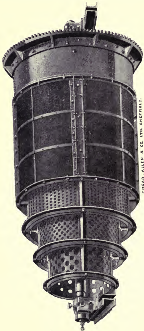
FIG. 26.—TELESCOPIC REVOLVING SCREEN
