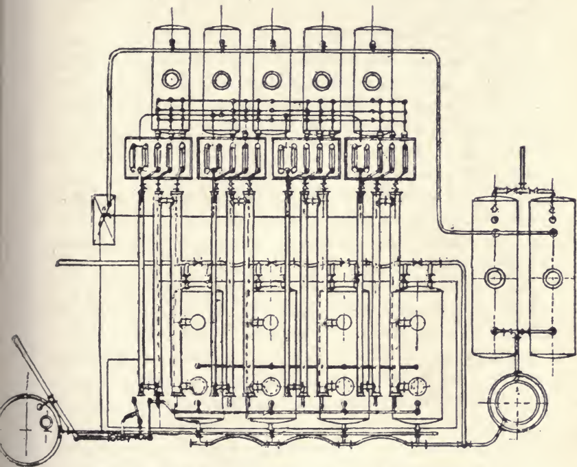
FIG. 112.—LUBRICATING OIL DISTILLING PLANT: PLAN.
