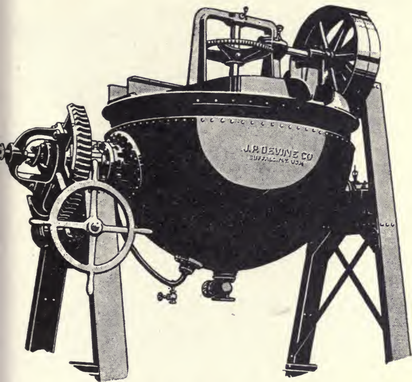
FIG. 89.—TILTING KETTLE.
