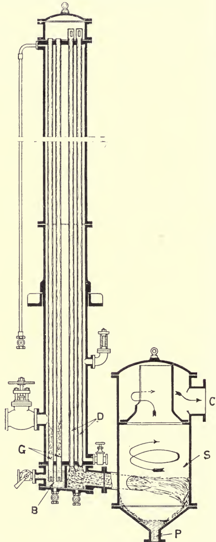
FIG. 99.—KESTNER FALLING FILM SINGLE-EFFECT EVAPORATOR.
