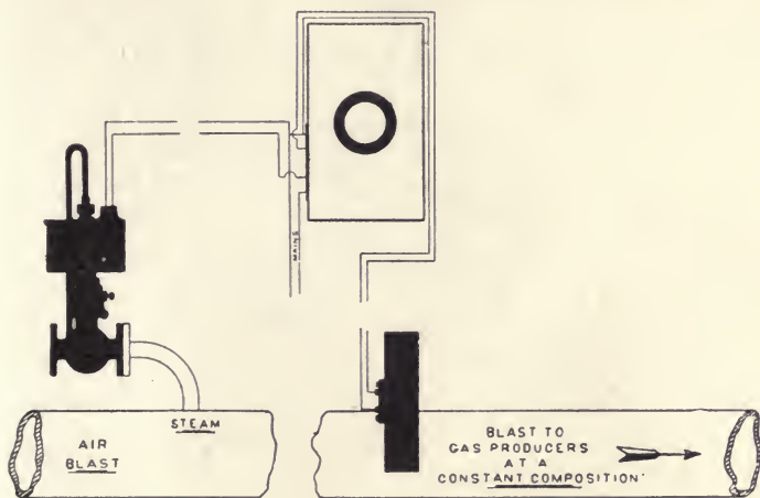
FIG. 136.—“ISOTHERMAL” CONTROL OF BLAST FOR GAS PRODUCER.
