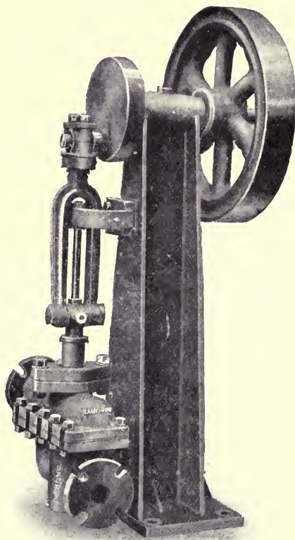
FIG. 166.—TANTIRON VERTICAL PUMP.
