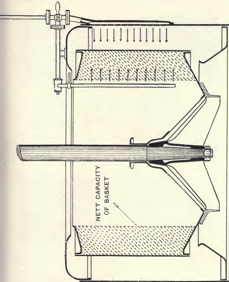
FIG. 64.—“WESTON” CENTRIFUGAL BASKET: SECTION.
