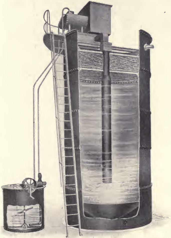
FIG. 126.—CYLINDRICAL WATER-SOFTENING APPARATUS.
