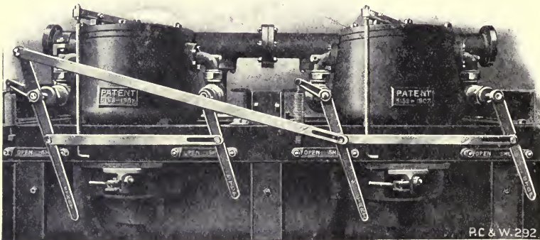
FIG. 71.—INTERLOCKING GEAR FOR WATER-DRIVEN CENTRIFUGAL SECTION.
