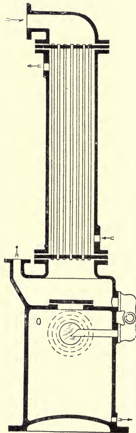
FIG. 97.—SURFACE CONDENSER: SECTION.
