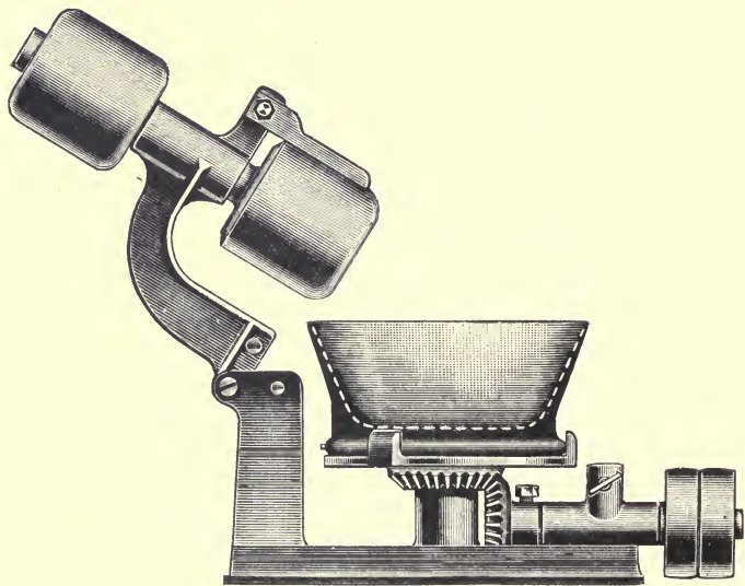
FIG. 17.—VERTICAL RUNNER MILL.
