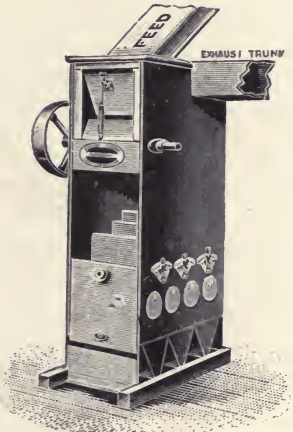
FIG. 33.—GRAVITY OR LEG SEPARATOR.
