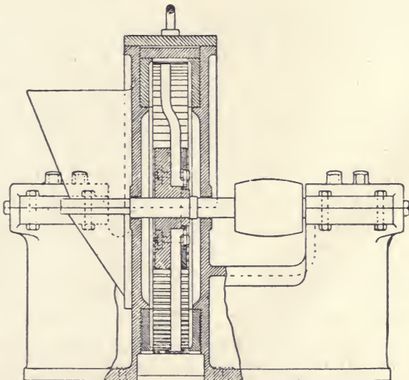
FIG. 13.—DISINTEGRATOR: SECTION.
