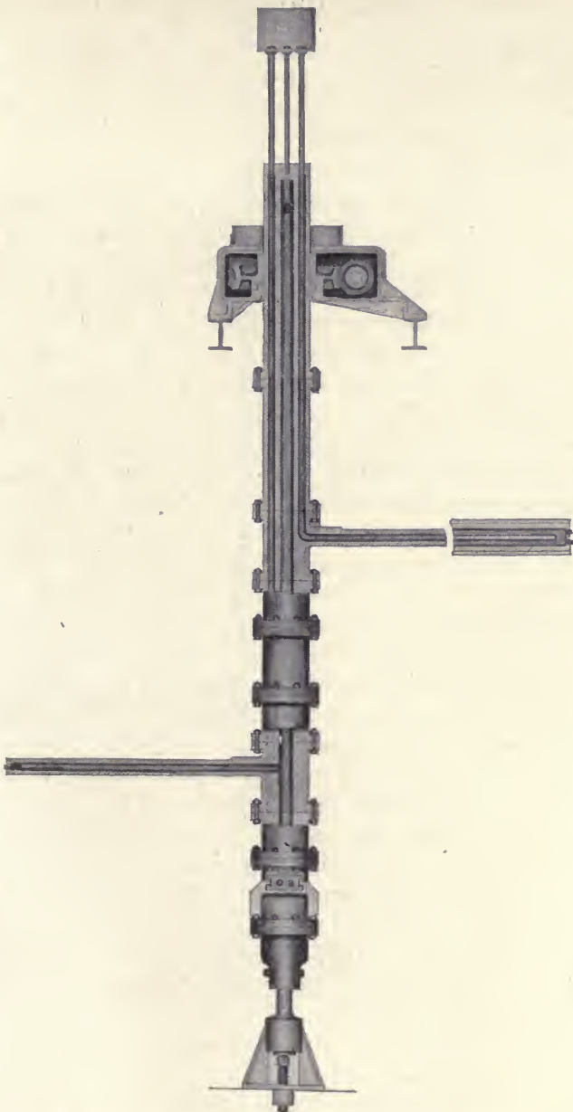
FIG. 120.—“ A ” TYPE SHAFT FOR ROASTING FURNACE.
