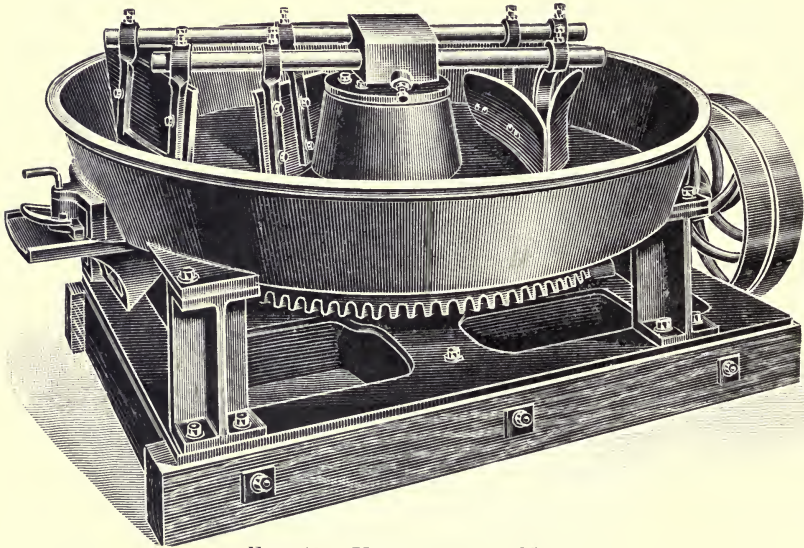
FIG. 49.—UNDER-GEARED MIXER.
