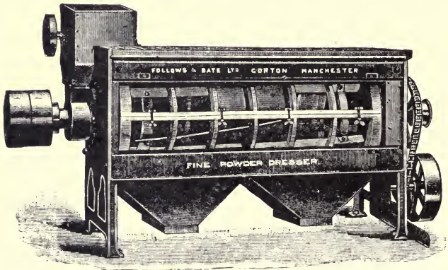
FIG. 29.—POWDER DRESSER.
