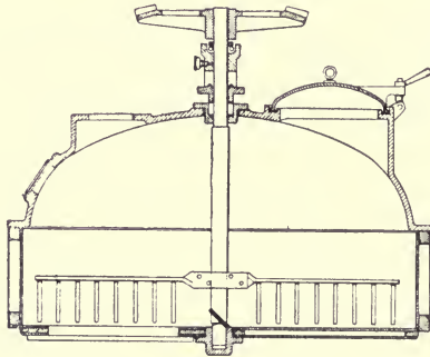
FIG. 84.—VACUUM "JOHNSTONE" DRYER: SECTION.
