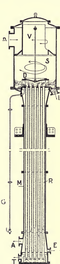
FIG. 98.—KESTNER CLIMBING FILM SINGLE-EFFECT EVAPORATOR.
