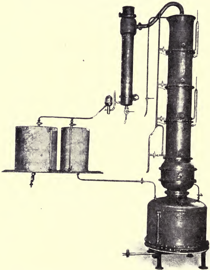
FIG. 105.—RECTIFYING STILL.
