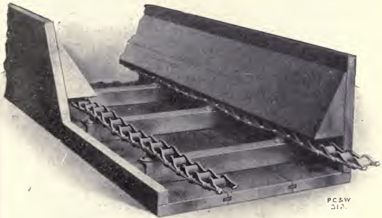
FIG. 158.—SCRAPER CONVEYOR.
