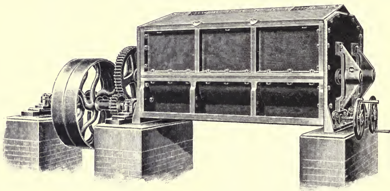
FIG. 47.—DOUBLE MIXER FOR SEMI-LIQUIDS.
