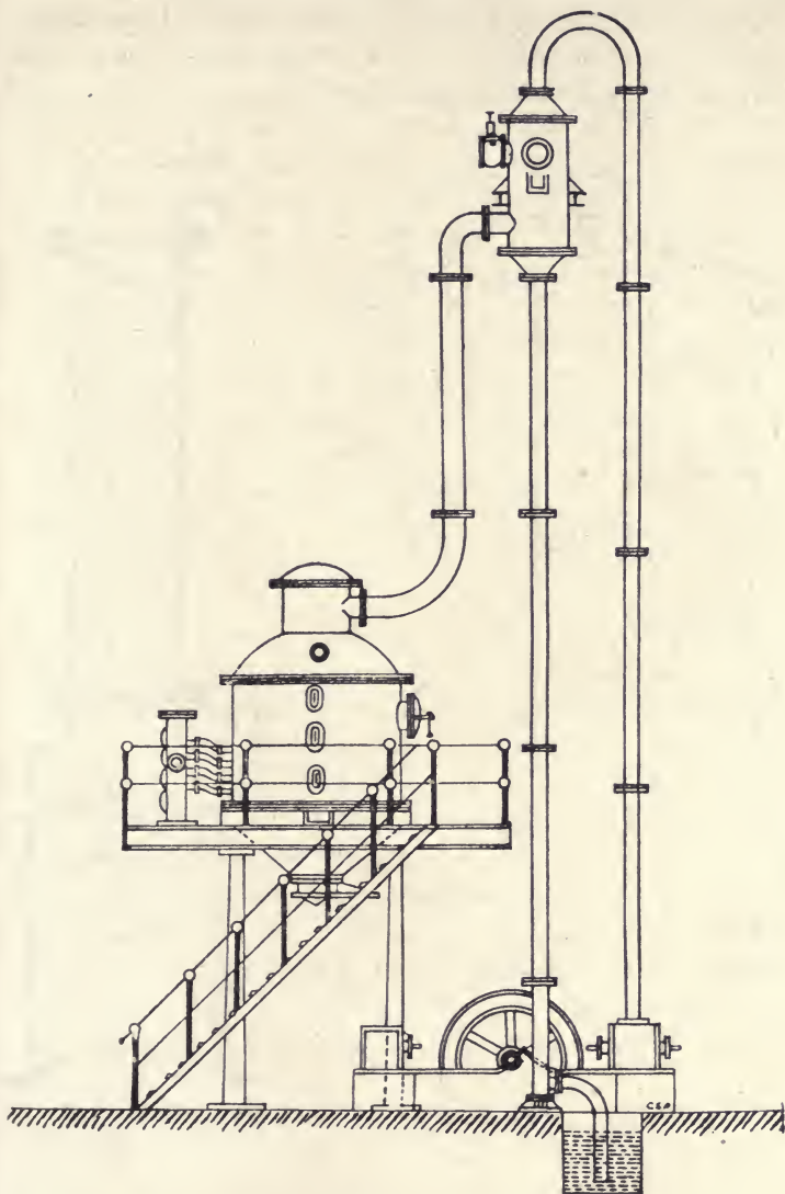
FIG. 95.—G.A. VACUUM PAN: TORRICELLIAN CONDENSER.
