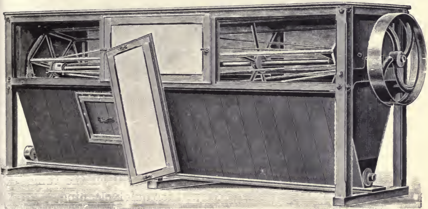
FIG. 28.—SIFTING REELS.
