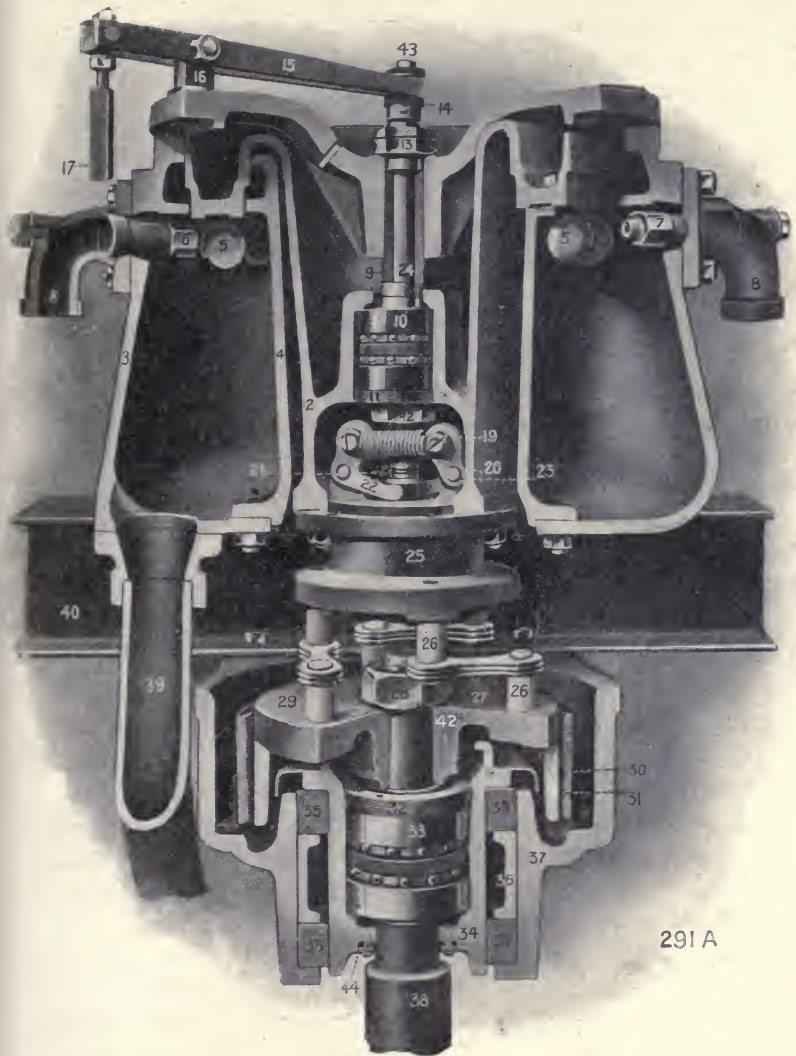
FIG. 70.—“ WESTON ” CENTRIFUGAL MACHINE: WATER-DRIVEN
