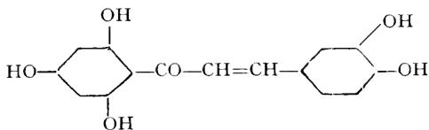
Eriodictyol, C_{15}H_{12}O_6
