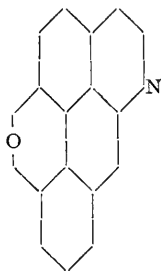
Morphine *
