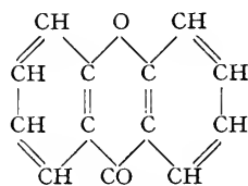
Xanthone
