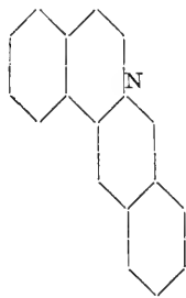
Berberine
