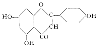
Apigenin
