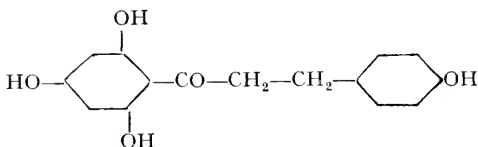
Phloretin
