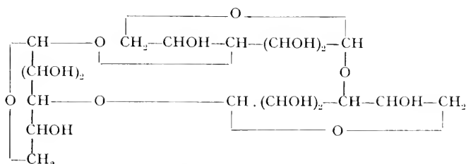
Amylopectin [(C_6H_{10}O_5)_3]_n
