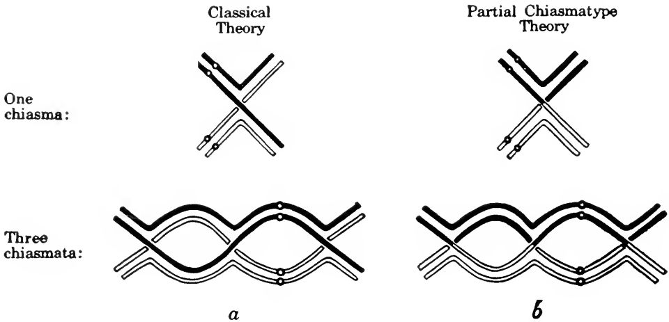
FIG. 64. The interpretation of chiasmata according to the classical theory (a) and the theory of partial chiasmotypy (b).
