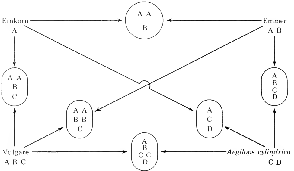
FIG. 135. Diagram showing the relationship between the einkorn , emmer , and vulgare wheats with one another and with Aegilops cylindrica . Illustrated also are the hybrids which would be produced between them. In their haploid stages, the einkorn wheats have genome A, the emmer group A and B, and the vulgare wheats A, B, and C. Aegilops cylindrica has genome C in common with the vulgare wheats and also a fourth genome, D.
