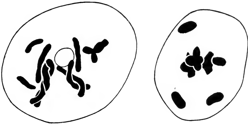
FIG. 134. Chromosomes in a triploid hybrid between Crepis capillaris and C. tectorum . Left , diakinesis showing three bivalents and four univalents. Right , first metaphase showing the same configurations. (Redrawn from Hollingshead in University of California Publications in the Agricultural Sciences .)
