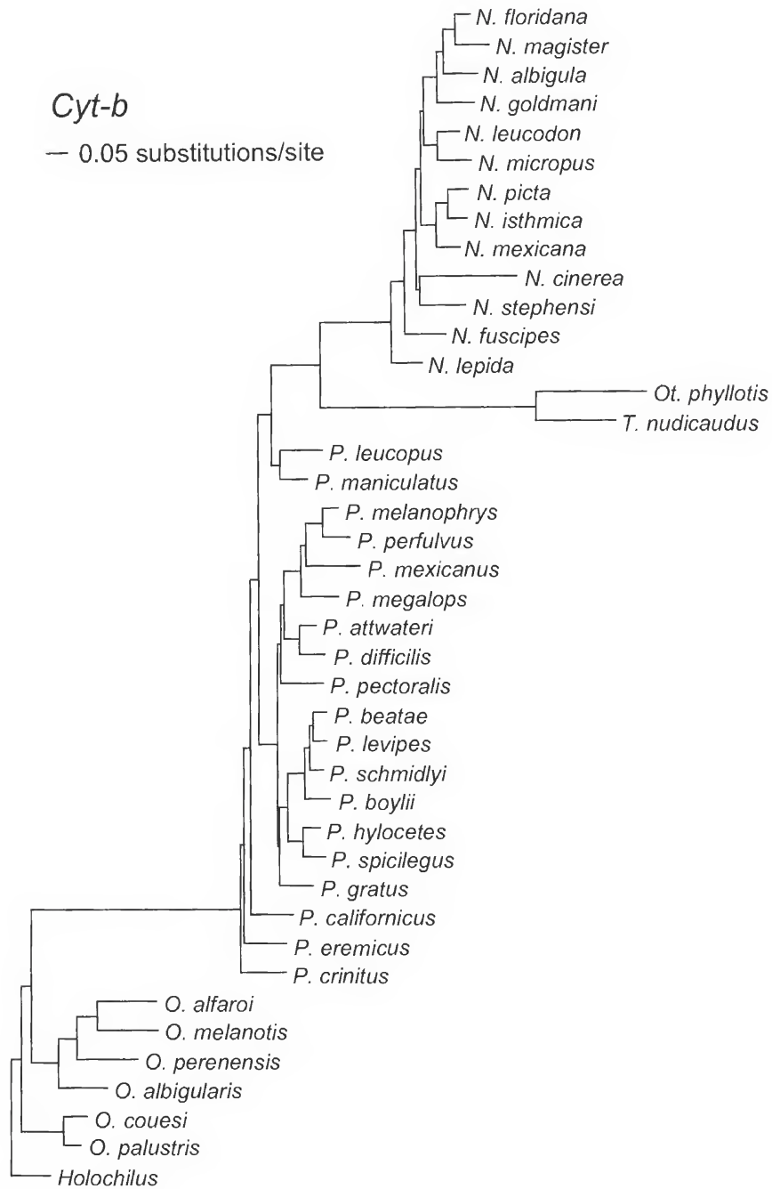
Figure 2. Maximum likelihood phylogram (LnL -14,379.922) from analysis of complete Cyt-b sequences (1,143 base pairs) using best-fit model (GTR + G + I; R_{AC} = 1.310 , R_{AG} = 10.479 , R_{AI} = 2.473 , R_{CG} = 0.708 , R_{CT} = 32.137 , \pi_A = 0.375 , \pi_C = 0.343 , \pi_G = 0.079 , \pi_T = 0.203 , \alpha = 0.687 , p_{mv} = 0.456 ). Holochilus was the designated outgroup. N. = Neotoma . O. = Oryzomys . Ot. = Ototylomys . P. = Peromyscus . T. = Tylomys .
