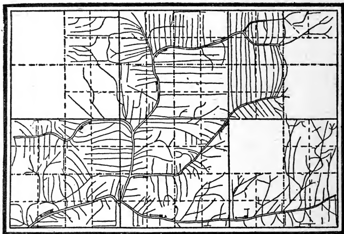
Fig. 151. Plan of drainage of lands of the Illinois Agricultural Company, Rontoul, Illinois. After J. O. Baker. The smallest squares are 40 acres; double lines show open ditches; single lines are tile drains.
