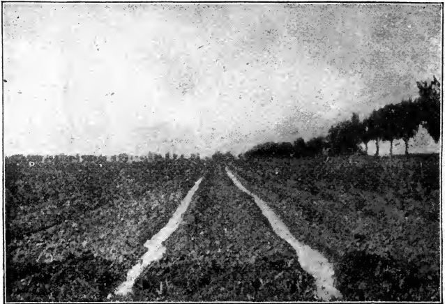
Fig. 94. Irrigating potato rows 40 rods long from head ditch of Fig. 92.
