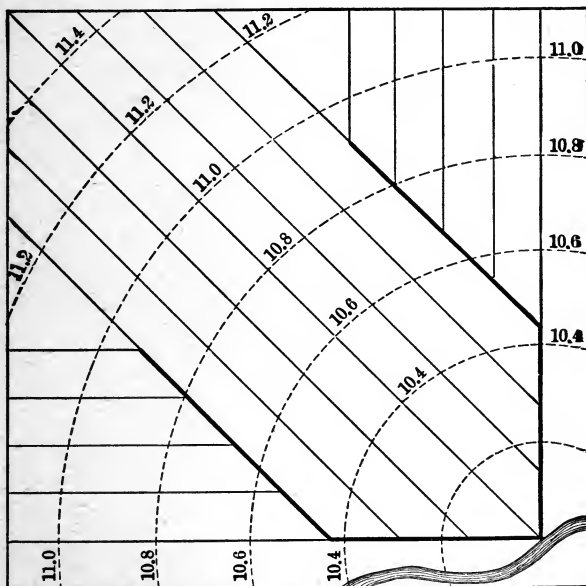
Fig. 156. Arranging drains to secure the maximum fall.
