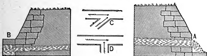
Fig. 142. Proper and improper outlet of drains. A, proper outlet ; B, improper outlet ; C, proper junction of lateral with main ; D, improper junction.
