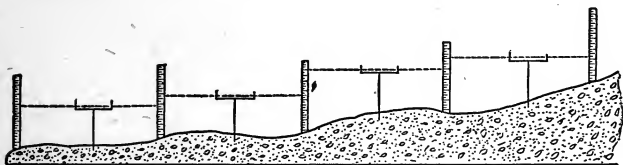
Fig. 154. Method of leveling.
