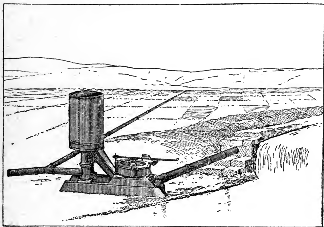
Fig. 69. Hydraulic ramming engine. (Wilson, U. S. Geol. Survey.)
