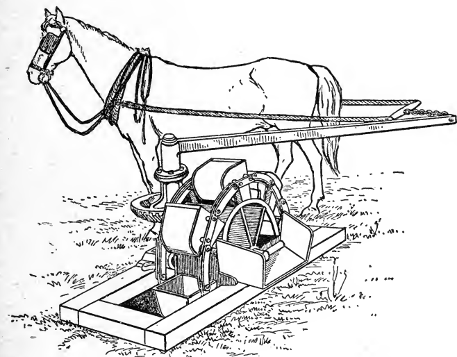
Fig. 79. Bucket pump for use with horse power. (Wilson, U. S. Geol. Survey.)
