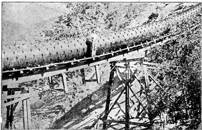
Fig. 59. Pipe line carried on trestle.
