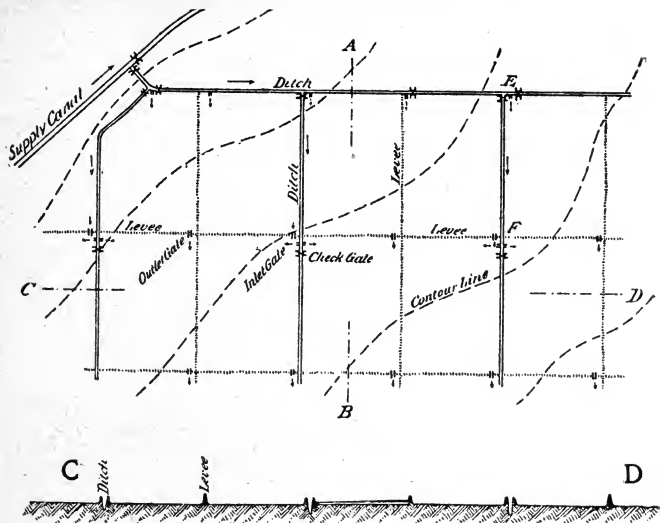
Fig. 87. Flooding field by rectangular checks. (Grunsky.)
