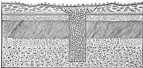
Fig. 149. Method of draining sinks.
