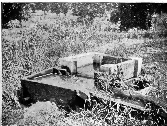
Fig. 62. Cement hydrant, with weir and distributing flume.
