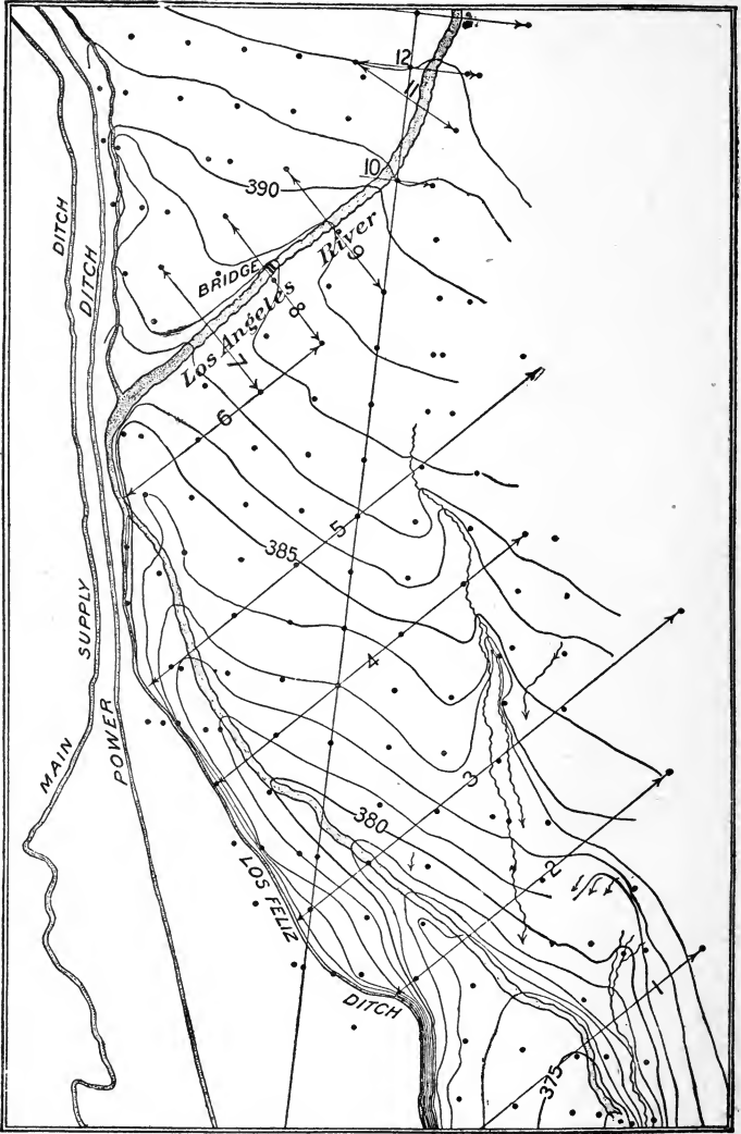
Fig. 135. Contours of ground water in the Los Angeles river valley, California. (U. S. Geol. Survey.)
