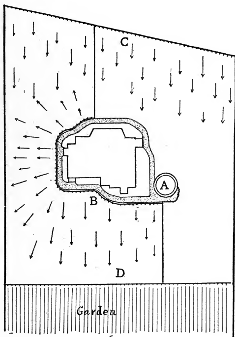
Fig. 122. Plan of lawn and garden irrigation.
