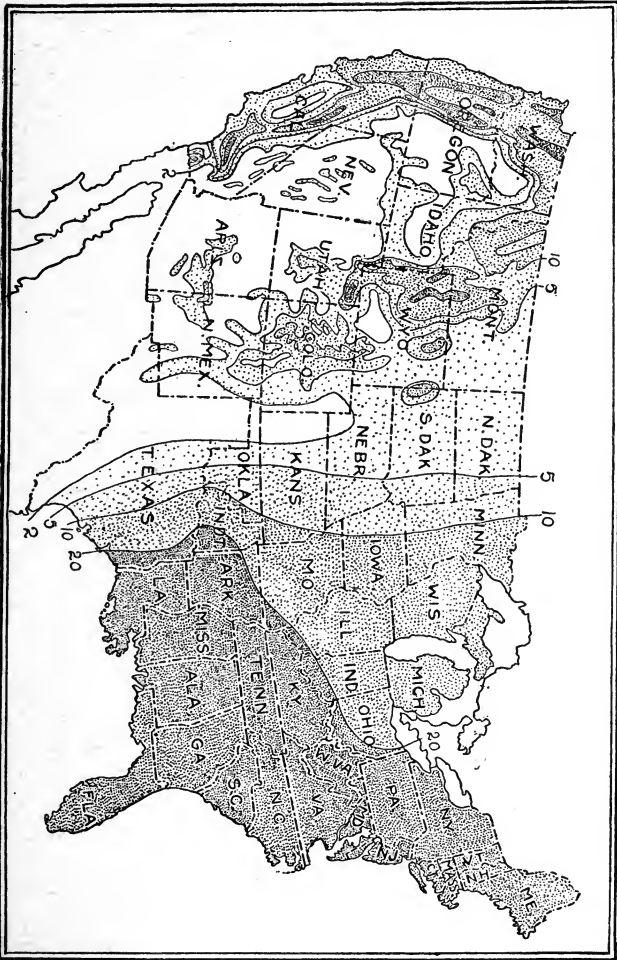
Fig. 22. Mean annual run-off in the United States. (After Newell.)
