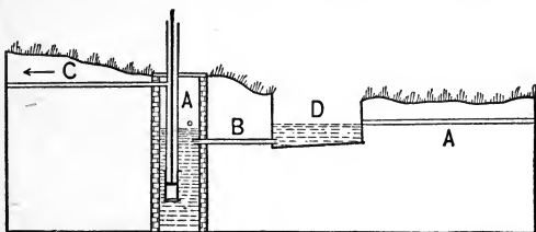
Fig. 150. Method of draining sinks by wind power.
