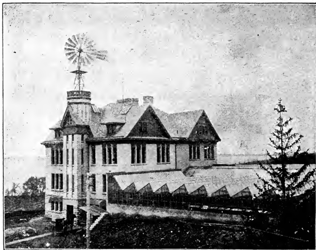
Fig. 71. Exposure of windmill which during one year pumped 79.1 acre-feet of water 12.85 feet high.
