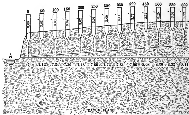
Fig. 157. Determining grade line and depth of ditch.
