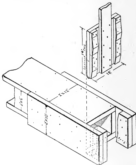
Fig. 75. Sluice and gate for reservoir. (Kansas Agr. Exp. Station.)
