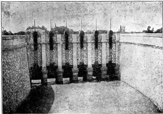
Fig. 48. Head-gate on the Durance above Avignon, France.
