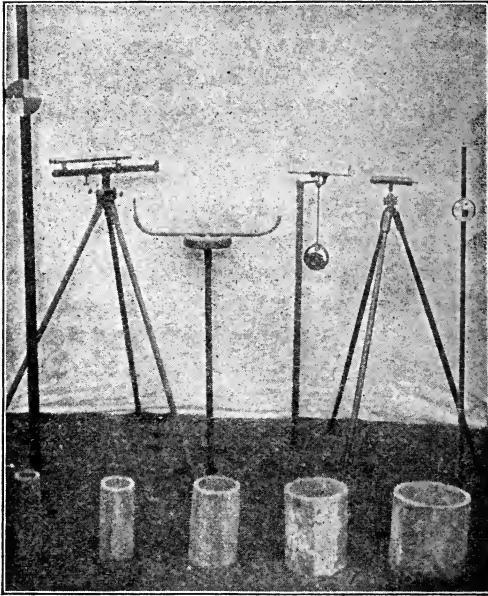
Fig. 153. Four forms of drainage levels, with target-rods.
