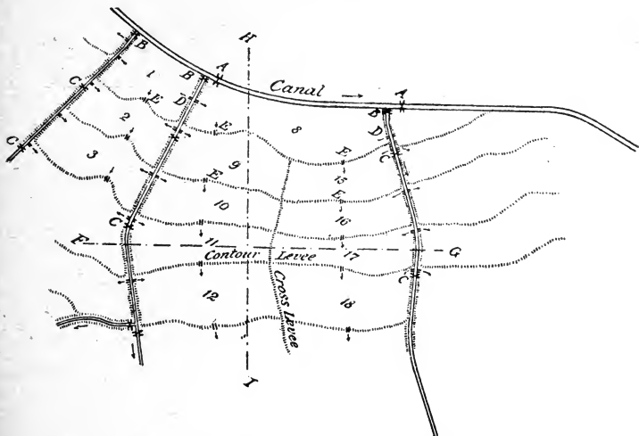
Fig. 88. Flooding field by contour checks. (Grunsky.)
