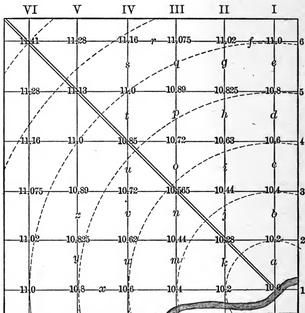
Fig. 155. Leveling for a contour map of field to be drained.
