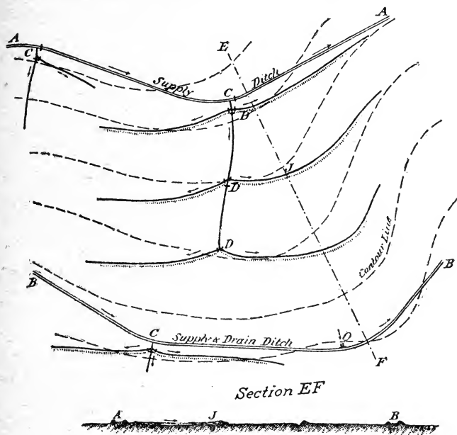
Fig. 86. Flooding field on steep slopes. (Grunsky.)
