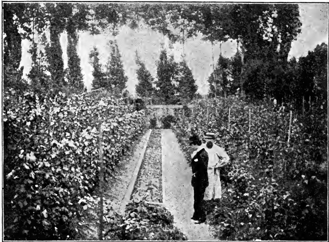
Fig. 126. Sewage irrigation, model garden, Paris.
