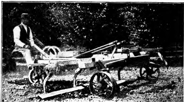
Fig. 110. Three-horse orchard cultivator used at San José, California.
