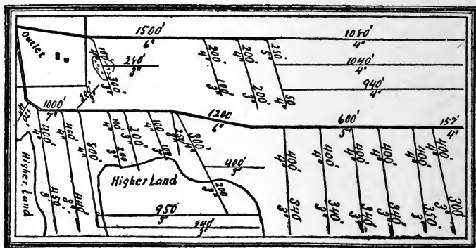
Fig. 141. Drainage system of 80 acres. Double lines represent mains; single lines are laterals. Numbers give length of drains and diameter of tile. After C. G. Elliott.
