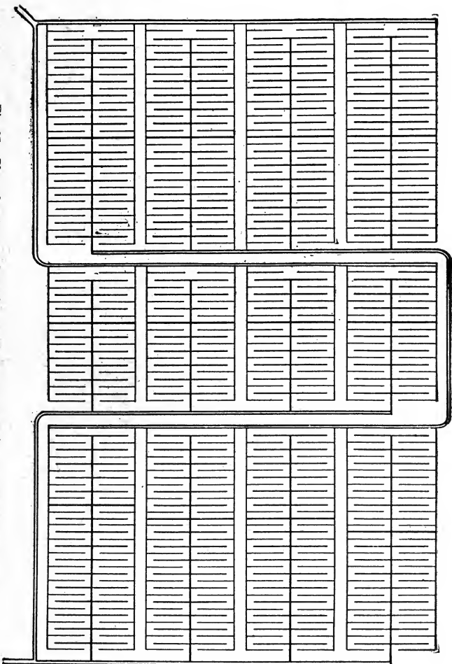
Fig. 97. Plan of water-meadows for using water over again. Neerpelt, Belgium.
