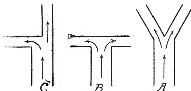
Fig. 43. Branching of canal to divide water equally (A and B) and unequally (C).
