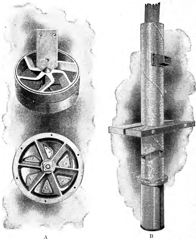
Fig. 73. Aermotor 14-inch reciprocating pump used by windmill. A, pump; B, piston head and suction valve.
