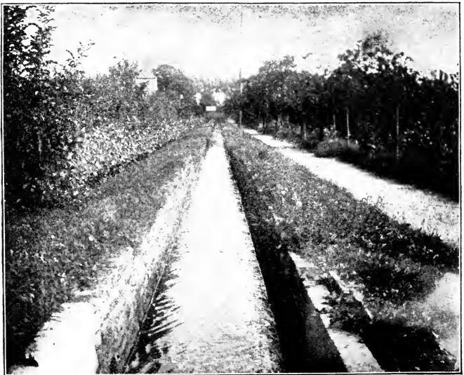
Fig. 128. Stone distributing canal leading from hydrant in Fig. 127.
