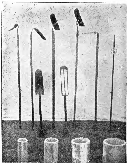
Fig. 158. Some drainage tools.
