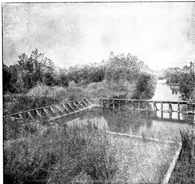
Fig. 56. Waste gate and regulator at head of Kern Island canal, looking across the canal. (Grunsky, U. S. Geol. Survey.)
