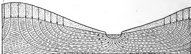
Fig. 134. Diagram of lines of flow of water in the drainage of a river valley.
