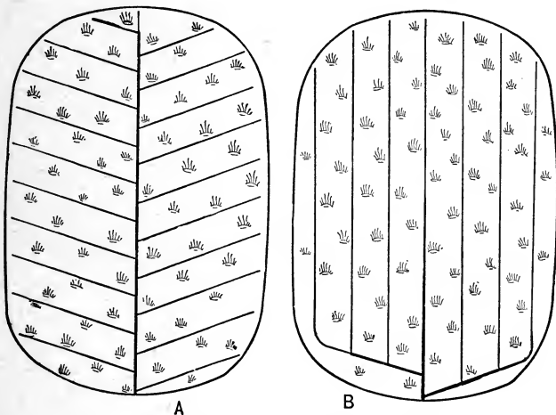
Fig. 145. Two systems of laying out drains.
