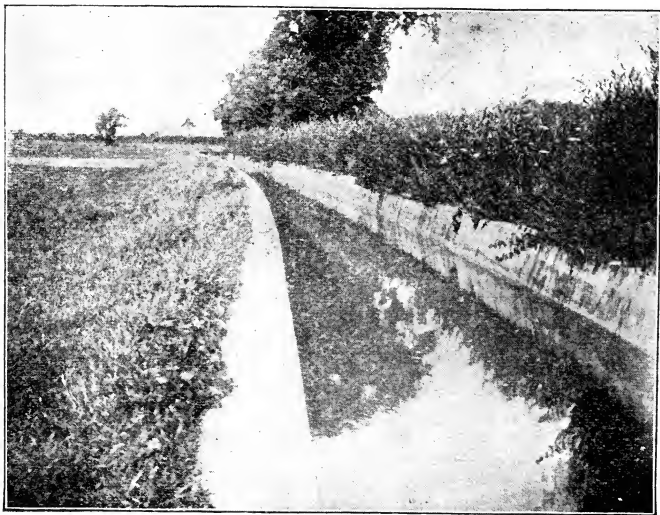
Fig. 130. Cement canal at sewage farm, Croyden, England.
