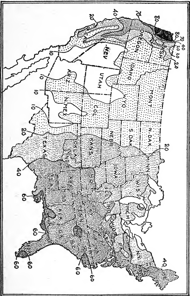
Fig. 23. Mean annual rainfall of the United States. (U. S. Weather Bureau.)
