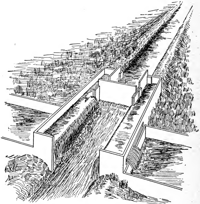
Fig. 45. Spill-back method of dividing water.
