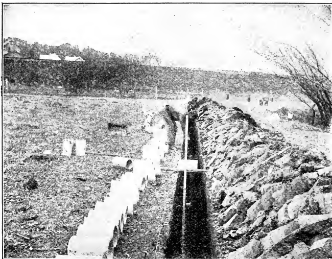
Fig. 161. Bringing the ditch to grade line with tile hoe.
