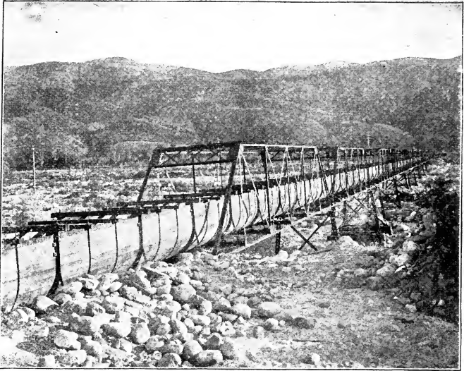
Fig. 60. Redwood stave flume carried across Mill creek wash on trestle.
