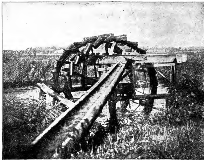
Fig. 15. Wheel for lifting water, at Baiersdorf, Bavaria.
