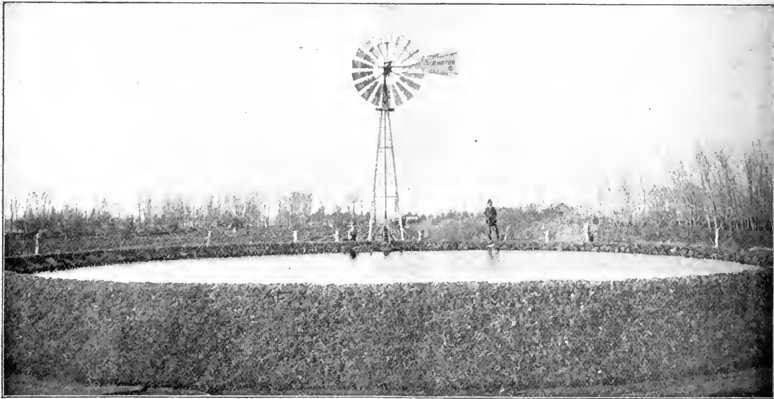
This is a reproduction from a photograph of an irrigating outfit owned by G. M. Davidson, Larned, Kan. It consists of a 12 foot pumping Aermotor on a 30 foot steel tower with an 8 inch irrigation pump. The mill is never turned off and irrigates perfectly 10 acres of ground, which is kept thoroughly soaked. The reservoir is 60 feet in diameter, 5½ feet high and the pump fills it in 10 hours.
