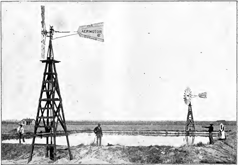
Photographic reproduction of a windmill irrigating plant owned by T. J. Dyke, Garden City, Kan. It consists of two 12 foot Aermotors with 10 inch pumps upon 12 inch strokes. The reservoir is 100x150 feet and 4 feet deep. The water is raised 15 feet. The amount of land irrigated is 28 acres.
