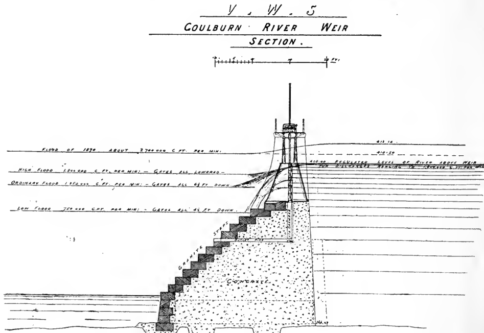
SECTION OF GOULBURN WEIR. (From drawing made especially for THE IRRIGATION AGE.)
