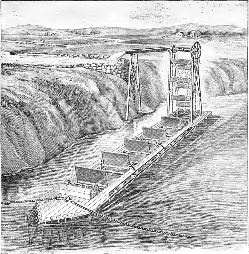
AUSTIN CURRENT MOTOR.
