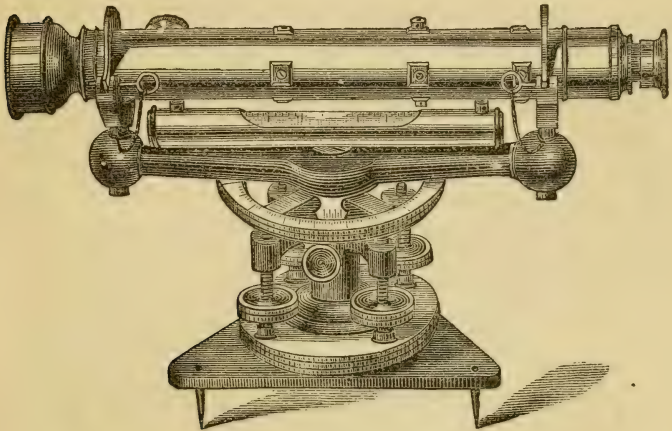
Fig. 84.—GURLEY'S LEVEL.
