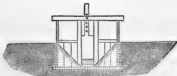
Fig. 60.—WATER GATE.
