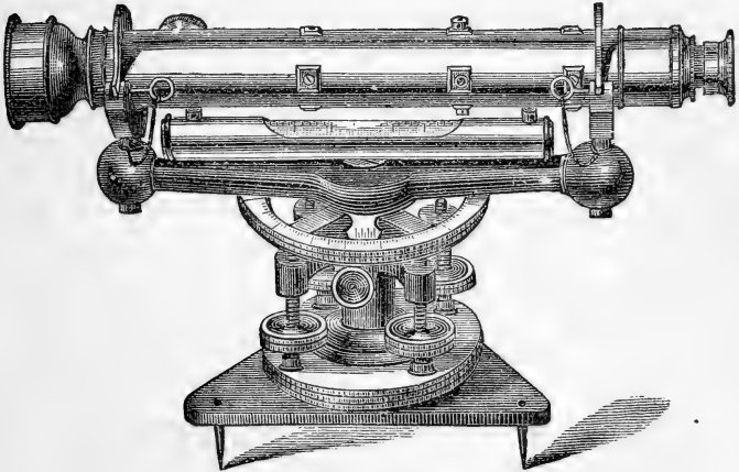
Fig. 84.—GURLEY'S LEVEL.
