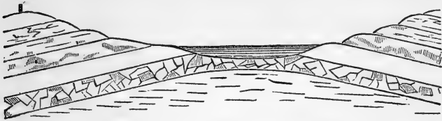
Fig. 112.—AN ANTICLINAL VALLEY.
