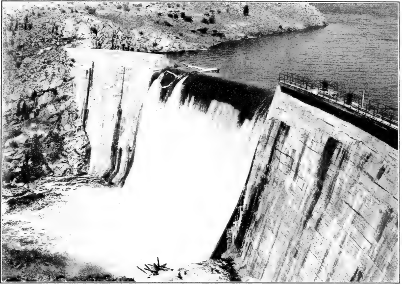
FIG. 1.—HALLIGAN DAM OF THE NORTH POUDBRE SYSTEM. DEPTH OF 1½ FEET ON THE SPILLWAY.
