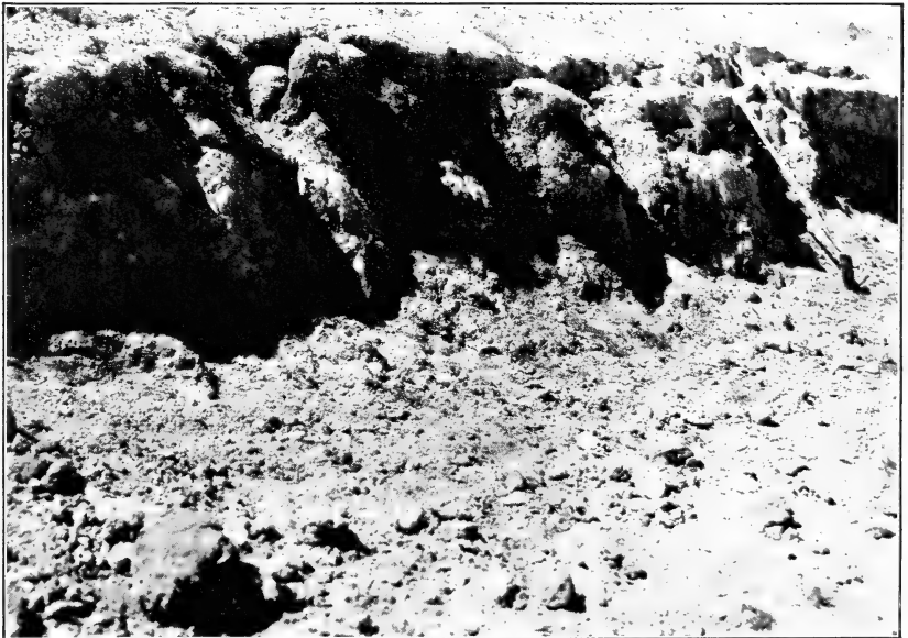
FIG. 2.—EFFECT OF WAVE ACTION ON THE INNER SLOPE OF THE DAM OF NORTH POUDBRE RESERVOIR No. 15.
