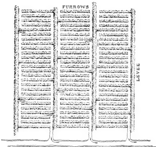
FIG. 4.—Combined check and furrow irrigation.
