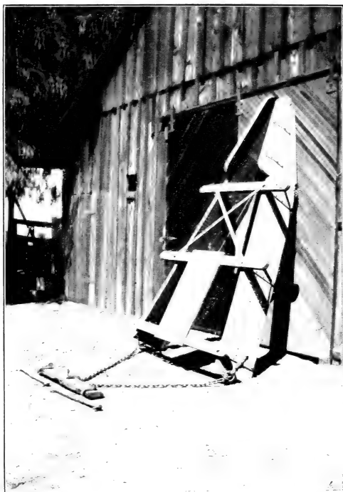
FIG. 1.—THE "RIDGER" FOR LEVEE MAKING IN THE CHECK SYSTEM.
