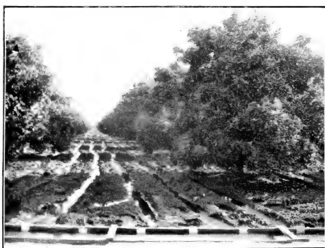
FIG. 2.—BOARD FLUME AND FURROW IRRIGATION AT FULLERTON, CAL.
