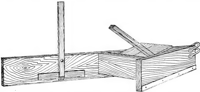
FIG. 2.—"Crowder" used in the preparation for distribution of water in the check system.
