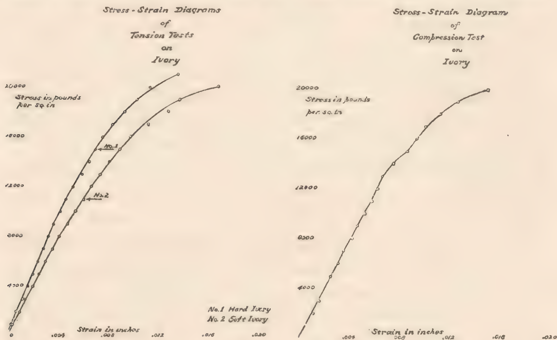
TENSION AND COMPRESSION TESTS
