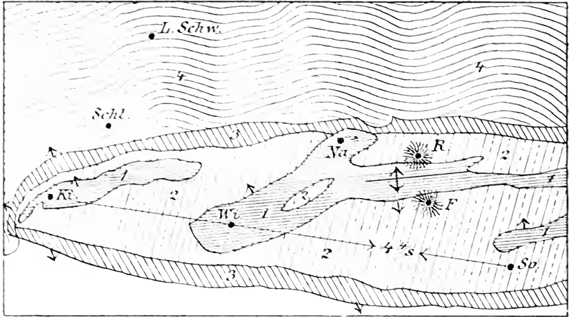
1. Sericit-Gneiss. 2. Sericit-Schiefer. 3. Phyllit. 4. Tannus-Quarzit.
