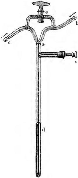
ALTMANN'S Thermoregulator.
