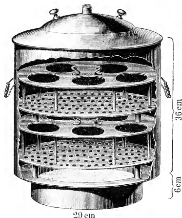
M. KIRCHNER'S Sputum-Desinfectionsapparat.
