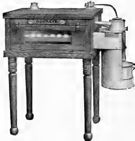
Buckeye Standard 60 Egg This incubator bears the underwriter's label. Complete, ready for use, $10.00 Weight. Crated ready for shipment, 85 pounds.
