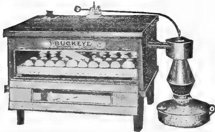
Style C Buckeye 50-Egg Incubators Single Walls Throughout. Complete Ready to Use, $6.00
