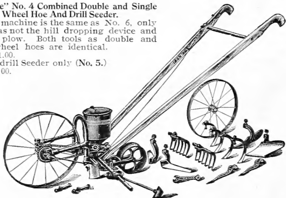
No. 40, No. 4 Combined Drill Seeder (Side hoes and teeth only.) Price $9.50.
