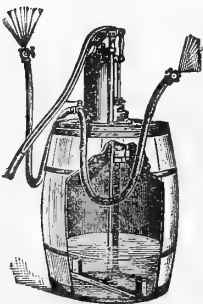
EMPIRE KING PUMP WITH AGITATOR.
