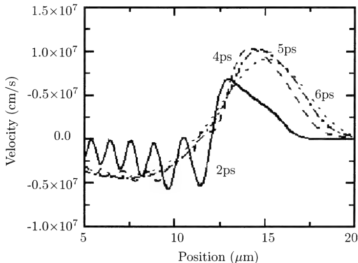
Figure 4. Ion velocity profiles at times 2, 4, 5 and 6 ps taken from genuine two fluids computations for a 3 \times 10^{15} W cm ^{-2} 4 ps rectangular laser pulse irradiating a deuterium plasma ramp of 20 \mu\text{m} thickness with critical density at 12 \mu\text{m} , confirming the generation of an ablating plasma block (negative velocity) and a compressing plasma block (positive velocity).
