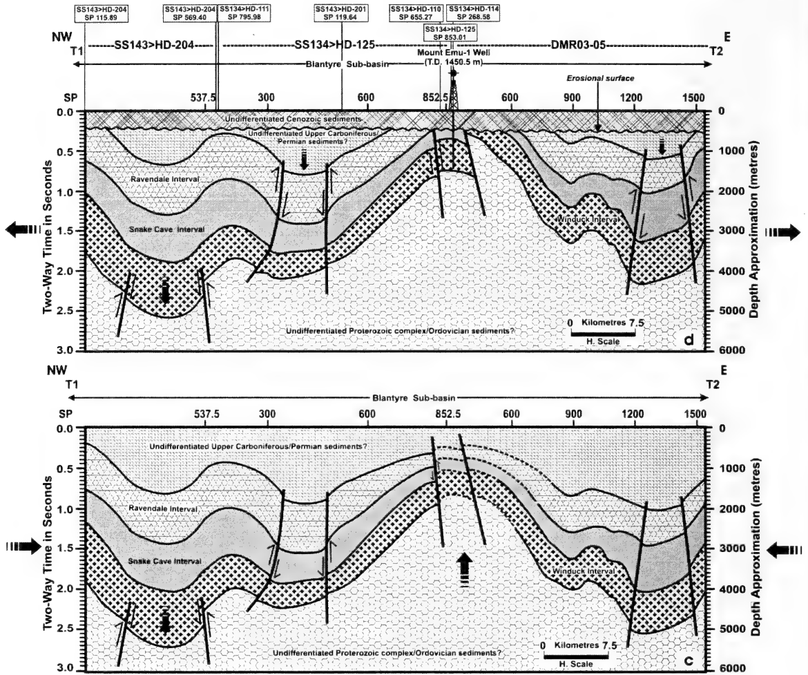
Figure 11 c & d. Cross-section T1-T2, showing the tectonic development of the Blantyre Sub-basin (See location of cross-section in Figure 2). (c) More compression, showing further anticlinal folding associated with the Mount Emu structure to create complex reverse faults (d) Further development of the Mount Emu thrust fault, followed by extension, erosion and deposition of the Cenozoic sediments.
