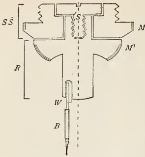
Fig. 11. The marker consists of the part SS with the milled edge (M). This part bears the Society or objective screw for attaching the marker to the microscope. R. Rotating part of the marker. This bears the eccentric brush (B) at its lower end. This brush is on a wire (W). This wire is eccentric, and may be made more or less so by bending the wire. The central dotted line coincides with the axis of the microscope. The revolving part is connected with the "Society Screw" by the small screw (S).
