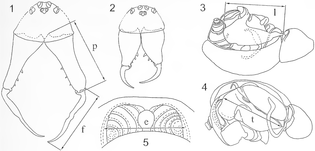
Figures 1–5.— Linyphia triangularis , illustrations of some of the characters measured. 1, 2. Frontal views of large male and medium size female, drawn at same scale. 3, 4. Left genital bulb, proteral (3) and retrolateral (4) views. 5. Epigynum, posterior view. e = epigynum width, f = fang length, l = bulbal lamina length, p = paturon length, t = tegulum length.
