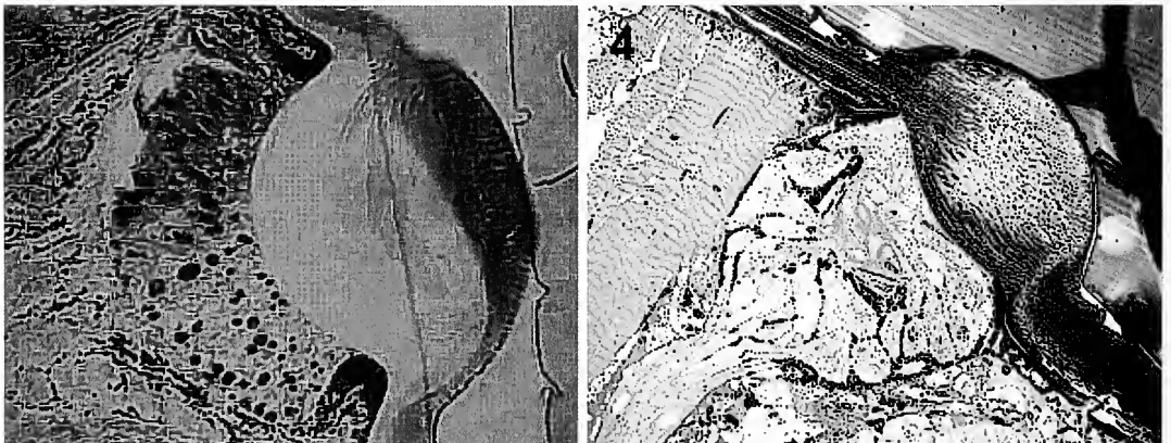
Figures 3—4.—3. Primary eye of B. insignis ; 4. Secondary eye of B. insignis .
