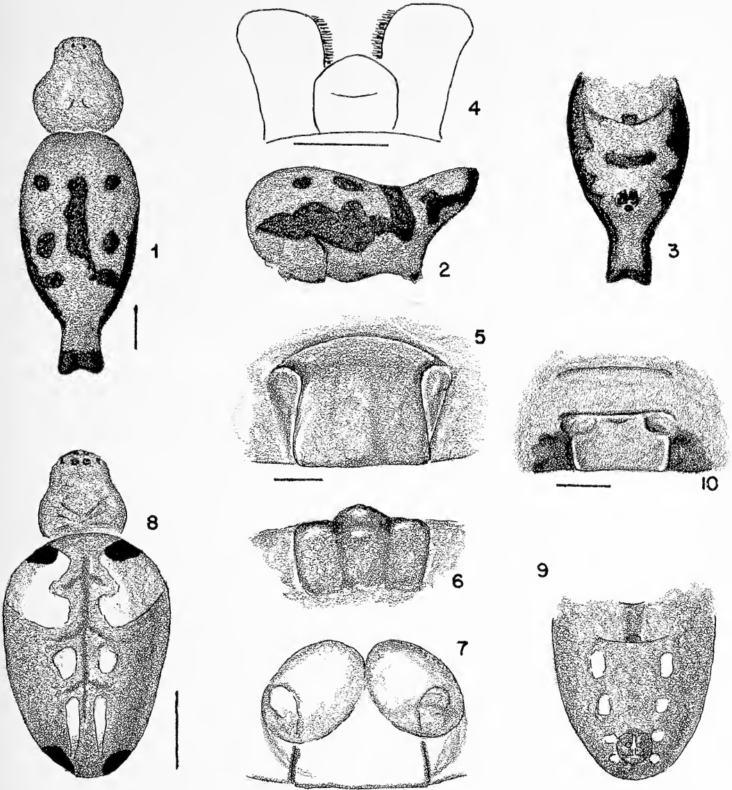
Figures 1-10.— Alcimosphenus licinus Simon. 1. Carapace and abdomen, dorsal; 2. Abdomen, lateral; 3. Abdomen, ventral; 4. Labium and endites; 5-7. Epigynum; 5. Ventral; 6. Posterior; 7. Ventral, cleared. 8-10. Leucauge rubripleurus (Mello-Leitão). 8. Carapace and abdomen, dorsal; 9. Abdomen, ventral; 10. Epigynum, ventral. Scale lines, 1.0 mm; of genitalia 0.1 mm; Fig. 4 = 0.5 mm.
