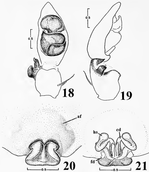
Figures 18–21.—Genitalia of Paratrechalea ornata . 18, 19. right palpus; 18. ventral view, 19. retrolateral view; 20, 21. female genitalia; 20. ventral view, 21. dorsal view. af = anterior genital field, cd = copulatory duct, fd = fertilization duct, hs = head of spermathecum.
