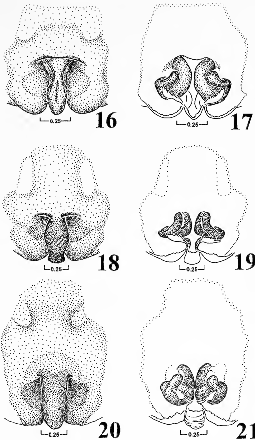
Figures 16–21.—Female genitalia of Hesydrus species. 16, 17. H. caripito ; 16, ventral view, 17, dorsal view; 18, 19. H. yacuiba ; 18, ventral view, 19, dorsal view; 20, 21. H. chanchamayo ; 20, ventral view, 21, dorsal view.
