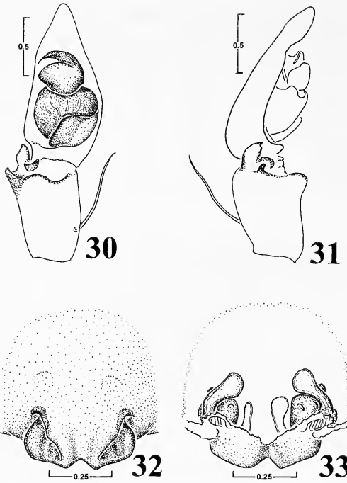
Figures 30–33.—Genitalia of Paratrechalea saopaulo . 30, 31. right palpus; 30. ventral view, 31. retrolateral view; 32, 33. female genitalia; 32. ventral view, 33. dorsal view.
