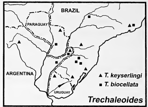
Figure 3.—Distribution of species of Trechaleoides .
