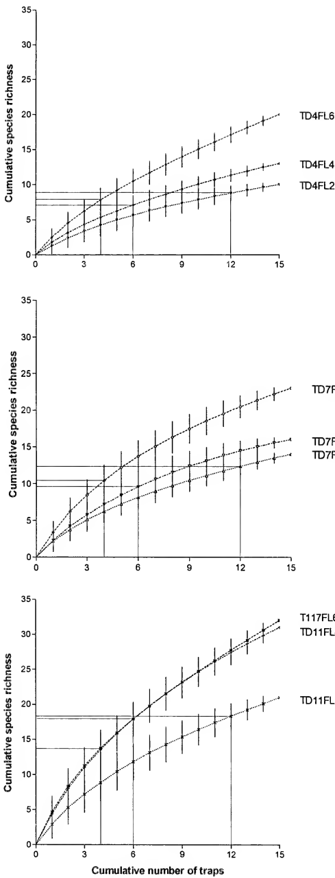
Figure 15.—Smoothed species accumulation curves showing the number of species likely to be sampled with standardized cumulative fence length of 24 m for all trap sizes of fenced traps. Error bars are \pm one standard deviation of the mean. TD4 denotes trap diameter 4.3 cm, TD7 denotes trap diameter 7.0 cm, TD11 denotes trap diameter 11.1 cm, FL2 denotes 2 m fence, FL4 denotes 4 m fence, FL6 denotes 6 m fence. Curves are spread over three graphs for the purpose of clarity.
