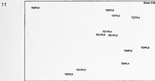
Figures 10–11.—Ordinations showing similarity in spider community composition between each fence length/trap size combination at (10) species and (11) family ranks. TD4 denotes trap diameter 4.3 cm, TD7 denotes trap diameter 7.0 cm, TD11 denotes trap diameter 11.1 cm, FL0 denotes no fence, FL2 denotes 2 m fence, FL4 denotes 4 m fence, FL6 denotes 6 m fence.
