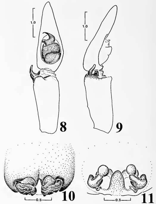
Figures 8–11.—Genitalia of Trechaleoides biocellata . 8, 9. right palpus; 8. ventral view, 9. retro-lateral view; 10, 11. female genitalia; 10. ventral view, 11. dorsal view.
