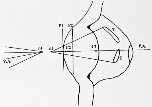
Figure 2.—Diagrammatic section of the secondary eye of B. insignis . n_1 = front nodal point; n_2 = rear nodal point; C_1 = center of curvature of front of lens; C_2 = center of curvature of the rear of lens; P_1 = front principal plane; P_2 = rear principal plane; P.A. = principal axis; T = tapetum; V.A. = visual axis.
