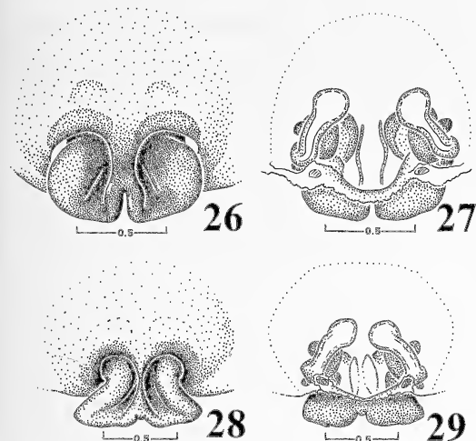
Figures 26-29.—Female genitalia of Paratrechalea species. 26, 27. P. galianoae ; 26. ventral view, 27. dorsal view; 28, 29. P. azul ; 28. ventral view, 29. dorsal view.
