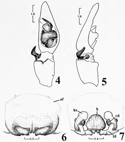
Figures 4–7.—Genitalia of Trechaleoides keyserlingi . 4, 5. right palpus; 4. ventral view, 5. retrolateral view; 6, 7. female genitalia; 6. ventral view, 7. dorsal view. af = anterior field, cd = copulatory duct, fd = fertilization duct, h = hood, hs = head of spermathecum, mf = middle field.
