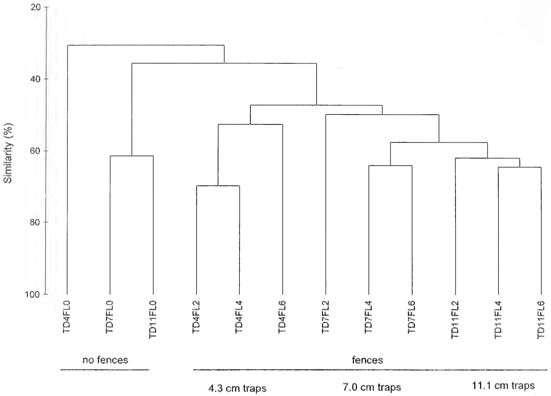
Figure 12.—Dendrogram for hierarchical clustering (group-average linking) of similarity in spider species composition between each fence length/trap size combination.
