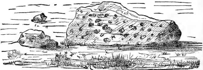
Erratic blocks near Thrapp.
