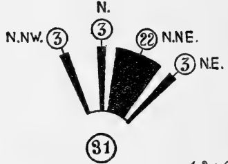
Fig. 4. Diagram showing wind directions and frequencies during October-December 1944
