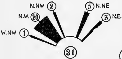
Fig. 4. Diagram showing wind directions and frequencies during October-December 1944
