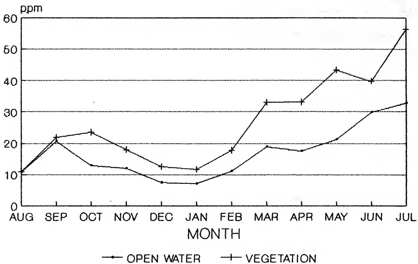
Fig. 5. Average CO 2 in macrohabitats during 1985-86.
