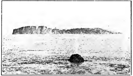
Fig 12.—The Inoko-jima rock in foreground and Shin-jima S in distance—the two new islets of 1779-1780. (After Yamaguchi.)
