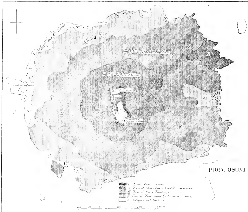
Fig. 7.—Sketch-map illustrating vegetable zones.
