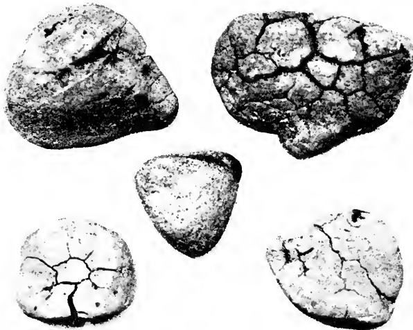
Fig. 41.—Various forms of lava scoria. Natural size. Loc.: Yokoyama.
