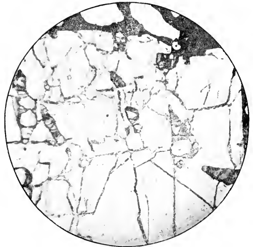
Fig. 44.—Feldspar-phenocryst in the eastern lava-field at Ycbino-tsuka. \times 18 .
