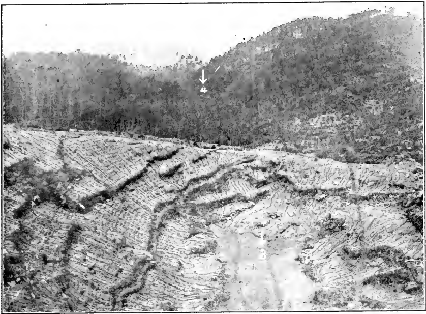
Fig. 35.—Vents No. 3 and 4 in the same lava-field as in Text-fig. 34.
