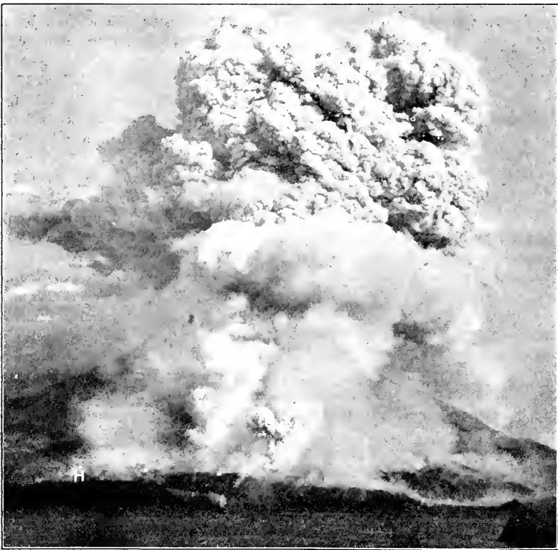
Fig. 20.—Lava-stream reaching the shore, on January 15th, as seen from the quay at Kagoshima. H—Hakamagoshi hill.
