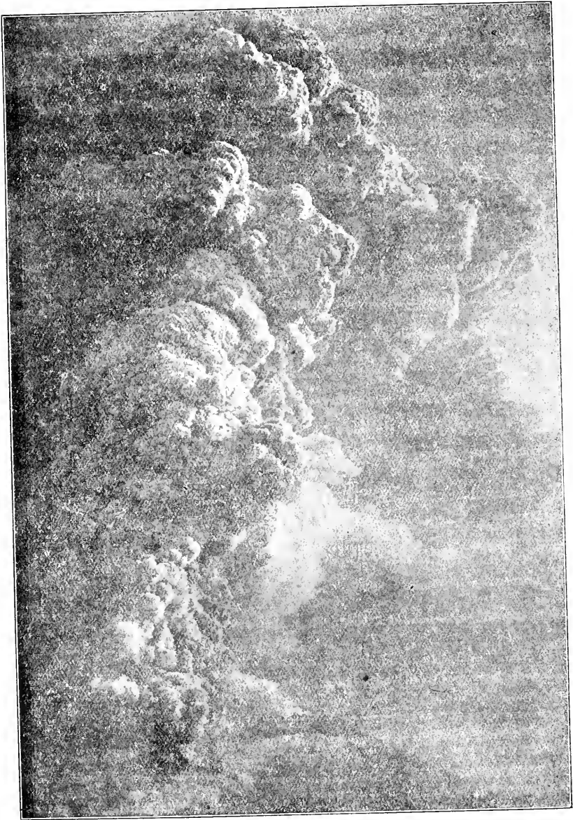
Fig. 15.—Sakura-jima at the first phase of eruption, as seen from Kagoshima. (Photo by Yamashita.)
