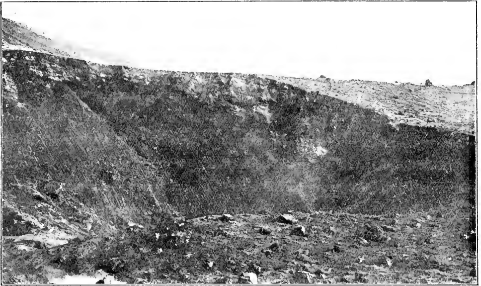
Fig. 27.—Blow-hole above No. 1 venthole in the western lava-field, marked with a cross in Pl. XV. (Photo by Mr. Yamaguchi.)
