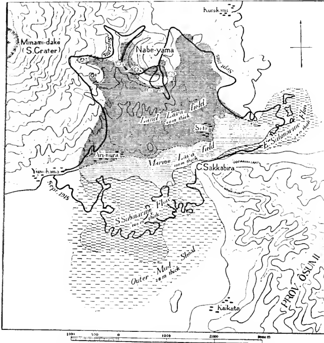
Fig. 24.—Distribution of the Nabé-yama lava-flows, land, marine and submarine. The heavy line, marked 'Sept. 1915,' shows the subterial extent of the lava-field by the recent survey (p. 104, footnote).
