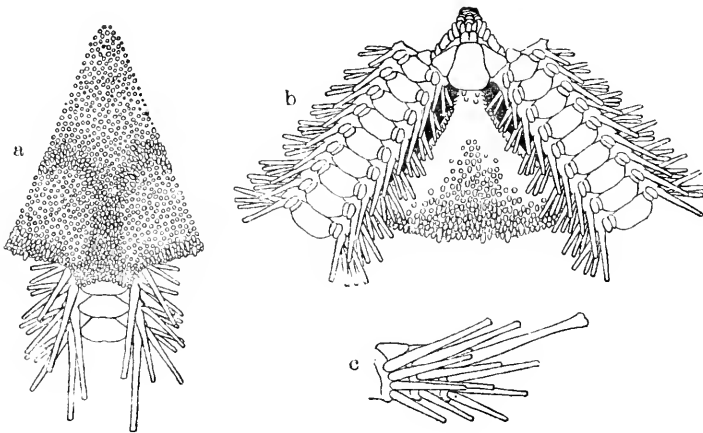
Fig. 97. Ophiomastix mixta . ×3. a . From above. b . From below. c . Side view of three arm joints near disk.
