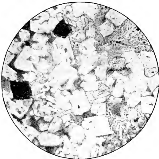
Fig. 36.—Miconoritic segregation in the Ôhira lava of 1749.
