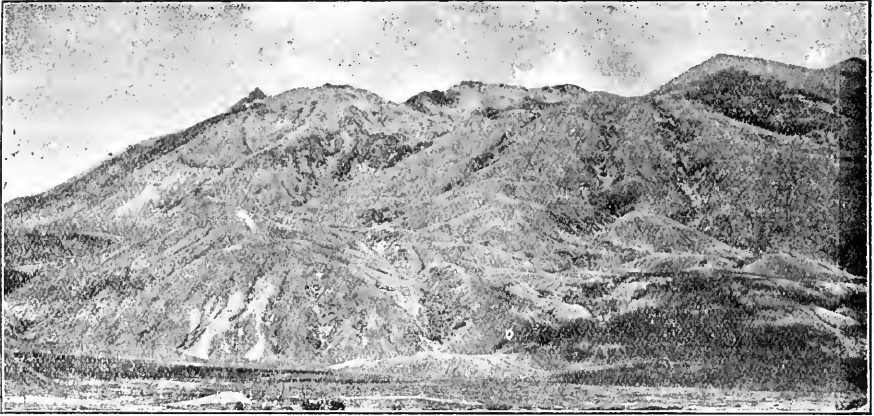
Fig. 9. Eastern view of the three cones.
