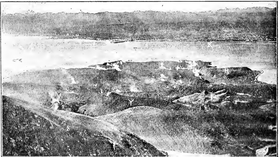
Fig. 31.—The volcanello Furihata on the western slope. (Photo by Mr. Yamaguchi.) yv—Yuno-hira vent. y—Yuno-hira somma. F—Collapsed dome of Furihata. n—Hakama-goshi. k t —Kanzé islet. k—Kagoshima.
