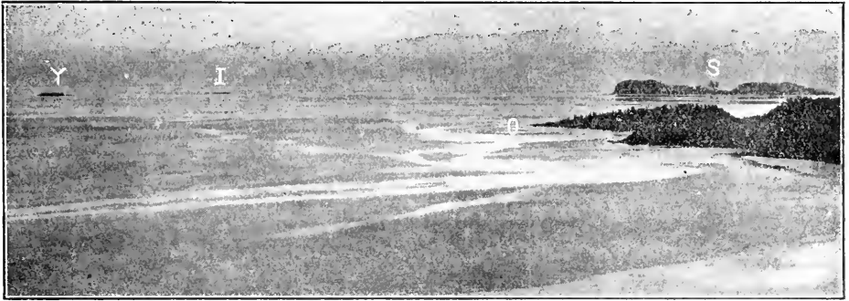
Fig. 13.—Three new islands, Shin-jima, Iwô-jima, and Yôbisu-jima, of 1779-1780. (After Yamaguchi.)
