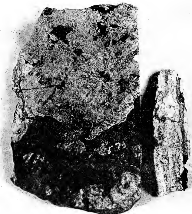
Fig. 42.—Ejecta of diopside-gabbro, a secretory product of angite-andesite. Right-hand figure is the cross section.
