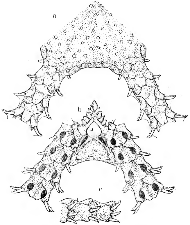
Fig. 1. Ophiostiba hiteki . \times 20 . a. From above. b. From below. c. Side view of three arm joints near disk.
