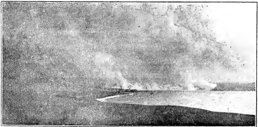
Fig. 23.—Lava end at the Sêto strait on Jan. 18, 1911.
