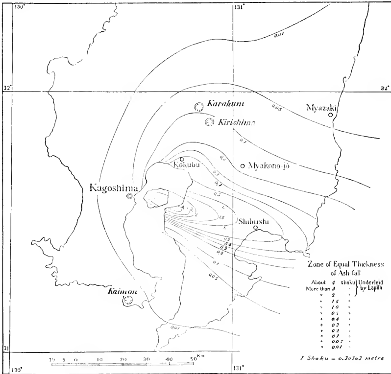
Fig. 26.—Distribution of ejecta in Southern Kyūshū.
