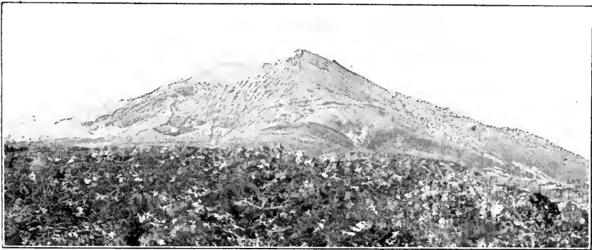
Fig. 37.—North Cone (Kita-daké, K) viewed from Kômen. Cf. Text-fig. 33, p. 158. (Photo by Mr. Yamaguchi.)
