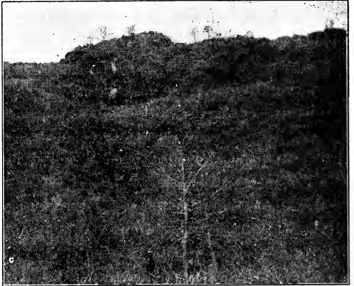
Fig. 38.—The sixth venthole in the northeast lava-field of 1779. See Text-figs. 10c, 11, 33, 37 and Geologic Map.
