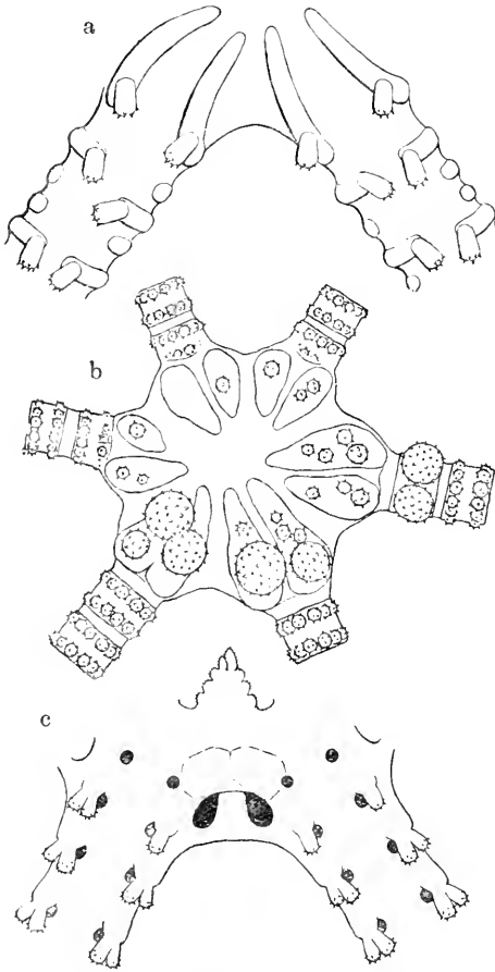
Fig. 7. Astroceras pergamena . a. From above. \times 7 . b. From above. \times 8 . c. From below. \times 14 . b and c. Young.
