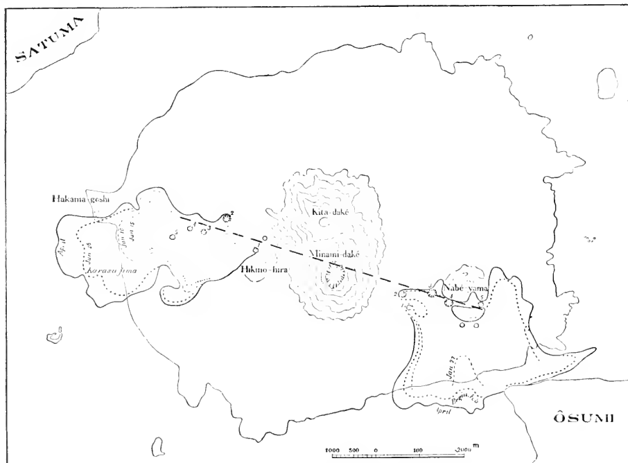
Fig. 19.—Lava-area and positions of bocche. (For Satuma read Satsuna .)
