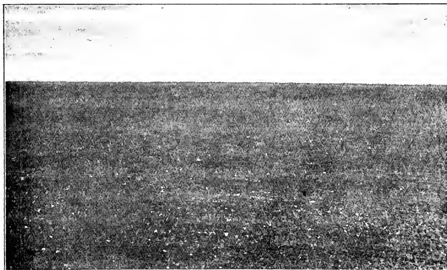
Fig. 21.—Floating pumice desert on the western shore of Sakura-jima.
