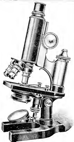
No. 40H TWO EYEPIECES Triple NOSEPIECE 16mm, 4mm and 2mm objectives. Condenser and iris diaphragms Net. $80.00
