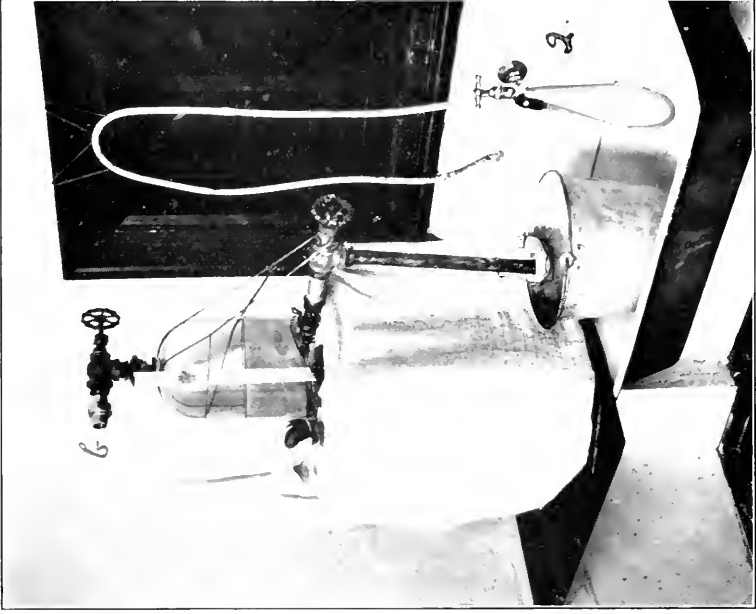
Apparatus for testing the porosity of cloths, etc., for fumigation outfits; 1a Aneroid barometer box; 2b Union coupling in which samples were placed for test (Original).
