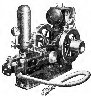
Deming Premier Power Sprayer
