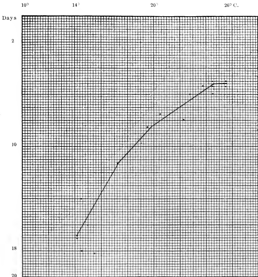
Fig. 19. Relation of temperature to the incubation of eggs of Carpocapsa pomonella in Arkansas, according to Jenne, 1908 (original).
