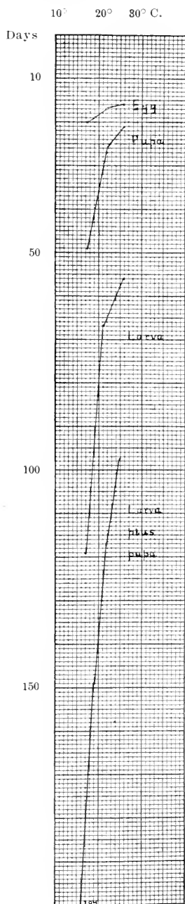
Fig. 13. Relation of temperature to development of Dendrolimus pini , from data quoted by Bachmetjew; egg, pupa and larva from Regener, 1865; larva plus pupa from Ratzeburg, 1839 (original.)
