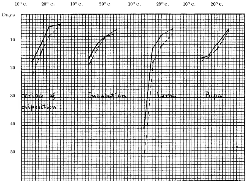
Fig. 14. Relation of temperature to different stages of Tomiscus typographus Linn; solid line represents 55 per cent and dash line 96 per cent moisture; as given by Hennings (1907), original.
