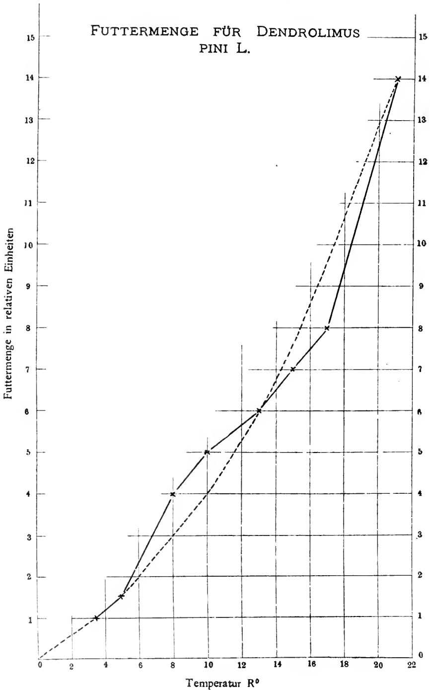
Fig. 16. Relation of temperature to the amount of food eaten by larva of Dendrolimus pini , according to Regener (21), from Bachmetjew.
