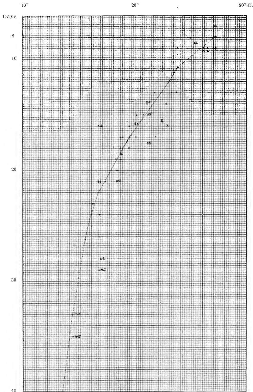
Fig. 20. Relation of temperature to the time of the pupal stage of Carposcypsa pomonella :— . . . according to Jenne, Arkansas, 1908; c—according to Gillette, Colorado, 1901; MJ—according to Melander and Jenne, Washington, 1904; XS—from author's data, New Hampshire, 1906-08 (original).
