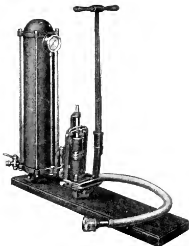
"Samson" Double Acting Sprayer
