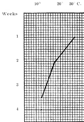
Fig. 12. Relation of temperature to life cycle of Culex pipiens according to data of Kerschbauer (original).
