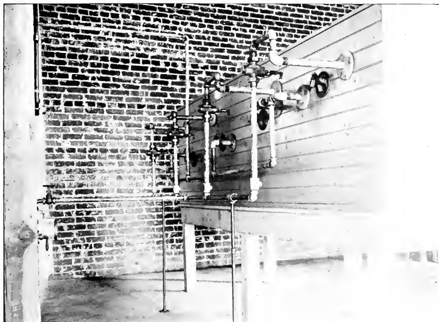
Back side of cool chambers showing brine piping and balanced valves before insulation was applied
