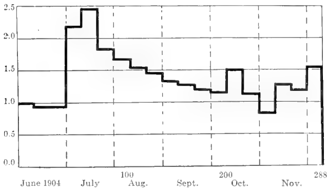
Fig. 2 Graph of the life history of Gastrostyla steinii showing the average daily rate of division of the four lines of animals which compose the culture, again averaged for ten day periods. Hay infusion culture medium. To illustrate a case where the rhythms are apparently absent for a considerable period. Compare with fig. 3. (Woodruff, '05)
