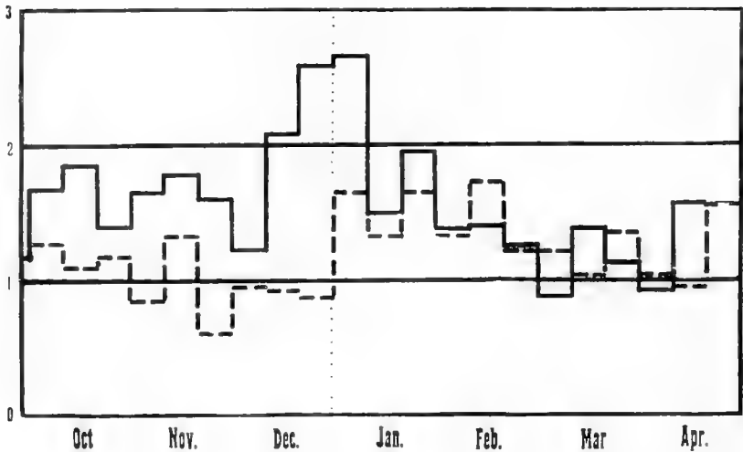
Fig. 1 Graph showing the rate of division of Paramaecium aurelia , Culture I and Culture IB, from October 1, 1910, through April 29, 1911. The ordinates represent the average daily rate of division of the four lines of the respective cultures, again averaged for ten day periods. Culture I = ———; Culture IB = - - - - -
