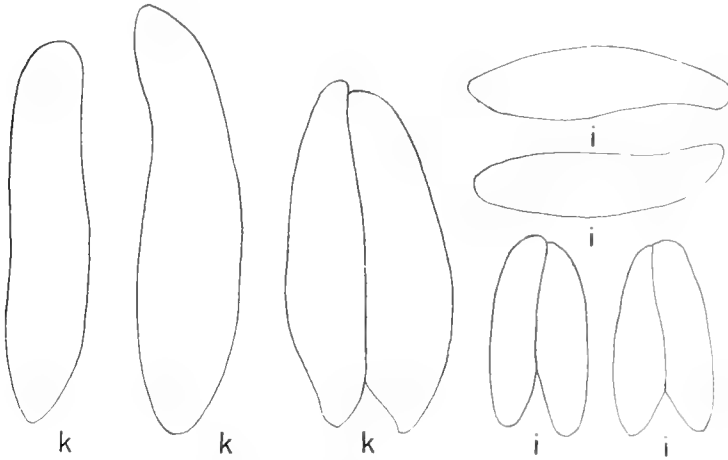
Fig. 13 Conjugants and non-conjugants from a culture composed of a mixture of the two aurelia races k and i , showing that each pair is composed of individuals of but one race,—either of k or i . \times 333 .
