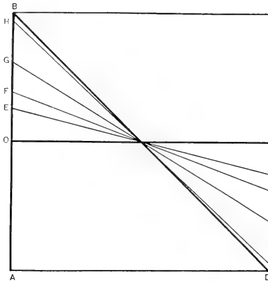
Fig 12 Diagram showing the average correlation in length between the members of pairs in wild cultures of one and of two species, and in pure races. O-O , mean; also line of no correlation; B-D , line of complete positive correlation. E , average correlation (0.250) for the twelve pure races of tables 2 and 3. F , average correlation (0.380) for the eight wild cultures of the present paper (tables 1 and 3). G , average correlation (0.614) in the five wild cultures studied by Pearl ('07). H , average correlation (0.940) for the two lots of table 3 where two species were present, both conjugating.
