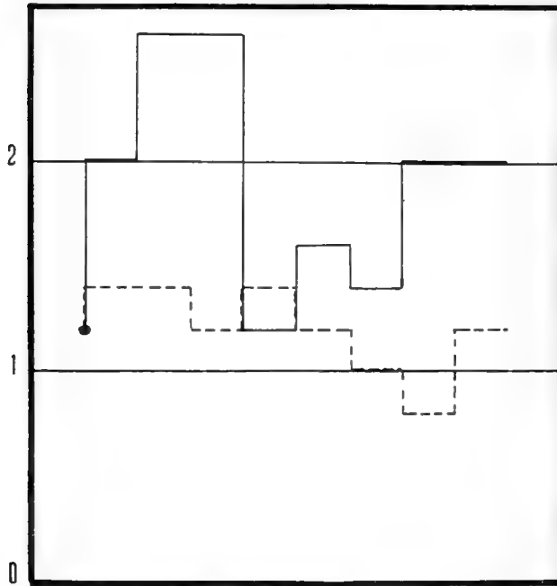
Fig. 11 Graph of the average daily rate of division for five day periods of line 1 (of the four lines of 'sister' cells) of series IBS2b (= continuous line) and of line 1 (of the four lines of 'sister' cells) of series IB76b (= - - - - line). To illustrate the same points as fig. 10. Compare with fig. 8, section B, and fig. 9, section B.
