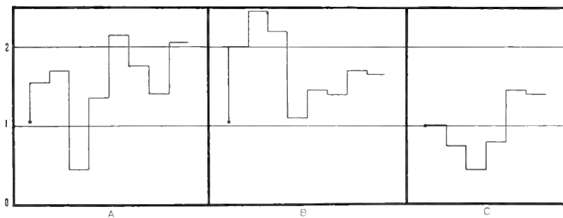
Fig. 8 A, Graph of the average daily rate of division at 82°F. of the four lines of 'sister' cells of Paramaecium aurelia , series IBS2a, again averaged for five day periods. B and C., Similar graphs for series IBS2b and IBS2c respectively. To illustrate the fact that rhythms in the rate of division appear more pronounced under practically constant environmental conditions. Compare with the last ten periods of the culture subjected to room temperature changes (fig. 4).
