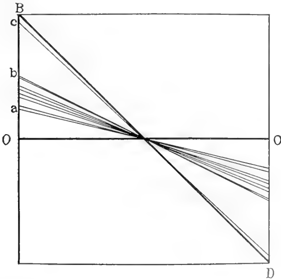
Fig. 7 Diagram illustrating the extent of correlation in the eight 'wild' cultures of tables 1 and 3 (at a to b ), and in the mixture of two species in lot 27 (at c ). Beginning at a the lines show in order the coefficients of correlation for lots 23, 2, 7, 22, 1, 5, 4, 3, (at b ); then that for the mixture of two species at c .
