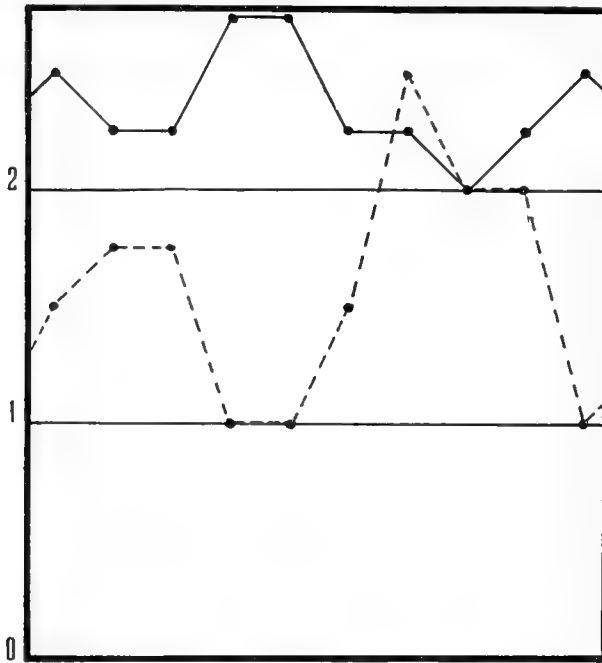
Fig. 13 Graph of the average daily rate of division of the four lines of 'sister cells of series IB82b (= continuous line) and of IB76b (= - - - line) for the ten days during which temperature variations were practically absent. To illustrate the same points as fig. 12. Compare with the section of fig. 12 included within the vertical dotted lines.
