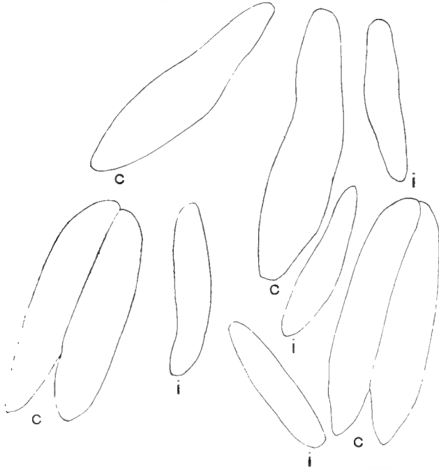
Fig. 1 Typical group of specimens from a culture consisting of a mixture of the large race C_2 and the small race i (both aurelia). Conjugating pairs all C_2 . \times 333 .
