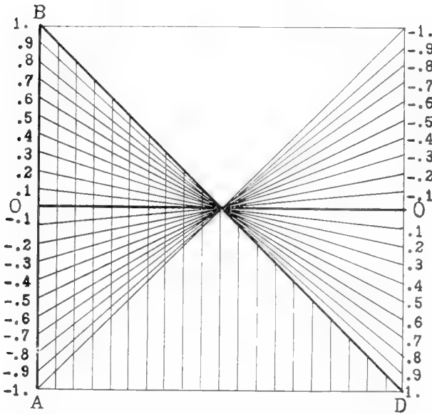
Fig. 6 Diagram illustrating the significance of different coefficients of correlation (should be compared with fig. 5, to the upper portion of which it corresponds). The vertical lines are the terminal portions of the lines representing the lengths of various classes of individuals, arranged according to their size, the largest ( A-B ) at the left. The terminations of these diverse lengths trace the oblique line B-D . O-O marks the position of the mean length of all. The lines B-D and O-O and the other oblique lines show the positions of the theoretical average dimensions for the mates of individuals of the given sizes, in case of different coefficients of correlation. If the dimensions of the mates fall in the same line B-D as those of the principals, the correlation is 1.000; if they fall at the mean O-O the correlation is 0; if they fall at right angles to B-D , the correlation is -1.00 . If they fall in a line dividing O-B into equal parts, the correlation is 0.500. The coefficients, from -1. to +1. , by tenths, are illustrated in the diagram, the numbers at the extremity of a given line showing the coefficient to which it corresponds.
