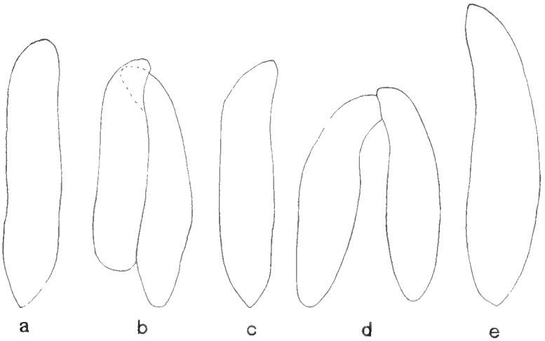
Fig. 2 Conjugants ( b and d ) and non-conjugants ( a , c and e ) from the race k , showing the relative sizes. \times 333 .
