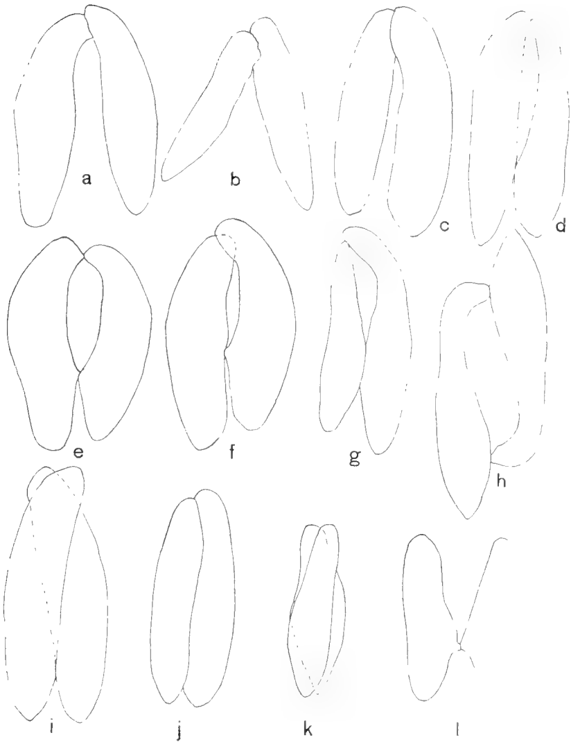
Fig. 3 Characteristic attitudes in conjugation. All are drawn with the projection apparatus from fixed specimens, save h , which is a free-hand sketch from a living pair. a, e, f belong to the race k ; c, d, g, i, j to the race C 2 ; b, k and l to the race c (all aurelia); a, b , and c , stages with only the anterior tips in contact; e, f, g , anterior tips and mouths in contact; h , reversed pair, at beginning of conjugation; i, j , most complete union; k , view of pair in profile, showing the crossing (also seen in i ); l , last stage, just before complete separation. Magnification (for all but h ), 333 diameters.
