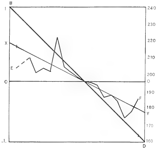
Fig. 8 Diagram illustrating correlation in lot 3 ('wild' culture). B-D , lengths of the classes of individuals in order of size. E-F , lengths of the mates for these classes. X-Y , regression line showing the general trend of the broken line E-F , and indicating by the proportion of the line O-B which it cuts off, the value of the coefficient of correlation (0.507). O-O , mean length for the entire lot. The numbers at the right show lengths in microns.
