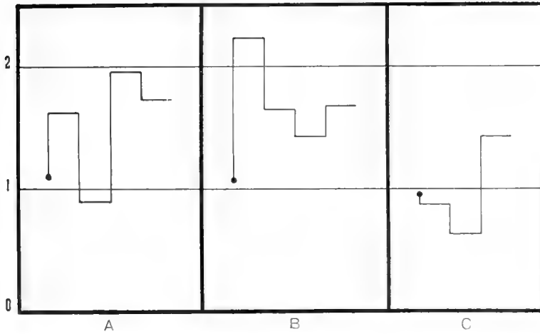
Fig. 6 A , Graph of the average daily rate of division at 82°F. of the four lines of 'sister' cells of Paramaecium aurelia , series IBS2a, again average for ten day periods. B and C , Similar graphs for series IBS2b and IBS2c respectively. To illustrate rhythms in the fission rate when the cultures are subjected to practically constant conditions, including temperature.
