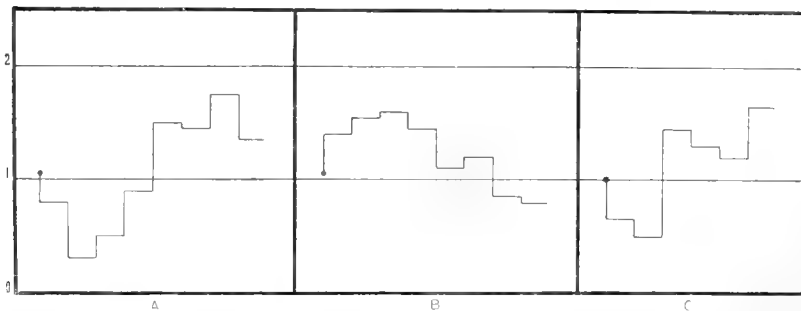
Fig. 9 A, Graph of the average daily rate of division at 76°F. of the four lines of 'sister' cells of Paramaecium aurelia , series IB76a, again averaged for five day periods. B and C., Similar graphs for series IB76b and IB76c respectively. To illustrate the same point as fig. 8.
