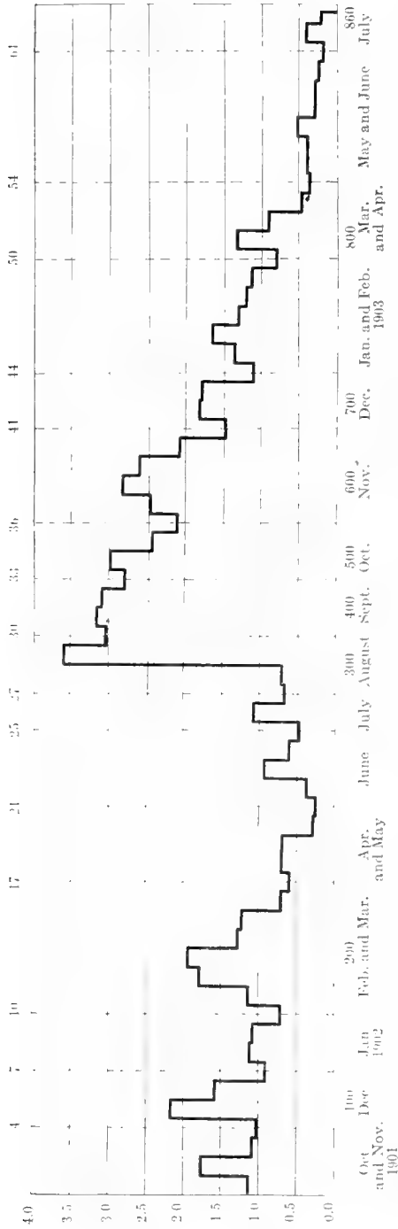
Fig. 1 Graph of the life history of Oxytricha fallax , culture A, showing the average daily rate of division of the four lines of animals, again averaged for ten day periods. 'Rejuvenated' at end of first cycle by artificial stimulation. To illustrate 'cycles' and 'rhythms' in the fission rate of infusoria under pedigree culture methods. The limits of the various rhythms are designated by vertical broken lines. (Woodruff, '05)
