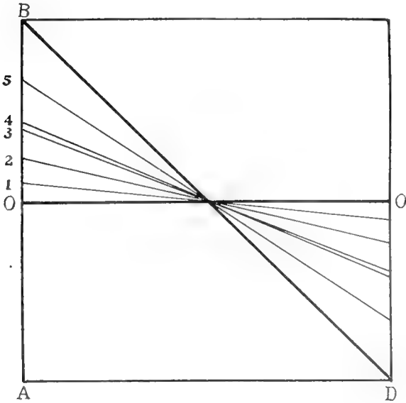
Fig. 14 Diagram showing the different degrees of correlation between members of pairs in lot 1 (table 11), according as we examine the mating of individuals of medium sizes or of those of extreme sizes. O-O , mean and line of no correlation; B-D , line of complete positive correlation. 1, Correlation (0.104) for pairs consisting exclusively of individuals of 'medium' size. 2, Correlation (0.229) when we take all specimens of medium size as principals, and compare them with their mates. 3, Correlation (0.398) when all specimens, of all sizes, are included. 4, Correlation (0.439) when we take all specimens of 'extreme' size as principals and compare them with their mates, of whatever size. 5, Correlation (0.678) for pairs consisting exclusively of individuals of extreme sizes. (For the sizes considered 'medium' and 'extreme' see table 11).
