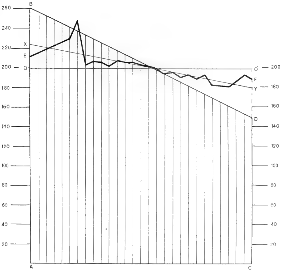
Fig. 5 Diagram to illustrate correlation in size between the members of pairs in lot 1 (see explanation in the text and compare fig. 4). The vertical lines represent the lengths of individuals of the different classes arranged in order from longest (260 microns) to shortest (148 microns), their terminations tracing the oblique line B-D . The distance from A-C to O-O' shows the average length for all. The distance from A-C to the broken line E-F shows the lengths of the mates of the classes of individuals represented by the vertical lines. The general trend of this line E-F is shown by the line X-Y ('regression line'). The value of the coefficient of correlation is given by the proportion which the line O-X is of the line O-B .
