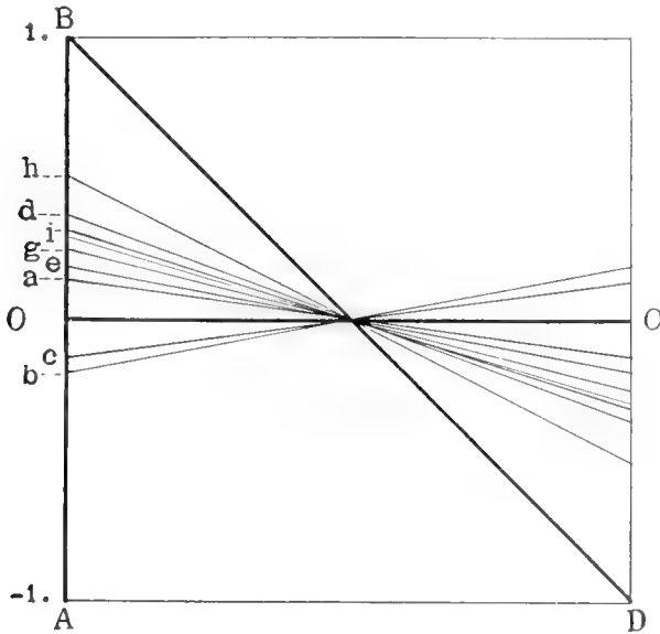
Fig. 9 Diagram illustrating the correlation in the eleven lots composed of pure races, of table 2. O-O , mean and line of no correlation; B-D , line of complete positive correlation. a , lot 9; b , lot 10; c , lot 11; d , lot 12; e , lot 13; g , lots 15 and 18; h , lot 16; i , lots 17 and 19. Just beneath i is the line for lot 14.
