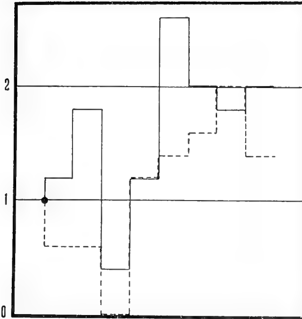
Fig. 10 Graph of the average daily rate of division for five day periods of line 1 (of the four lines of 'sister' cells) of series IB82a (= continuous line) and of line 1 (of the four lines of 'sister' cells) of series IB76a (= - - - - line). To illustrate the fact that rhythms of practically the same amplitude and character appear in a graph of a single line of cells as appear when four such lines are averaged together. Compare with fig. 8, section A, and fig. 9, section A.
