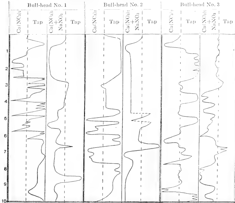
Fig. 2 Showing the reaction of bull-heads ( Ameiurus melas ) to \text{Ca}(\text{NO}_3)_2 , alone, and in combination with a trace of \text{NaNO}_3 . The concentration of the calcium salt was 0.01 N throughout and that of the sodium salt 0.0002 N; experiments performed in distilled water; numbers at left indicate time in minutes.
